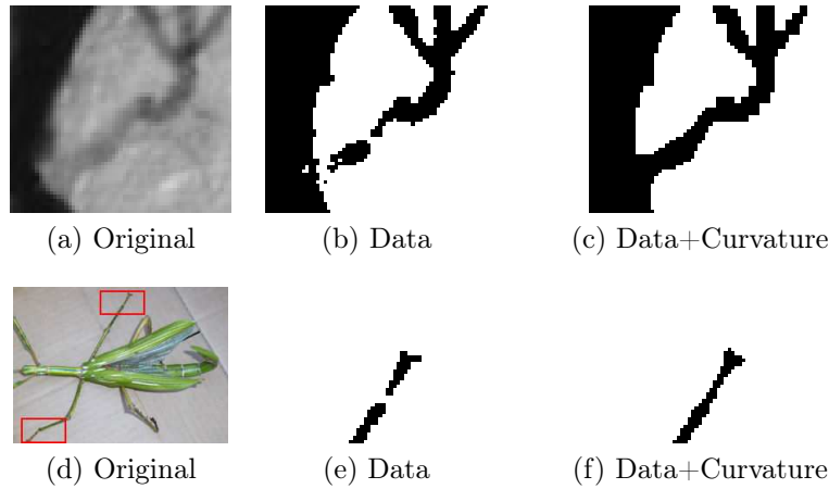
Figure 3.12: Results for the grid graph model [EG10]. The original image is displayed in the left; segmentation using only data in the middle; and the segmentation using squared curvature regularization in the right. Connectivity is encouraged, but to a very limited extension.
