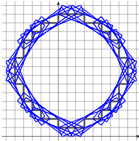
Figure 4.5: Tangential cover. The tangential cover is the collection of all maximal DSS in the digital contour of some digital shape. (Extracted from [Lac13])
