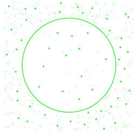
(b) Result of level-set method for \lambda = 1
