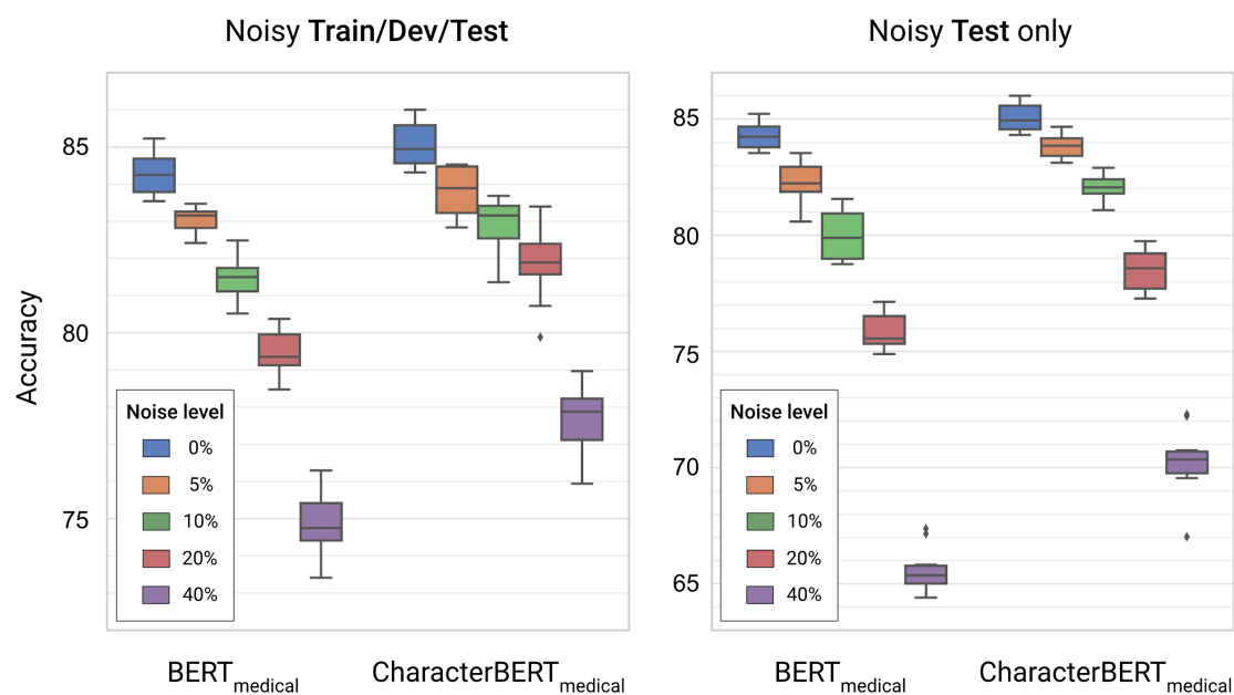
Figure 5.11: Comparing BERT and CHARACTERBERT on noisy (misspelled) versions of MEDNLI test.
