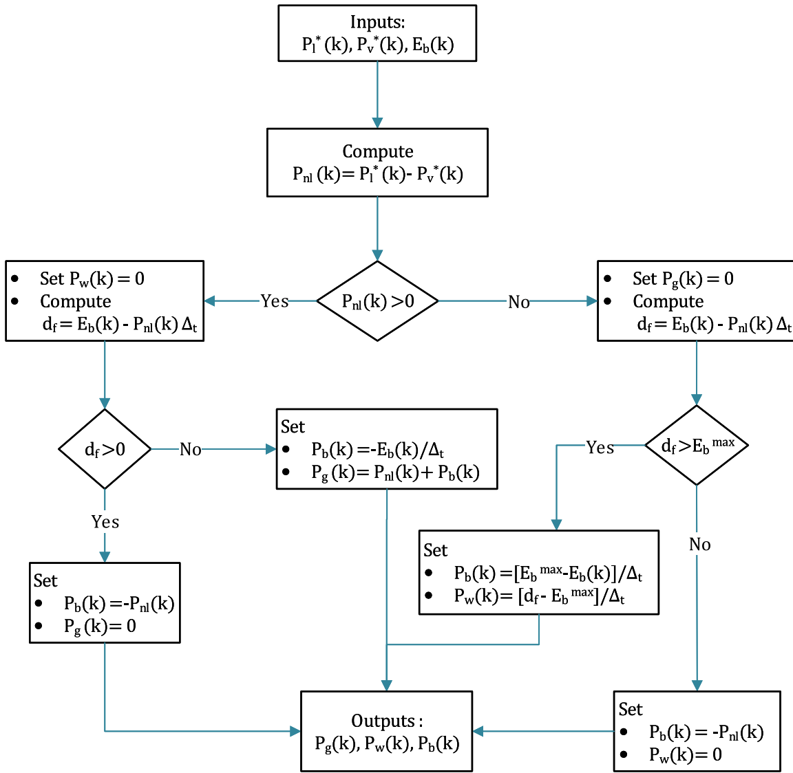
Figure 3.9 – Flowchart algorithm of a Rule-based controller for HEMS.
