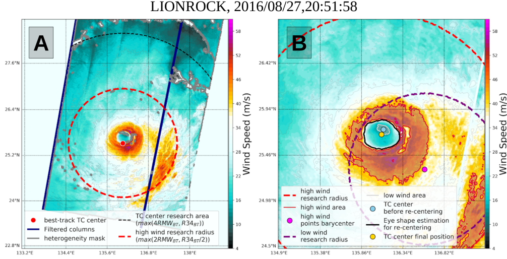
Figure 3.2 – Illustration of the TC center research algorithm on the case of TC LIONROCK (Western Pacific) observed with Sentinel-1 SAR on the 27th of August 2016 . The TC wind field ( \text{m.s}^{-1} ) as retrieved from the SAR is shaded in (A) and (B); (B) is a zoom over the TC eye. In (A) the heterogeneity mask (masking high gradient values of the backscatter signal) is represented with grey contours, the black dashed circle denotes the radius at which the heterogeneity mask is removed, the subswath signatures are identified with dark blue lines, and the red dot locates the interpolated BT TC center. The red dashed circle in (A) and (B) denotes the first research area for TC center. In (B) the detected high wind points are contoured in red, their centroid is located with the magenta dot, the second research circle is featured by the purple dashed line, the low wind points are contoured in light grey, and their centroid is located with the cyan dot. The raw eye shape signal is depicted by the black contour, and the final TC center is located with the yellow dot.
