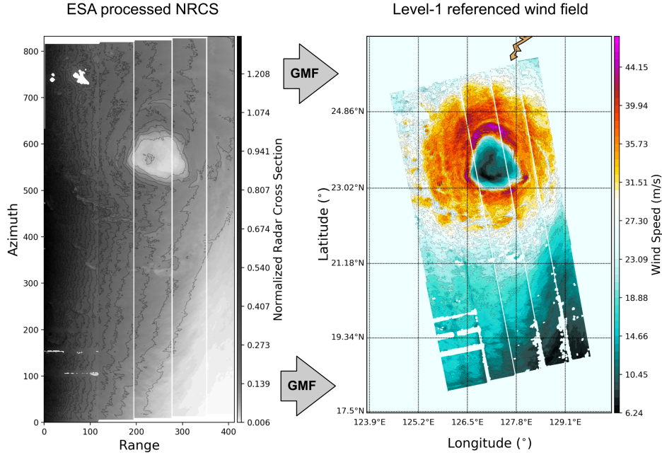
Figure 2.3 – (A) Level-1 NRCS from SAR acquisition on TC TRAMI (2019/08/28,09:35); (B) Surface wind field retrieved after application of CMOD5n-MS1A-HW GMF
