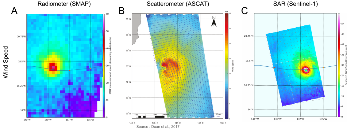
Figure 1.10 – Examples of satellite radiometer, scatterometer and SAR wind speed retrievals. (A) SMAP radiometer acquisition on TC LESTER (2016); (B) ASCAT scatterometer acquisition on TC LIONROCK (2016) with retrieved directions indicated by black arrows; (C) Sentinel-1 SAR acquisition on TC LESTER (2016).
