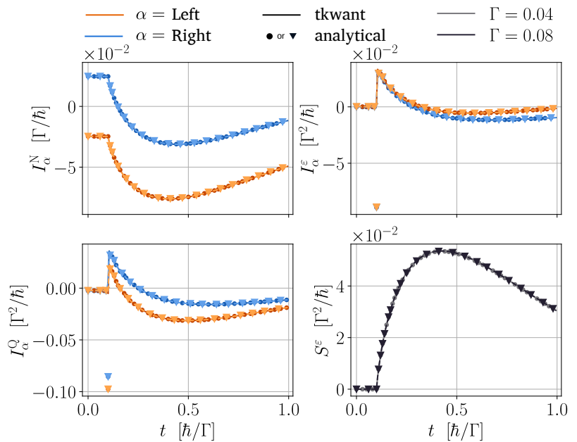
Figure 6.9 – Transport quantities as calculated from analytical formulas (symbols) and by tkwant (lines), for two values of \Gamma ( \Gamma = 0.04 (circles and light colors) and \Gamma = 0.08 (triangles and dark colors)). The set of data for both values of \Gamma are perfectly superimposed. The discrepancy points between analytics and numerics for the energy and heat currents, at the time of jump t = t_0 , is a signature of a singularity appearing in the WBL [37]. For \Gamma = 0.04 and \Gamma = 0.08 , the other values being fixed to \bar{t}_0 = 0.1, \bar{\Delta t} = 3.9, \bar{V}_0 = 0.5, \bar{\Delta V} = 0.5, \bar{\mu}_L = -0.1, \bar{\mu}_R = 0.1, \bar{T}_L = 0.11, \bar{T}_R = 0.09, wb = 500
