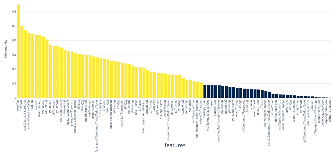
Figure 5.7: Features informativity for dataset of individual accounts, where features that have a correlation with the label \geq 0.1 are highlighted with yellow.
