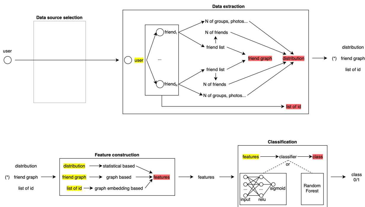
Figure 4.16: Technique for individual bot detection. Inputs of modules are highlighted with yellow, and outputs with red.
