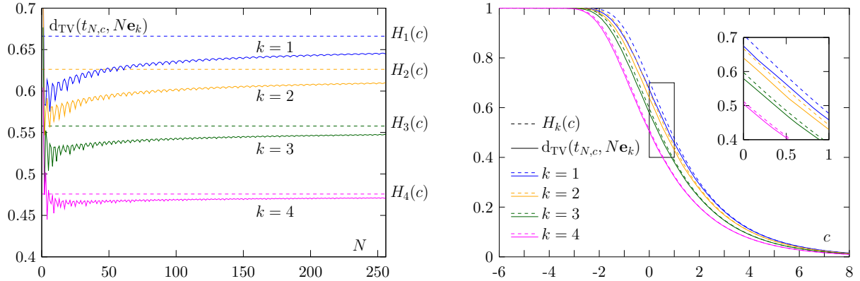
Figure 9: For parameters K = 4 , k \in [K] , \mu = (0.7, 0.8, 1.0, 1.3) , p = 0 : left panel shows d_{\text{TV}}(t_{N,c}, N \mathbf{e}_k) as a function of N , 2 \leq N \leq 256 for c = 0.17 and right panel shows H_k(c) and d_{\text{TV}}(t_{N,c}, N \mathbf{e}_k) as functions of c , with -6 \leq c \leq 8 , for N = 100 .
