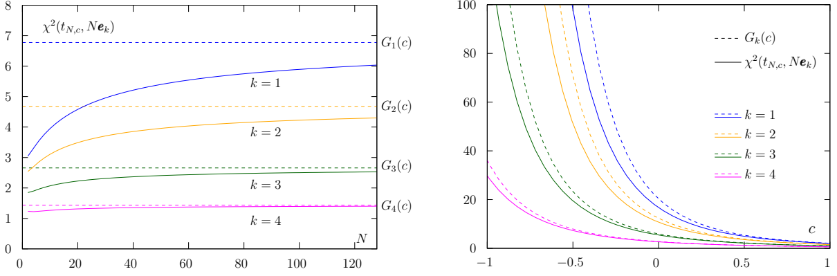
Figure 8: For parameters K = 4 , k \in [K] , \mu = (0.7, 0.8, 1.0, 1.3) , p = 1.7 : left panel shows \chi^2(t_{N,c}, N \mathbf{e}_k) as a function of N , 2 \leq N \leq 128 for c = 0.4 , and right panel shows G_k(c) and \chi^2(t_{N,c}, N \mathbf{e}_k) as functions of c , with -1 \leq c \leq 1 , for N = 150 .
