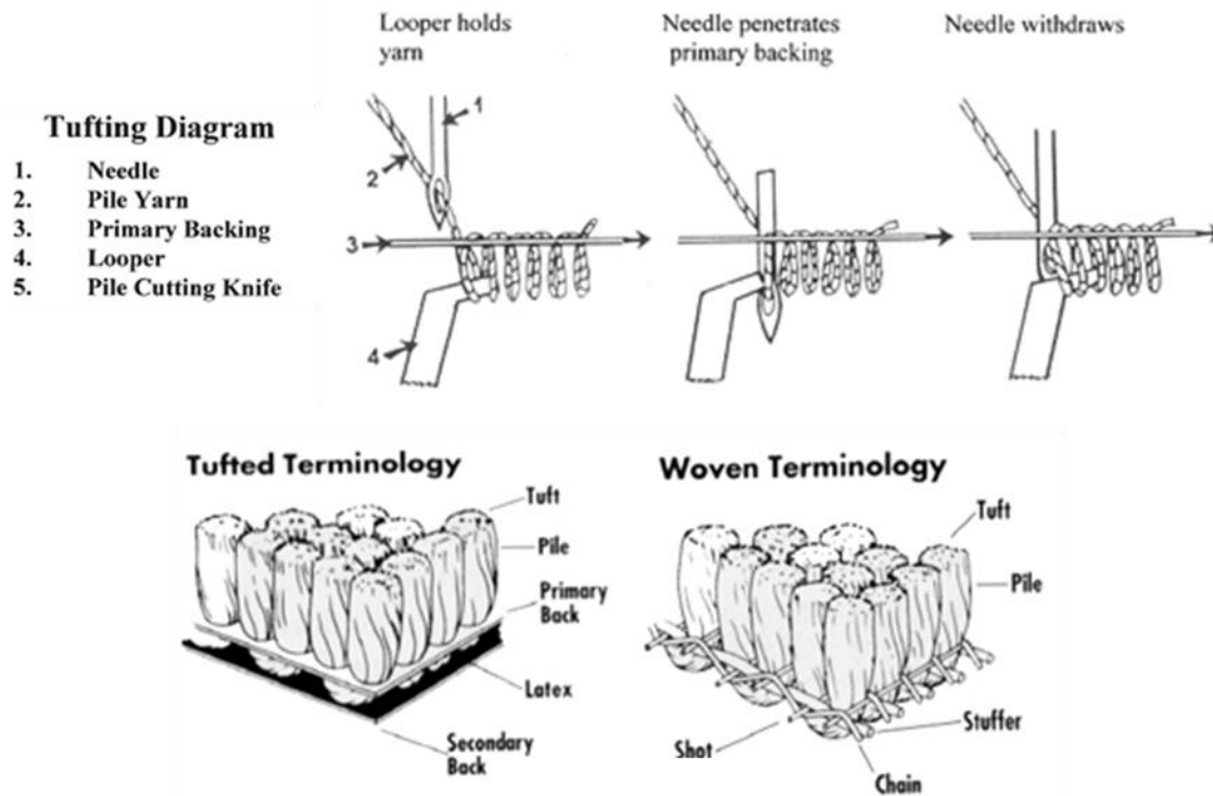
Figure 2: Tufting process.
