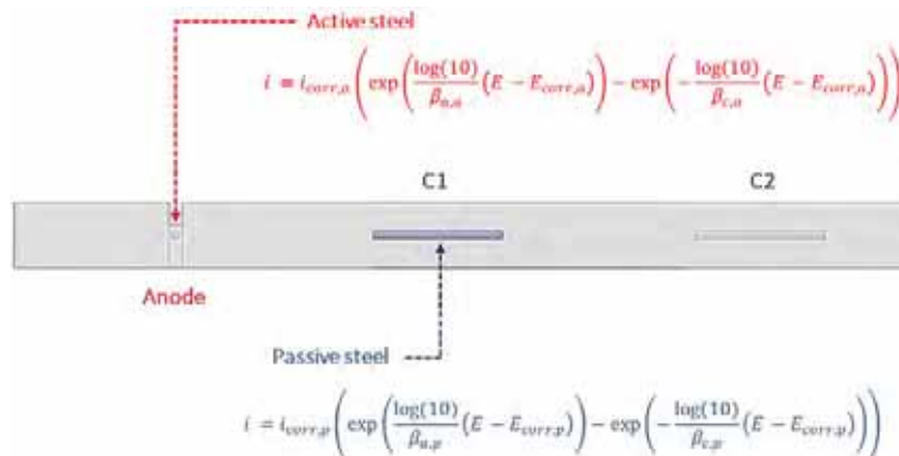
Fig. 9. Boundary conditions of the reinforcement bars of the beam for the anode–cathode C 1 connection system (side view of the first end of the simulated beam).
