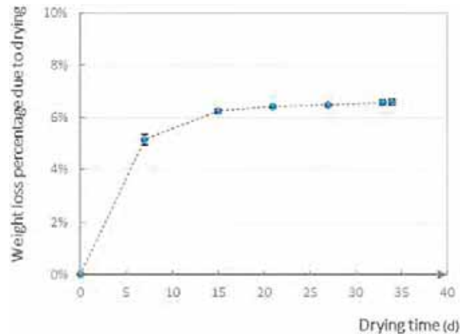
Fig. 4. Stabilization of the weight loss of anodes during their drying in the oven.
