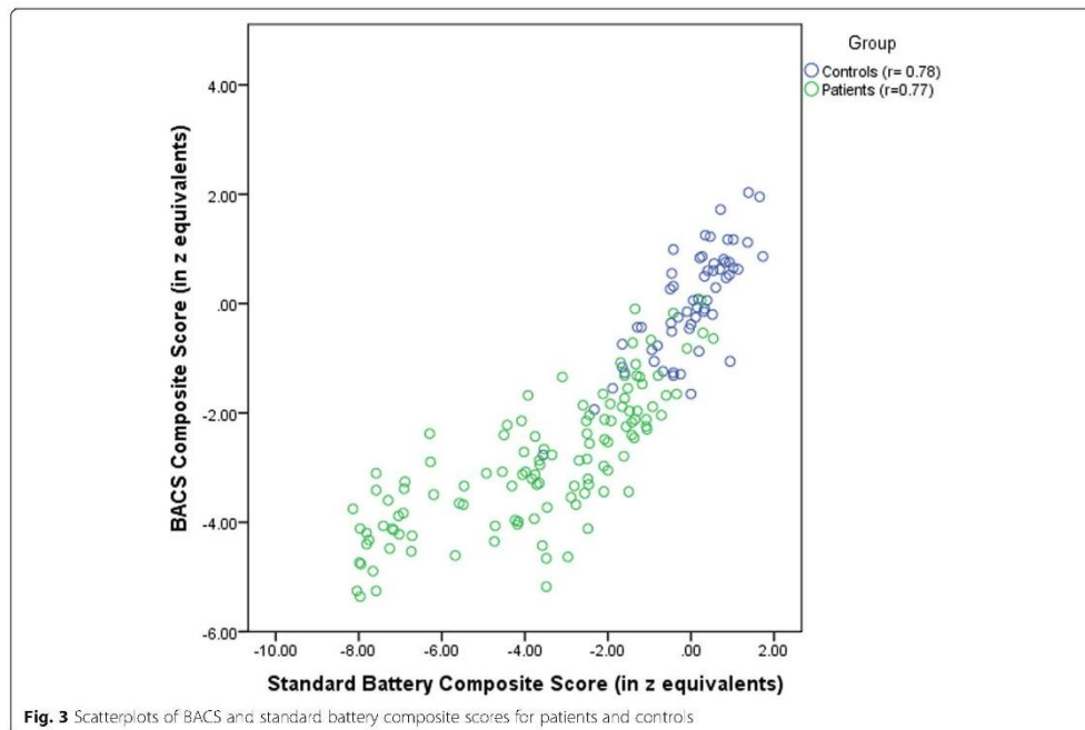
Fig. 3 Scatterplots of BACS and standard battery composite scores for patients and controls
