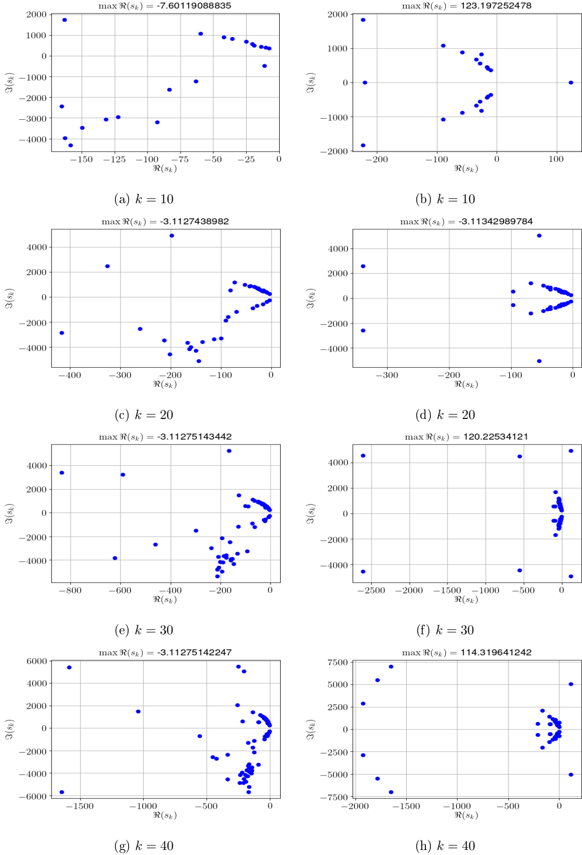
Figure 3.11: The poles of reduced order models in (\mathbf{u}_s, \phi) using the reduced basis of iteration k of Classical Greedy Algorithm 1. Left: case of Petrov-Galerkin projection of Lemma 3.2.2. Right: case of Galerkin projection.
