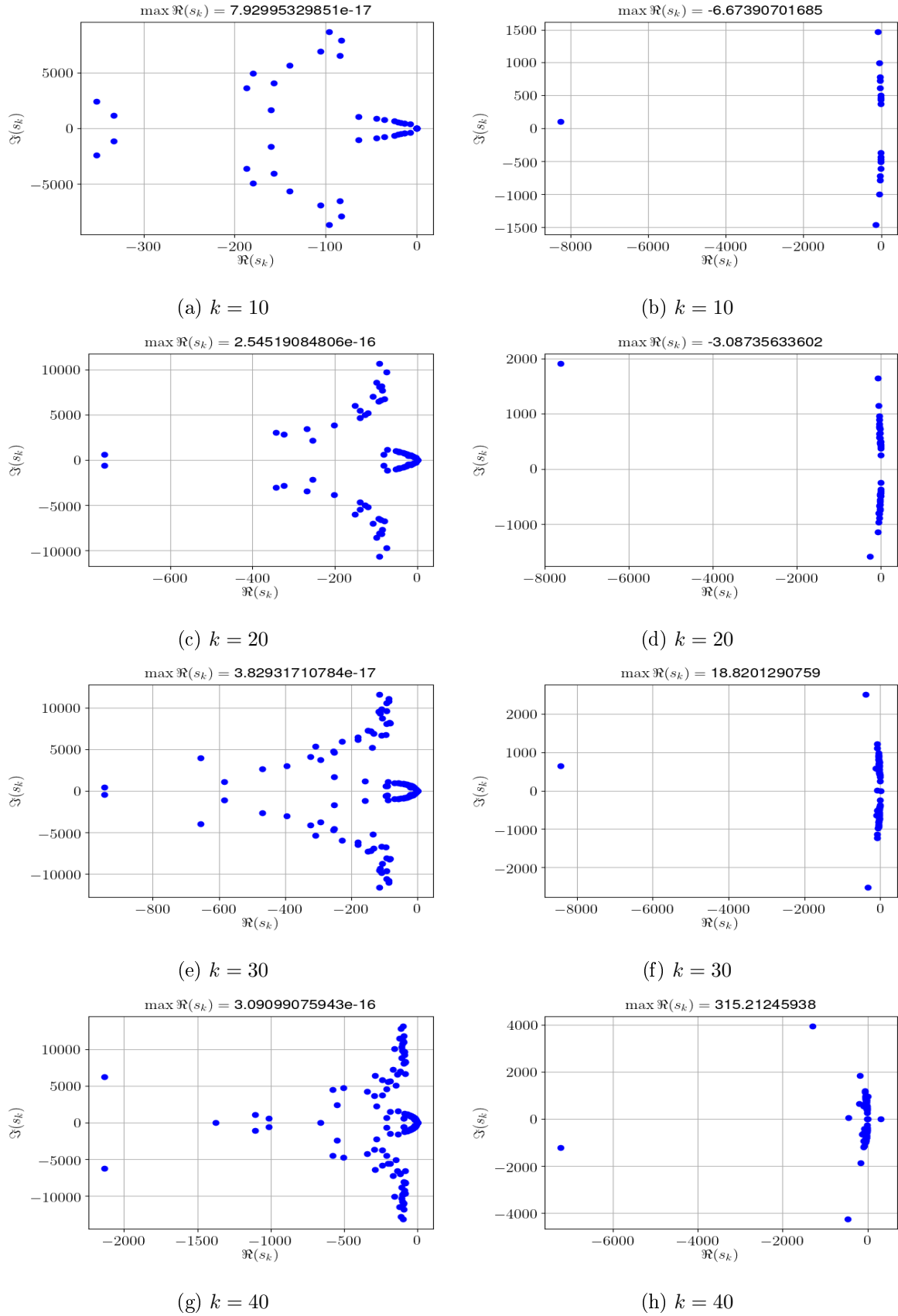
Figure 3.13: The poles of Galerkin reduced order models in (\mathbf{u}_s, p, \varphi) using the reduced basis of iteration k of Greedy Algorithms. Left: case of Classical Greedy Algorithm 1 . Right: case of modified Greedy Algorithm 3 .
