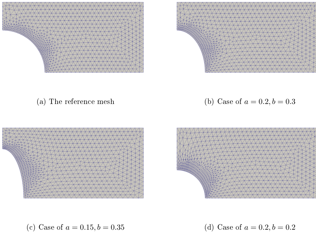
Figure 5.12: The reference mesh (top left) and the deformed mesh in the first example
