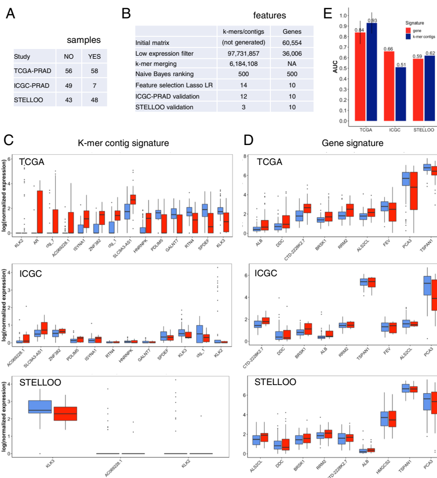
Fig. 5 Relapse signatures generation and analysis. a Characteristics of prostate tumor RNA-seq datasets. b Result of filtering procedure on the k-mer and gene matrices for relapse analysis. Expression of relapse signature elements in LR and HR samples in the TCGA-PRAD, ICGC-PRAD and STELLOO cohorts c k-mer contig signature; d Gene signature. e Signature performances for relapse prediction in the TCGA-PRAD, ICGC-PRAD and STELLOO cohorts
