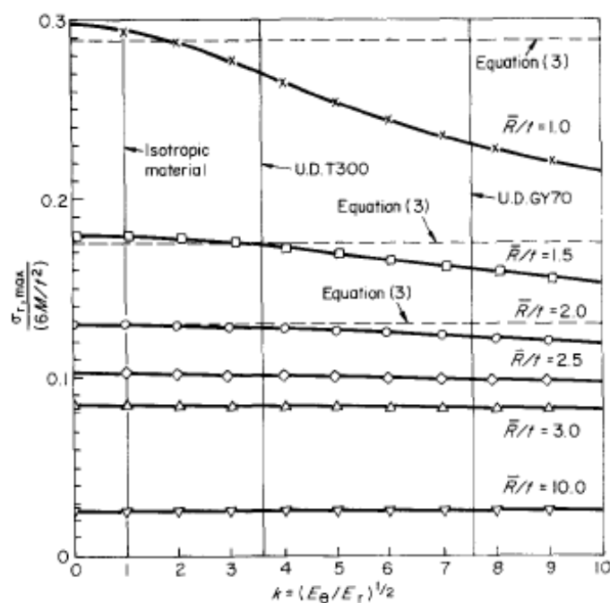
Fig. 5.2. Normalized radial stress as a function of the anisotropy. Kedward et al. 's approximated and Lekhnitskii 's solutions are represented by dashed and solid lines, respectively. For \frac{R_m}{t} \geq 2.5 and \frac{E_\theta}{E_T} \leq 6.0 , the maximum error resulting from the approximated solution is \leq 2.0\% . [ Kedward et al. , 1989]
