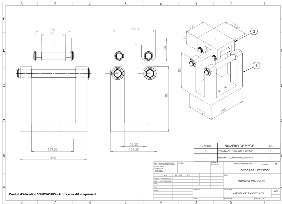
Fig. B.1. Design drawing of 4PB test setup.
