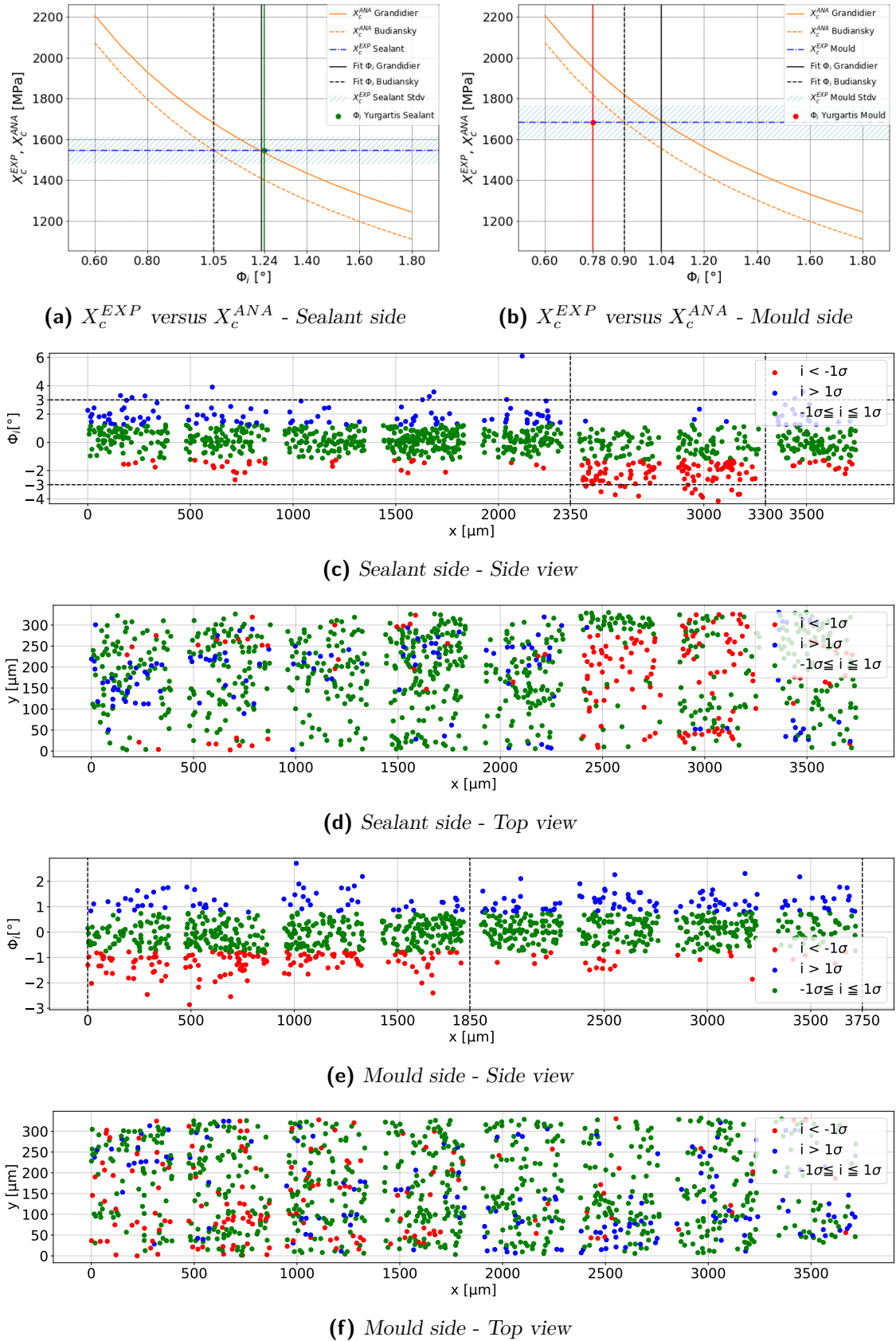
Fig. 4.5. Series 3 - SE84 LV/IM2C - In-plane fibre misalignment \Phi_i .
