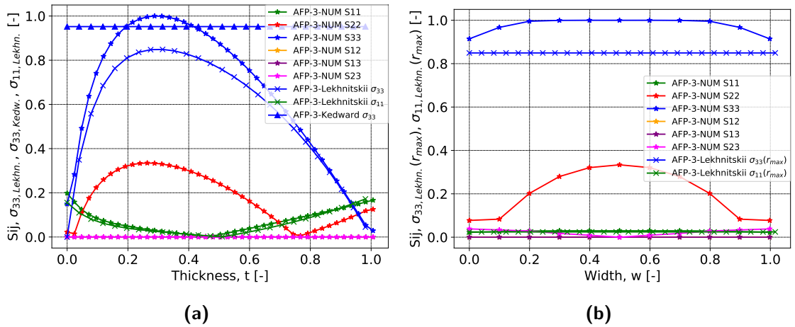
Fig. B.5. Normalized calculated stresses and strains S_{ij} , and analytically estimated radial and circumferential stresses \sigma_{33, Lekhn.} , \sigma_{11, Lekhn.} (Lekhnitskii) and \sigma_{33, Kedw.} (Kedward et al.) as a function of the normalized (a) thickness and (b) width of specimen AFP-03.
