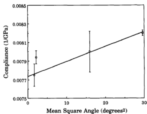
Fig. 2.7. Compliance of laminates (estimated from zero strain) as a function of the mean square fibre misalignment angle for unwrinkled preregs. The deviation is small. [Mrse & Piggott, 1993]
