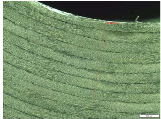
(c) AFP-02, microstructure of the L-beam's arm. (d) AFP-02, microstructure of curved segment.
