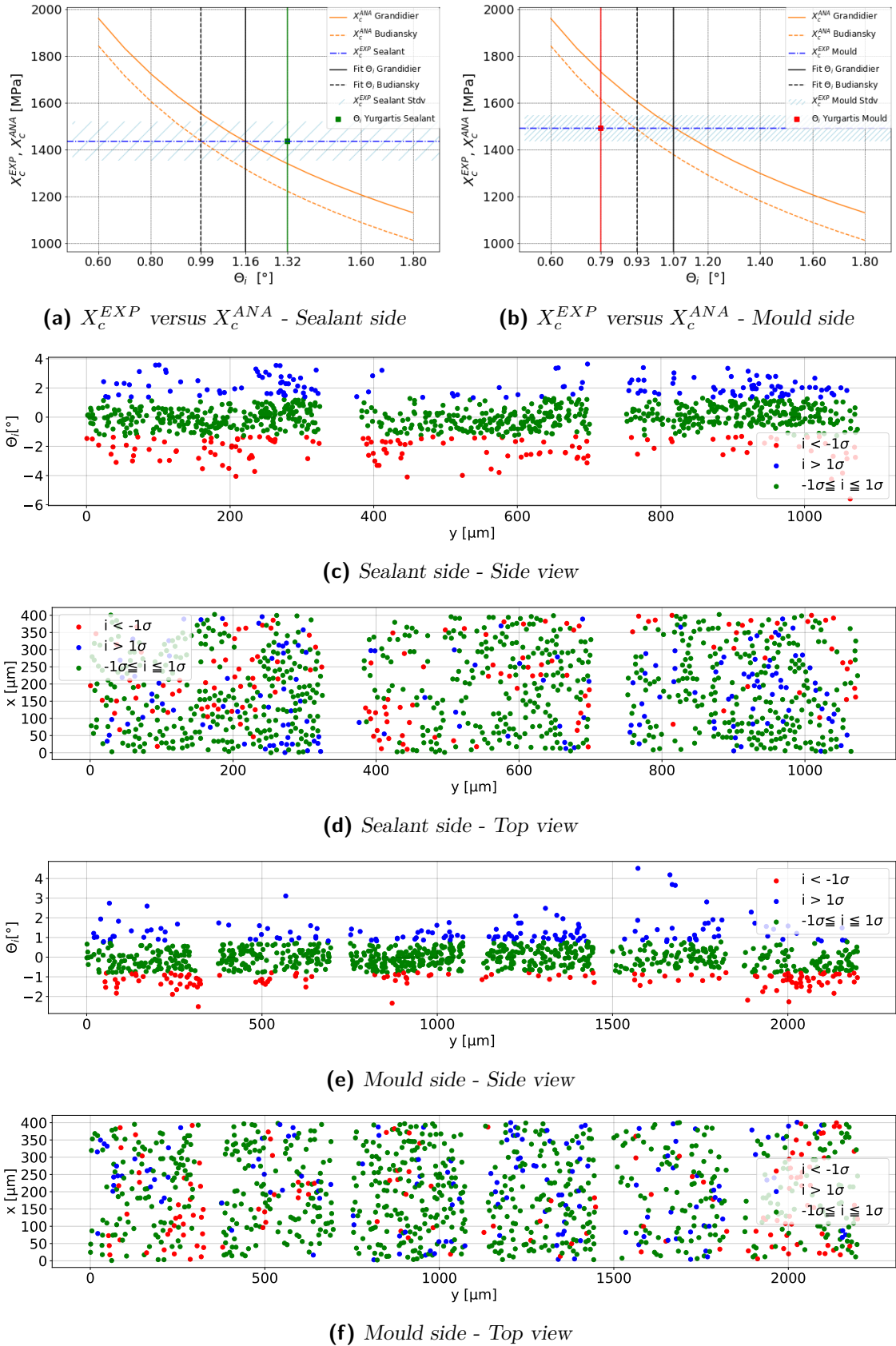
Fig. 4.10. Series 6 - MTC9810/T800S - Out-of-plane fibre misalignment \Theta_i .
