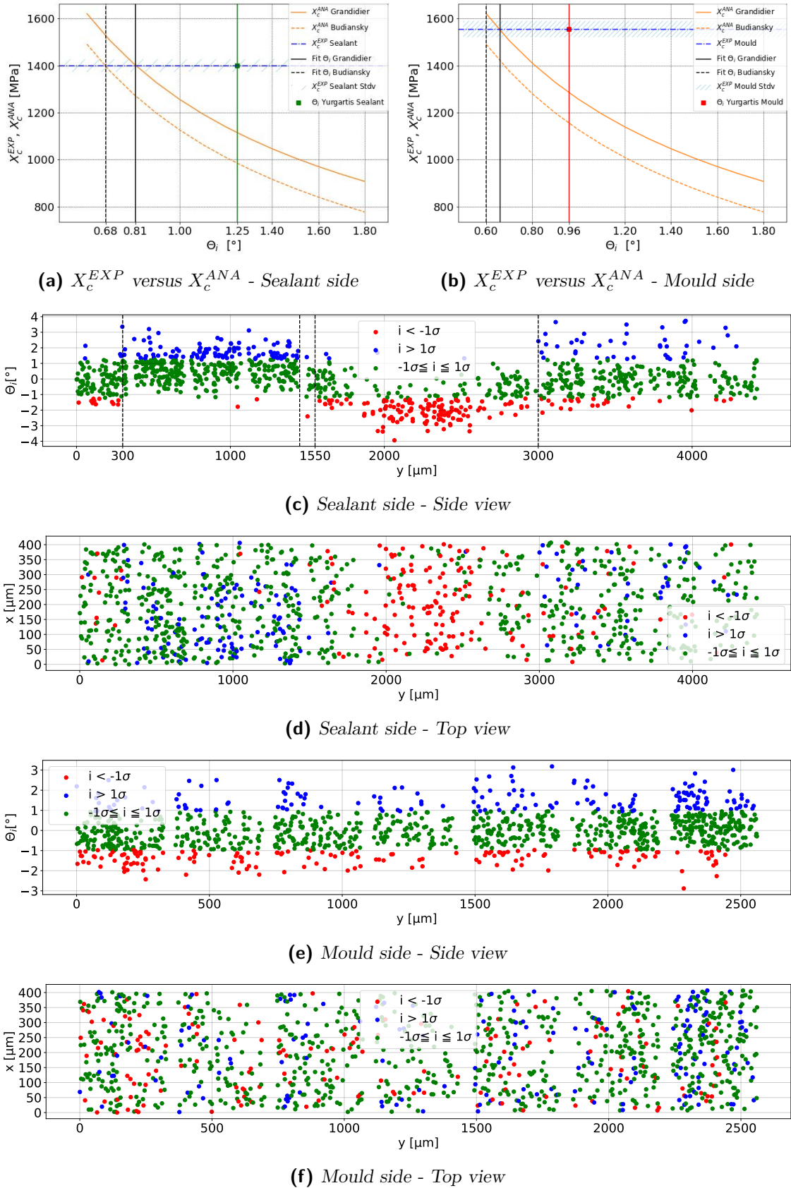
Fig. 4.12. Series 7 - M79/IM2C - Out-of-plane fibre misalignment \Theta_i .
