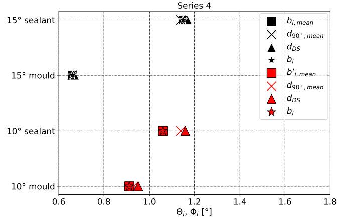
Fig. A.1. Confrontation of fibre misalignment angles as a function of different fibre diameters for series 4.
