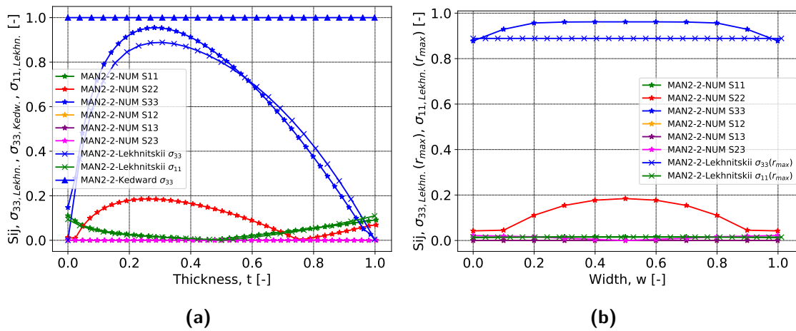
Fig. B.12. Normalized calculated stresses and strains S_{ij} , and analytically estimated radial and circumferential stresses \sigma_{33, \text{Lekhn.}} , \sigma_{11, \text{Lekhn.}} (Lekhnitskii) and \sigma_{33, \text{Kedw.}} (Kedward et al.) as a function of the normalized (a) thickness and (b) width of specimen MAN-02.
