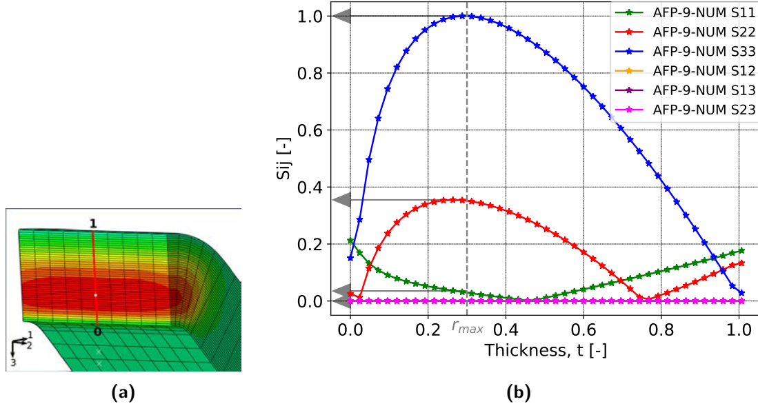
Fig. 7.11. (a) Node path along the specimen thickness over which the stresses S_{ij} were measured. The white measuring point corresponds to the same measuring point along the width (at r_{max} and at half the specimen width). (b) Normalized stresses S_{ij} as a function of the normalized mean thickness of L-beam specimen AFP-09. Arrows indicate the equal S_{ij} stresses at the common measuring point along the width (Fig. 7.12b).
