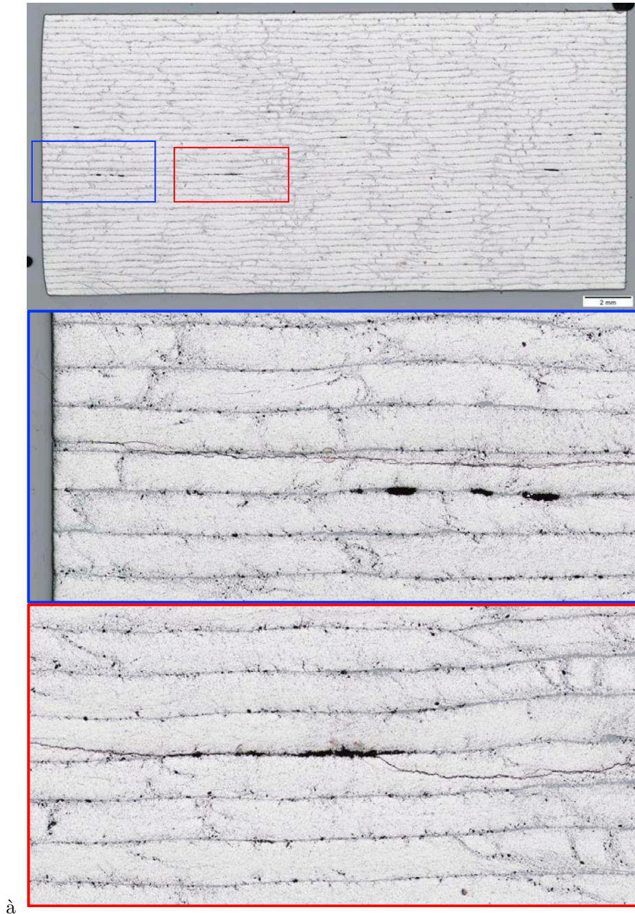
Fig. 9.6. Cross section of L-beam specimen MAN-06. The crack path is mostly intralaminar and interlaminar when pockets of porosity are given.
