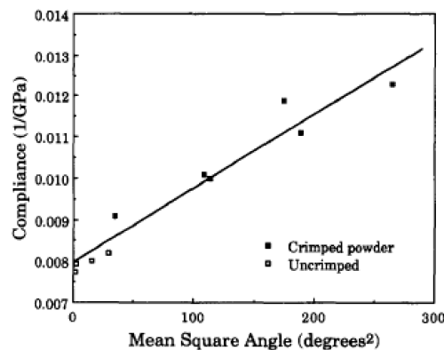
Fig. 2.8. Compliance of laminates (estimated at zero strain) as a function of the mean square fibre misalignment angle for crimped and non-crimped preregs. The deviation of crimped preregs is higher than for non-crimped ones. [Mrse & Piggott, 1993]
