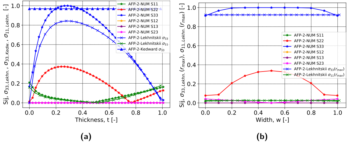
Fig. B.4. Normalized calculated stresses and strains S_{ij} , and analytically estimated radial and circumferential stresses \sigma_{33, Lekhn.} , \sigma_{11, Lekhn.} (Lekhnitskii) and \sigma_{33, Kedw.} (Kedward et al.) as a function of the normalized (a) thickness and (b) width of specimen AFP-02.
