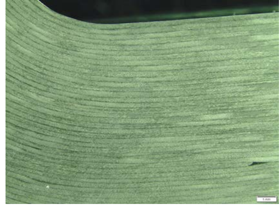
(a) AFP-09, microstructure of the L-beam's arm. (b) AFP-09, microstructure of curved segment.
