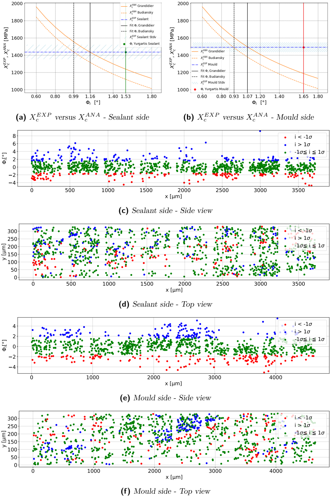
Fig. 4.11. Series 6 - MTC9810/T800S - In-plane fibre misalignment \Phi_i .
