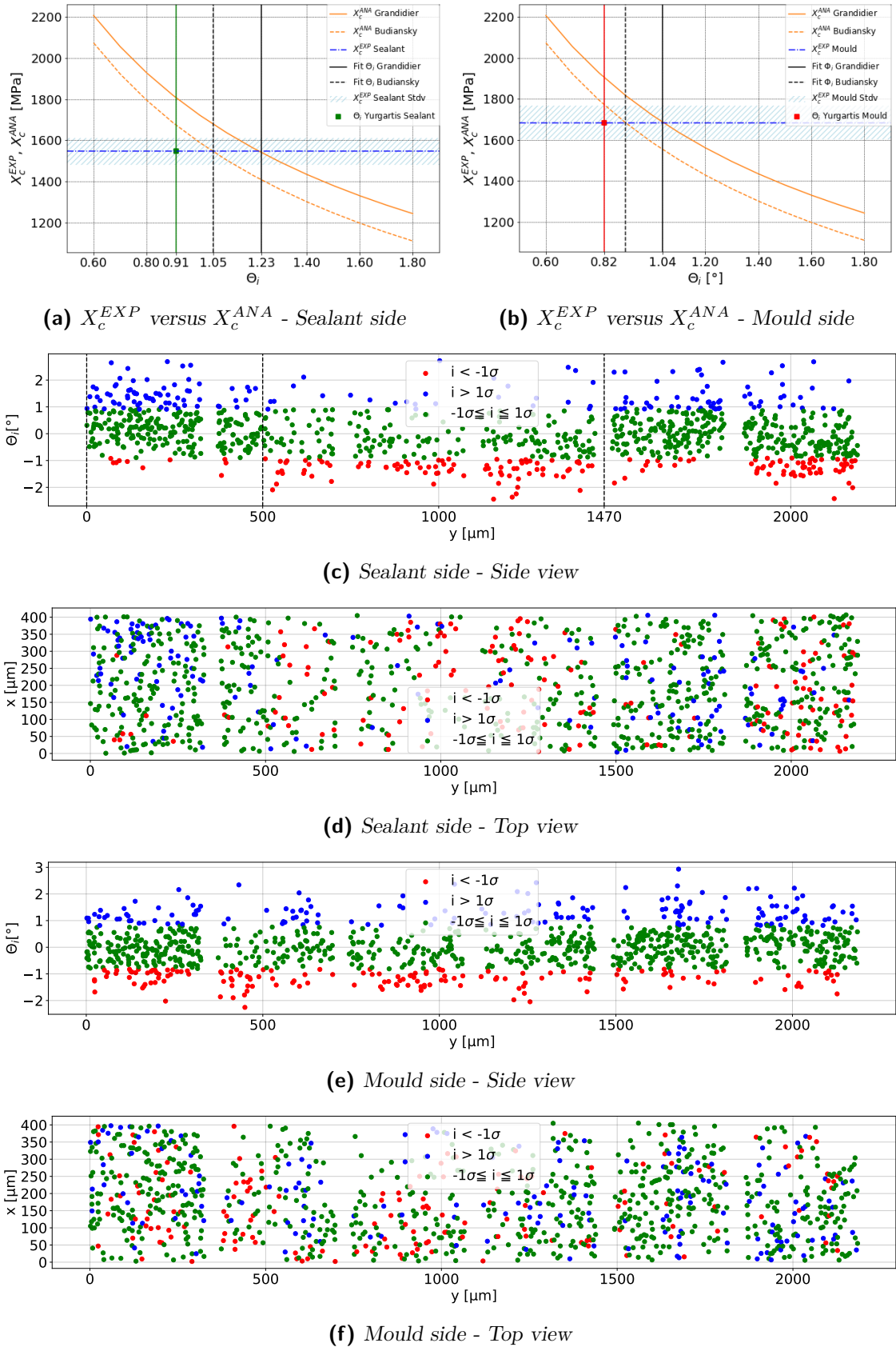
Fig. 4.4. Series 3 - SE84 LV/IM2C - Out-of-plane fibre misalignment \Theta_i .
