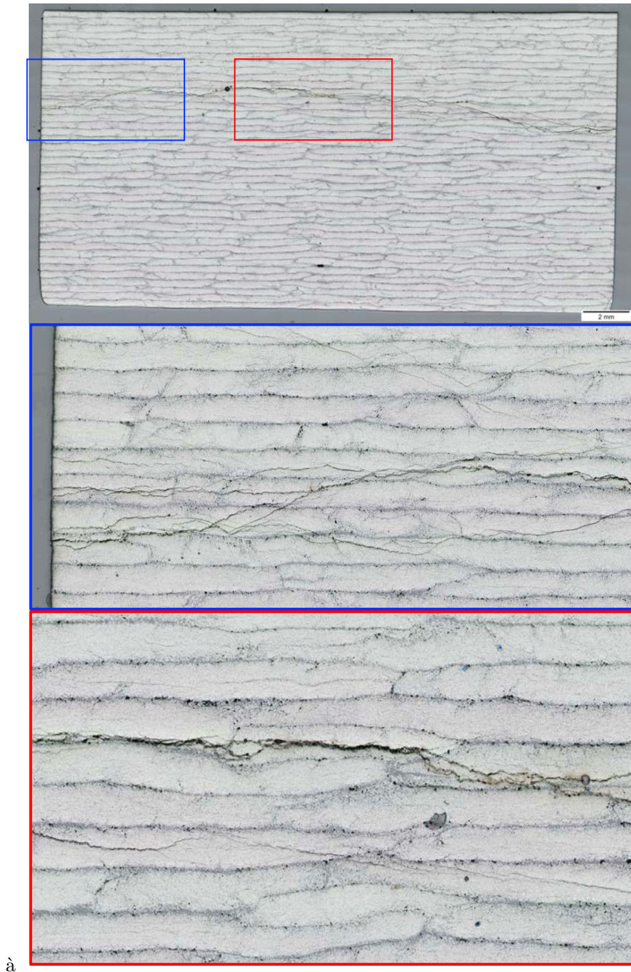
Fig. 9.7. Cross section of L-beam specimen AFP-09. The porosity is more diffuse and located between the tapes, so that "between" and "inside" each ply. The crack is translaminar, running through several plies (up to 6).
