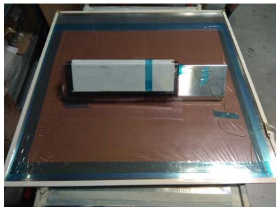
Fig. 8.6. Positioning of PC caul-plate and application of thermocouple.
