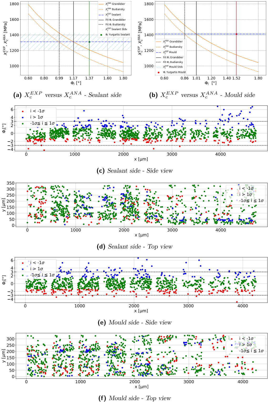
Fig. 4.9. Series 5 - XB3515/IMS65 - In-plane fibre misalignment \Phi_i .
