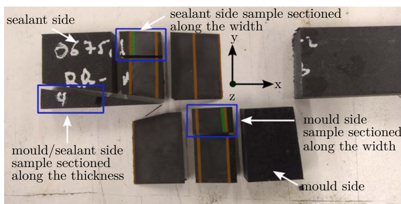
Fig. 3.11. Example of a specimen that was sectioned along the width and along the thickness. The samples used in the present study for the fibre misalignment determinations are framed. Those samples contain the zones of interest (marked in green for specimen sectioning along the width) in which at least 1000 ellipses were analysed. Orange zones mark the \pm 45 plies.
