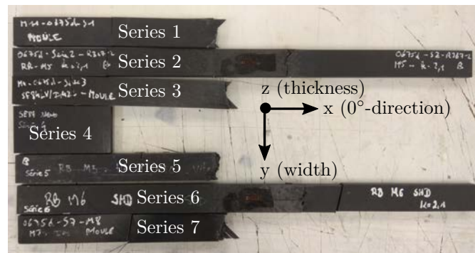
Fig. 3.1. Specimens from 4PB tests taken to determine the fibre misalignment angles according to Yurgartis' method.
