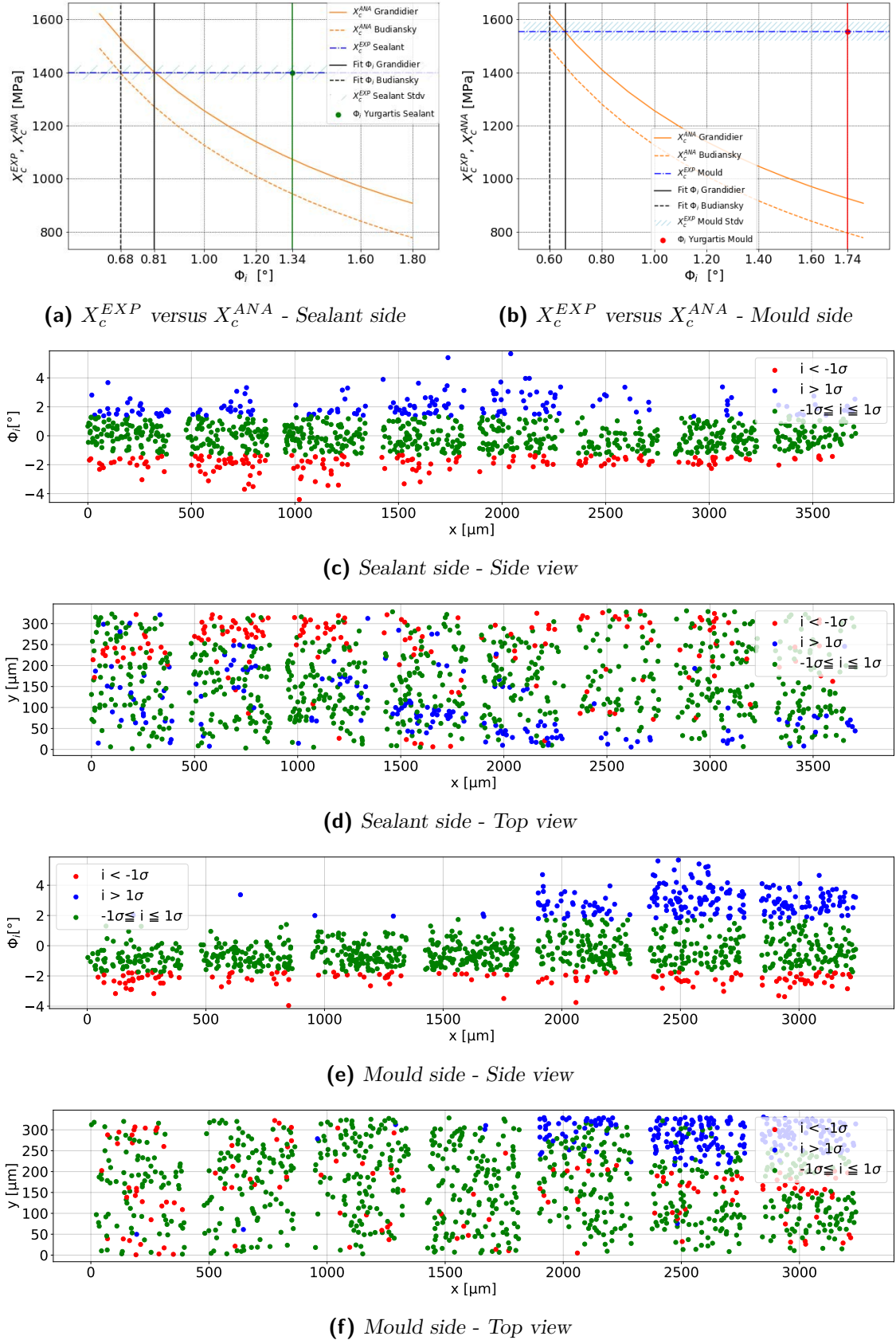
Fig. 4.13. Series 7 - M79/IM2C - In-plane fibre misalignment \Phi_i .
