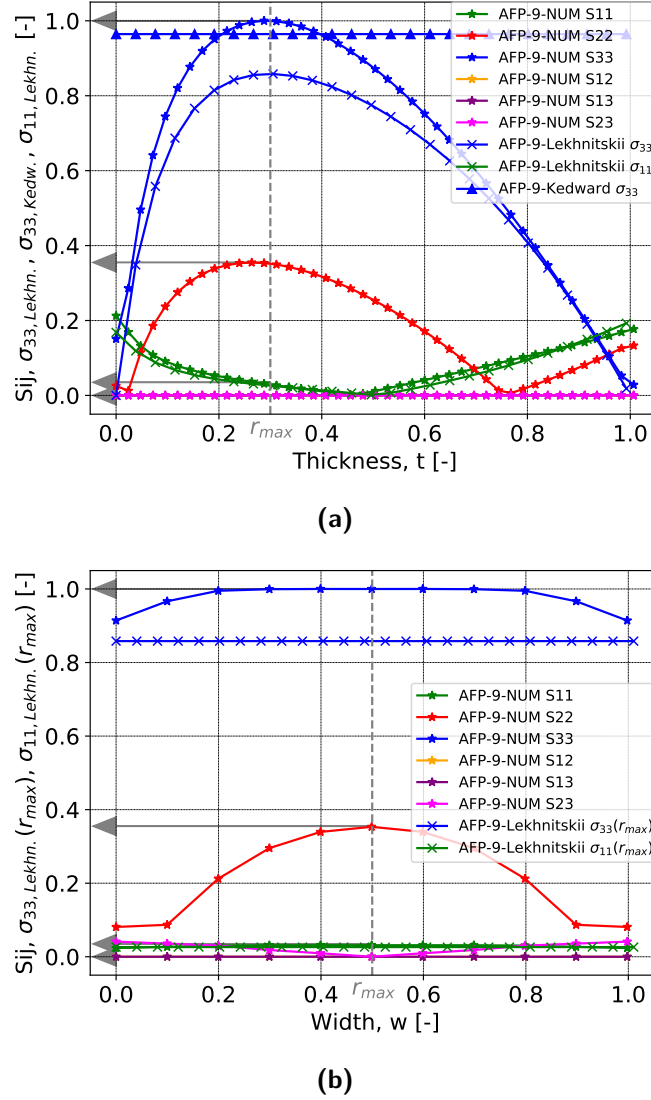
Fig. 7.14. Normalized stresses S_{ij} and analytically estimated radial and circumferential stresses \sigma_{33, Lekhn.} , \sigma_{11, Lekhn.} (Lekhnitskii) and \sigma_{33, Kedw.} (Kedward et al.) as a function of the normalized (a) thickness and (b) width of L-beam specimen AFP-09. Arrows indicate the equal stress values at half the specimen width along the width, and at r_{max} along the thickness.
