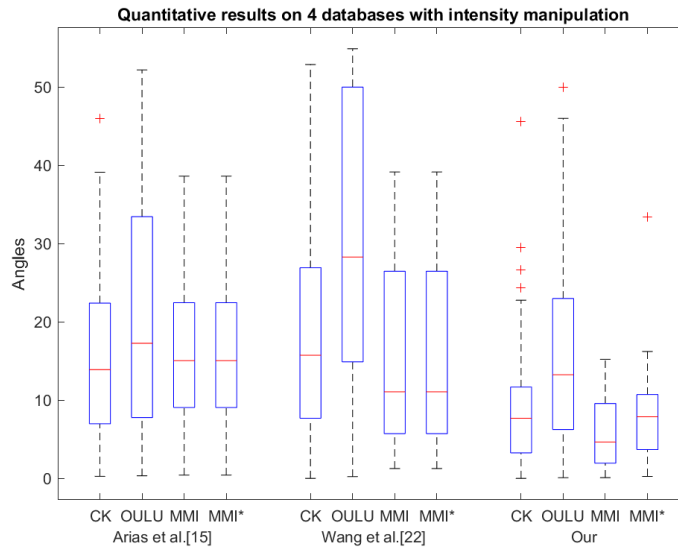
FIGURE 4.13 Representation of the angles calculated with the 3 methods on the 4 databases CK, OULU, MMI* and MMI* for the landmark of the left corner of the mouth for all the subjects.
