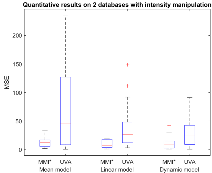
FIGURE 4.15 Representation of the results of the MSE of 2 databases MMI* and UVA-NEMO.
