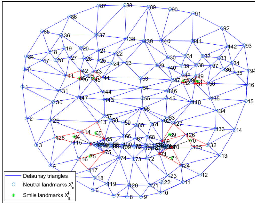
FIGURE 3.7 Positions of the smiling landmarks relative to the neutral landmarks. Each landmark of the smiling face is inside a triangle of the neutral face.
