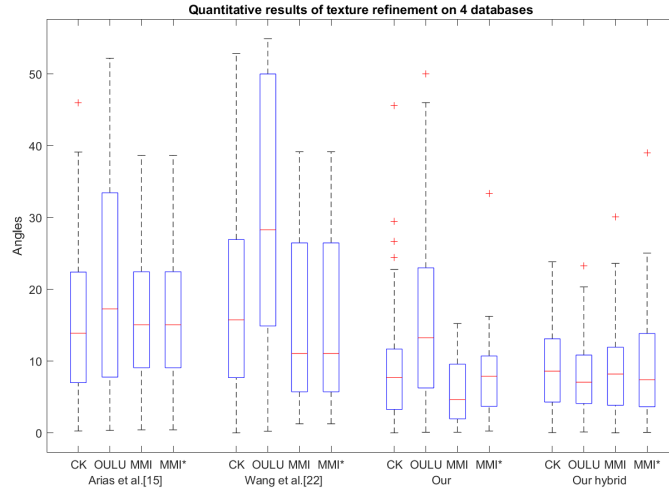
FIGURE 4.19 Representation of the angles of refinement results on the 4 databases with the different methods.
