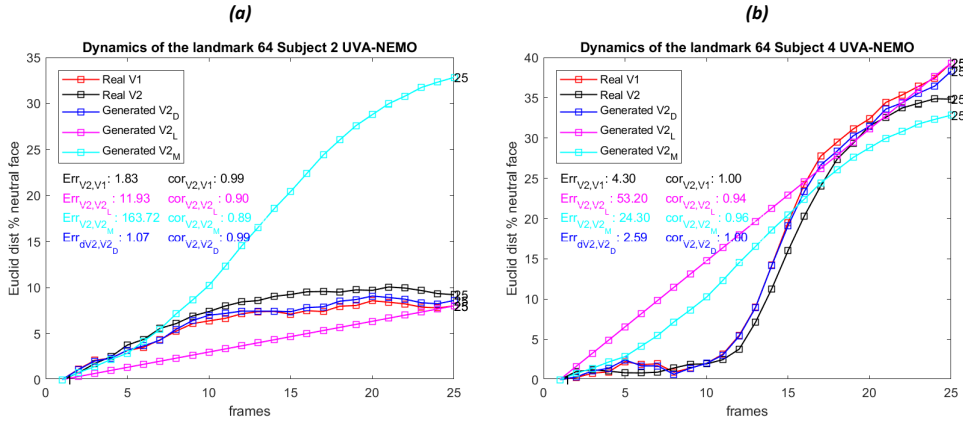
FIGURE 4.14 Example of the generated and real smile dynamics of 2 subjects. We notice that the dynamic model (blue) respects the Neutral-Apex time for each subject unlike the model based on amplitude (magenta) \widehat{V2}_L or the average model (cyan) \widehat{V2}_M . The intensity of the expression in (a) (Apex) is taken into account by the dynamic model \widehat{V2}_D but not with \widehat{V2}_L and \widehat{V2}_M models. Moreover, the target intensity is usually achieved by the dynamic model \widehat{V2}_D .
