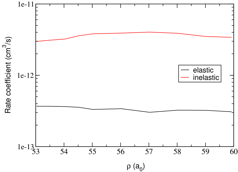
Figure 8.6: Elastic (black curve) and inelastic (red curve) rate coefficients as a function of the hyperradius. The initial channel chosen is ( v = 6, j = 0 ) and the relative kinetic energy is E_k = 500 nK.
