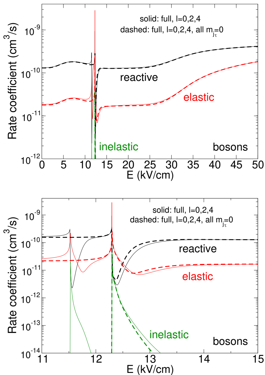
Figure 5.3: Rate coefficients as a function of the electric field for bosonic ^{41}\text{K}^{87}\text{Rb} for a collision energy E_k = 500 nK. Black line: reactive process, red line: elastic process, green line: inelastic process. Solid lines: complete treatment, dashed lines: complete treatment but with all m_{j_r} = 0 .
