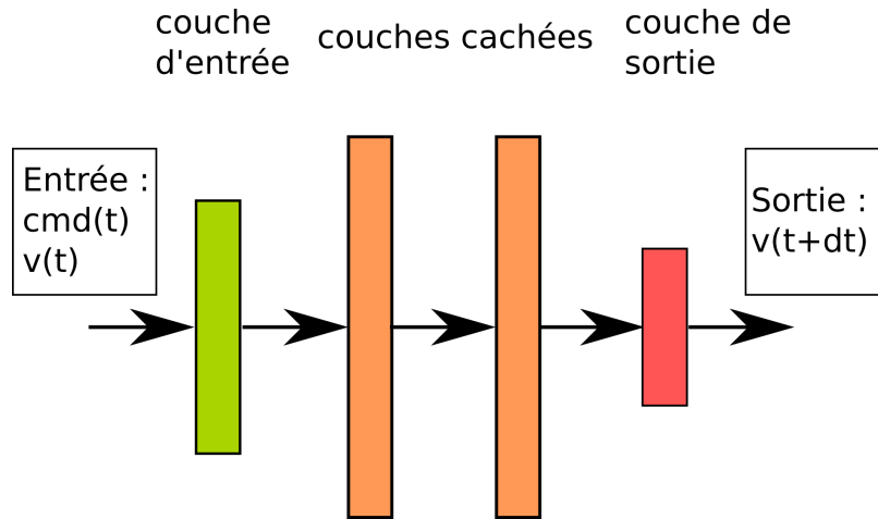
FIGURE 4.4 – Perceptron multi-couches.
