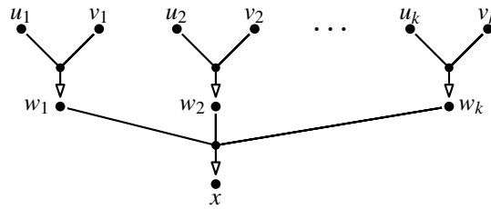
Figure 1.6 – The directed hypergraph associated to \Sigma .
