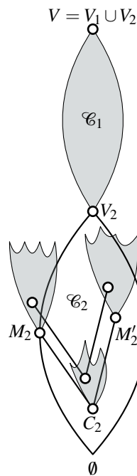
Figure 2.19 – Computing extensions of a closed set using extensions of meet-irreducible elements of \mathcal{C}_2 .
