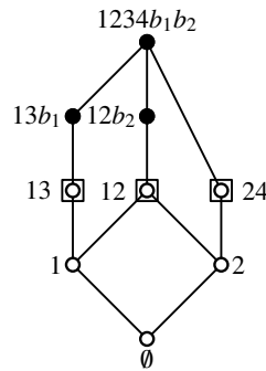
Figure 3.8 – The closure system \mathcal{C}_r derived from \mathcal{C} in Example 46.
