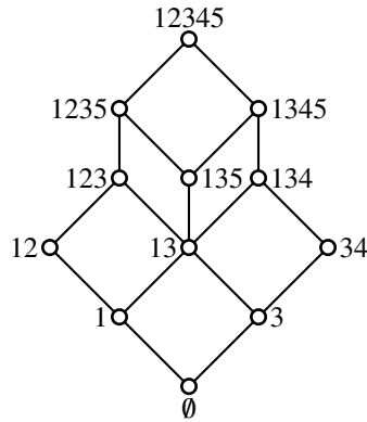
Figure 1.5 – A closure system \mathcal{C} over \{1, 2, 3, 4, 5\} .
