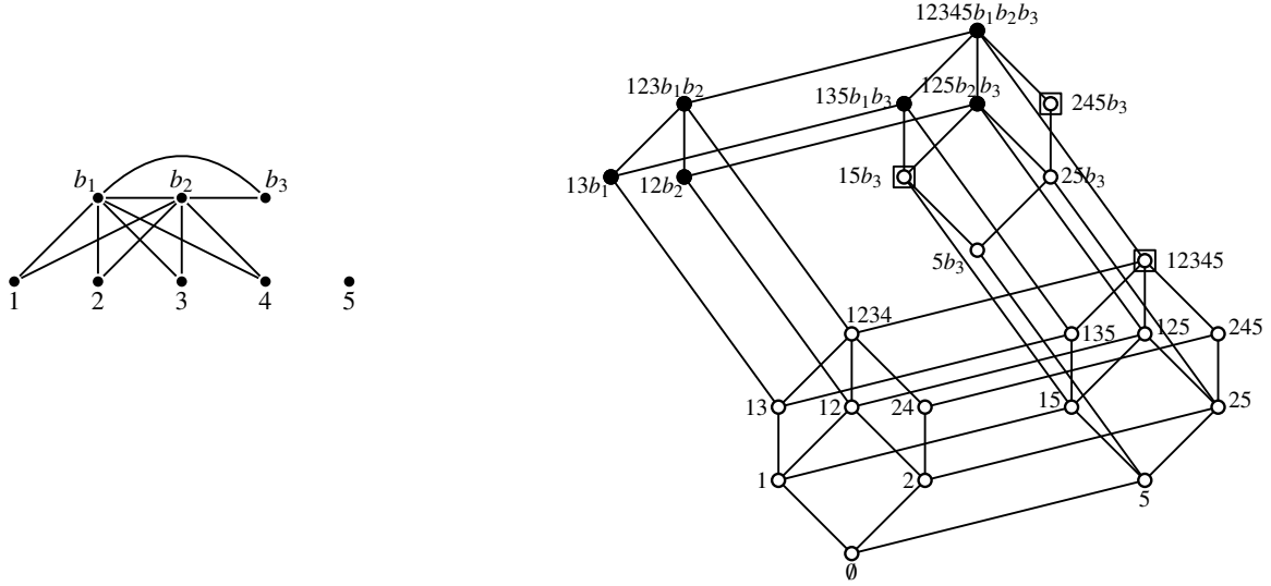
Figure 3.9 – The closure system \mathcal{C}_r derived from \mathcal{C} in Example 47.
