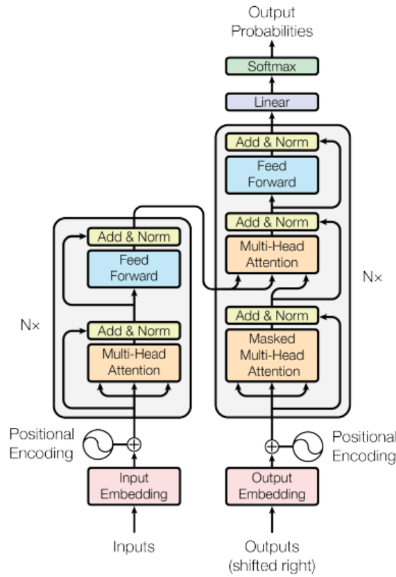
Figure 6.4: Architecture of the Transformer model. The image is adapted from [32].
