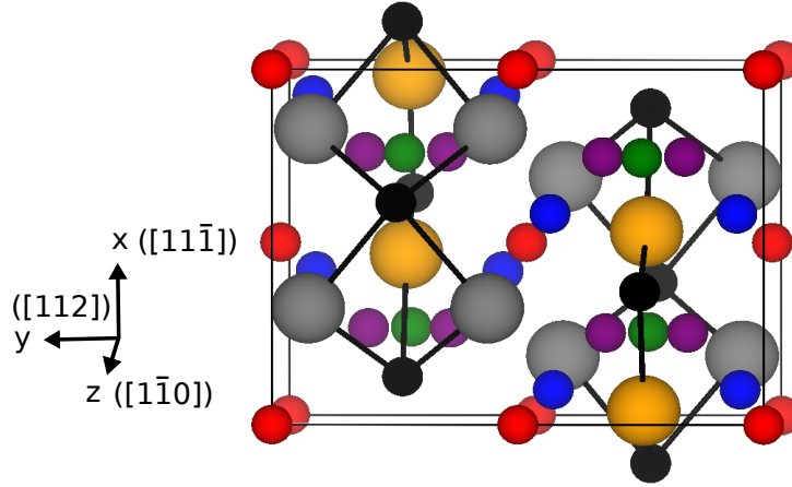
FIGURE 2.2: Crystal structure of Fe 3 C cementite. Larger atoms are Fe atoms. Fe s atoms are in orange, while Fe g atoms are in grey. Smaller atoms are C atoms. C atoms forming the ideal cementite structure (C intrinsic atoms) are in black. Interstitial octahedral sites for C are in red. T1, T2 and T3 sites are in green, blue and purple, respectively.
