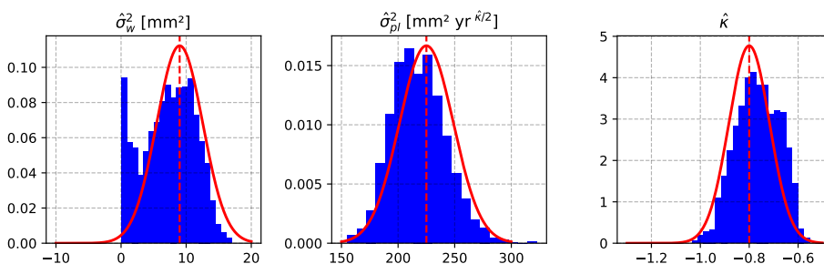
FIGURE 8.2: Distribution of variance component estimates obtained using the non-negative nonlinear LS-VCE method for the WN+PL stochastic model (blue histogram). True variance component (dashed red line). Normal distribution centred on the true value, with variance computed using Equation (8.13) based on the true variance components in Table (8.1) (solid red line).
