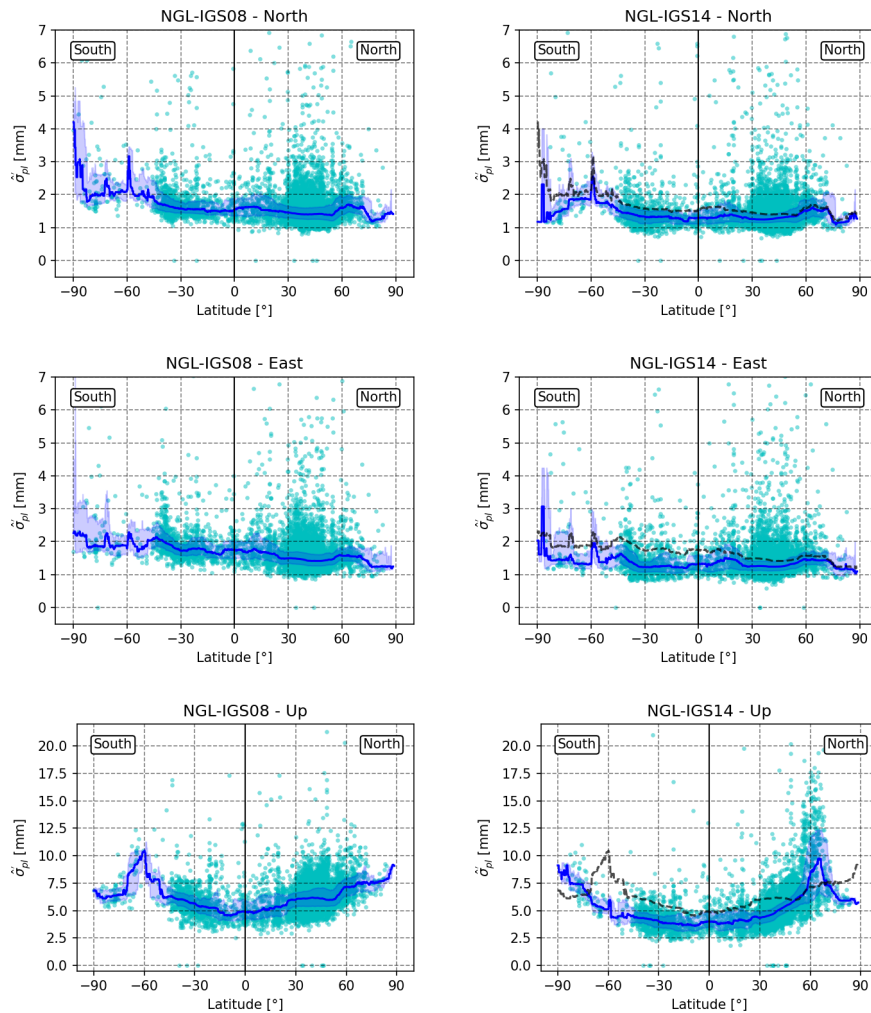
FIGURE 10.8: Latitude dependence of power-law process amplitudes \hat{\sigma}_{pl}^l for the North coordinate ( top ), for the East coordinate ( middle ), for the Up coordinate ( bottom ), and for both the NGL-IGS08 solution ( left ) and NGL-IGS14 solution ( right ). The dots in cyan represent the raw estimates. The continuous blue lines represent running medians over centered 10^\circ latitude windows. The shaded areas represent the corresponding interquartile range. The dashed black lines correspond to the running median for NGL-IGS08, reported on the NGL-IGS14 results to ease the comparison.
