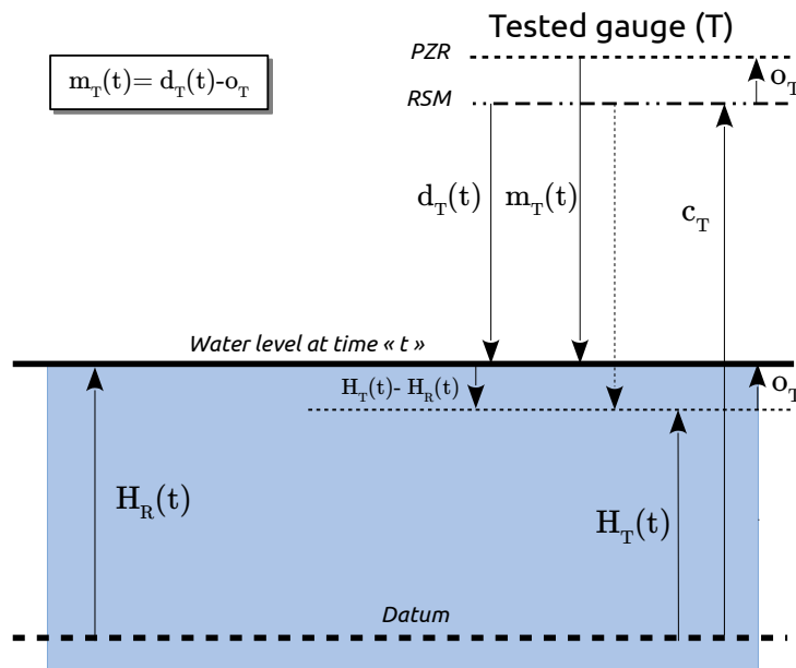
FIGURE 6.2: Configuration with an offset but no scale error. RSM: Reference Survey Mark. PZR: Point of Zero Range.
