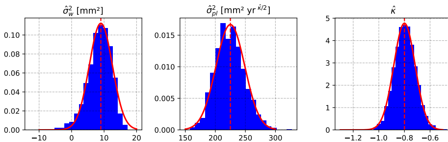
FIGURE 8.1: Distribution of variance component estimates obtained using the unconstrained nonlinear LS-VCE method for the WN+PL stochastic model (blue histogram). True variance component (dashed red line). Normal distribution centred on the true value, with variance computed using Equation (8.13) based on the true variance components in Table (8.1) (solid red line).
