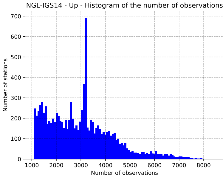
FIGURE 10.2: Histogram of the number of stations used as a function of the number of observations for the NGL-IGS14 solution and the Up coordinate.
