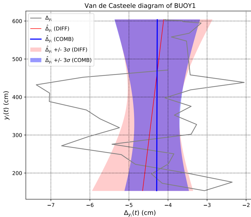
FIGURE 7.7: Van de Castelee diagram of BUOY1. The sea level bias model estimated with the COMB method is displayed in blue, and the one estimated with the DIFF method is displayed in red.
