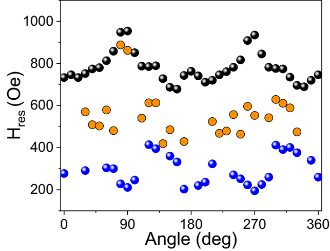
Figure 6.2: Angular resonance field dependence of the studied antidot arrays. Measurement was carried out at 8 GHz excitation field frequency with azimuthal angle varying from 0 to 360 degrees.
