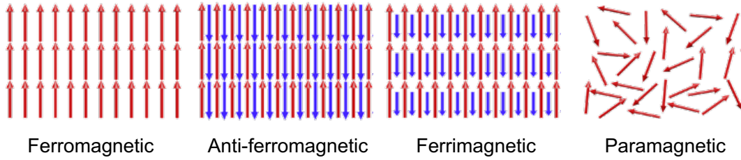
Figure 2.2: Magnetic materials classes. The ferromagnetic order exhibits an homogeneous magnetic moment modulus, the antiferromagnetic an alternative alignment of antiparallel magnetic moments of same modulus, the ferrimagnetic has the same distribution, antiparallel magnetic moment with different amplitudes and the paramagnetic class which shows a random spatial distribution of the magnetic moments.
