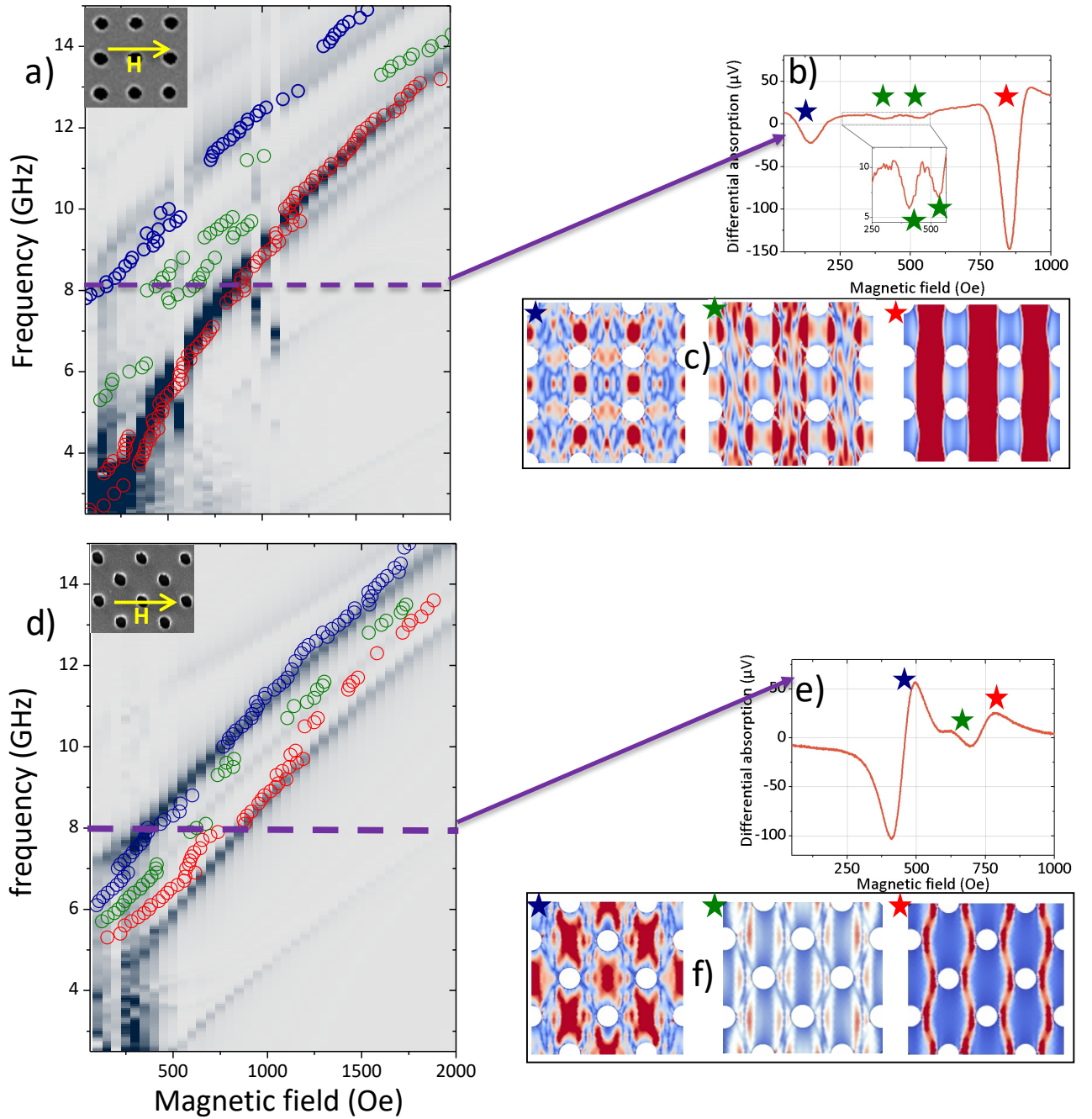
Figure 6.3: Experimental and numerical results obtained with a magnetic field applied along x -axis in absence of electric field for the two studied systems. a-c) SA system and d-f): CSA system. a),d)) Frequency as function of the applied magnetic field. The colors correspond to the relative power spectrum density obtained by micromagnetic simulations while the open symbols are experimental data. b),e) Typical experimental spectrum recorded at 8 GHz, the stars are used to identify the different peaks. c),f) Spin precession amplitudes at H = 750 Oe (applied along x -axis) obtained by micromagnetic simulations (spatial Fourier transform) showing the localization of the modes identified in the FMR spectra. The colors encode m_y component, the red part reflects a high precession amplitude while the blue one means zero precession amplitude. The stars inside the images correlate the mode profiles with positions in the FMR spectra (a) and d)).
