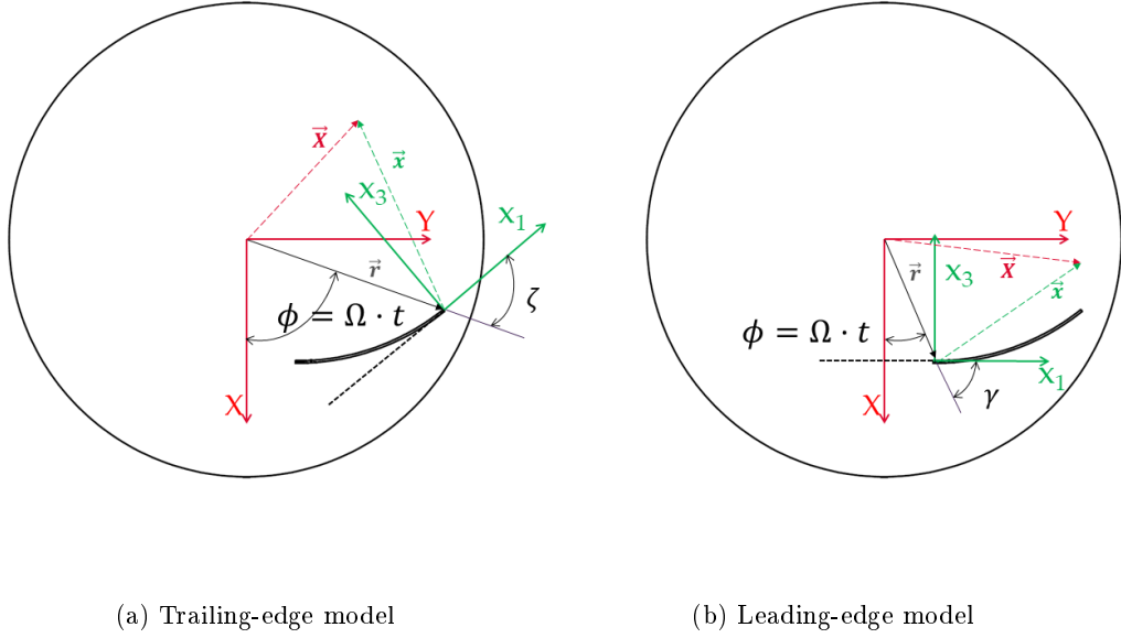
Figure 2.7 – Rotating and fixed reference frames
