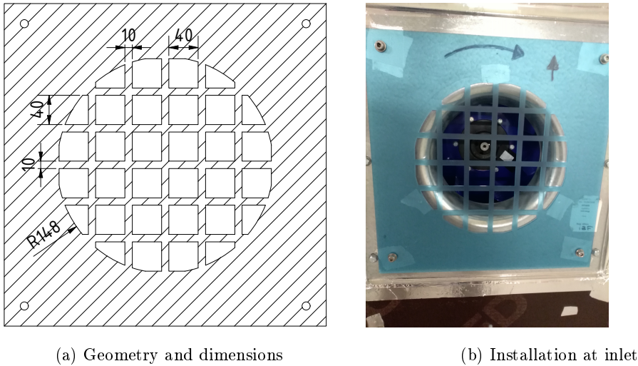
Figure 1.37 – Turbulence grid
