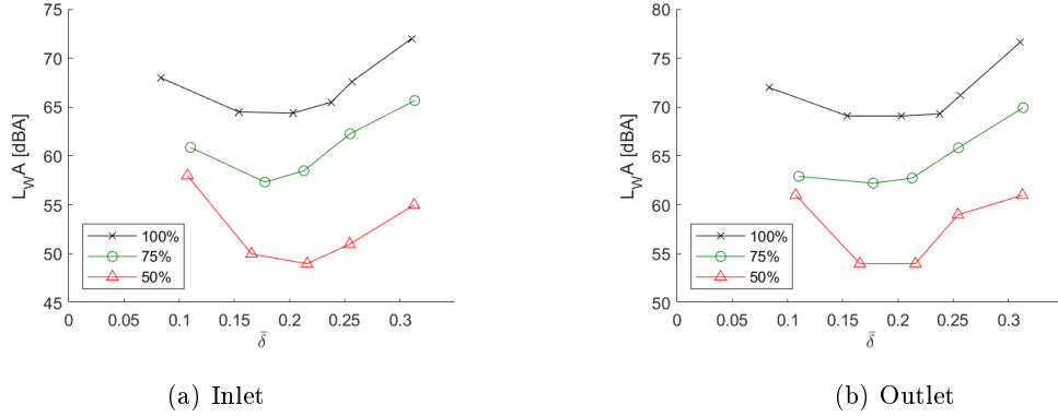
Figure 1.11 – Sound power level curves of the tested baseline fan
