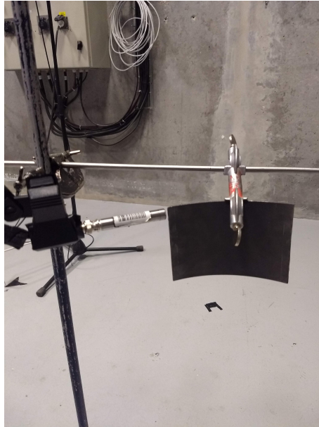
(b) Blade mock-up
