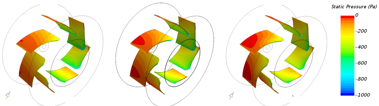
Figure 3.11 – Static pressure on the blades ( q_v = 1706, 2196, 2584 \text{ m}^3/\text{h} ), N=1440 rpm
