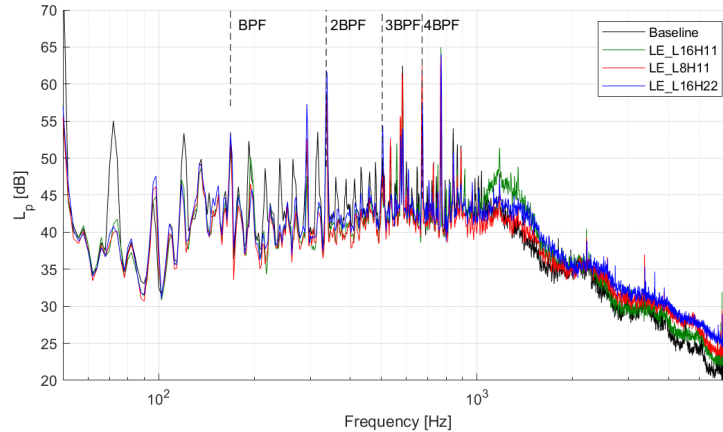
Figure 1.29 – Typical averaged narrowband sound pressure spectra at outlet for q_v = 2200 \text{ m}^3/h , N=1440\text{rpm} , \Delta f = 2 \text{ Hz}
