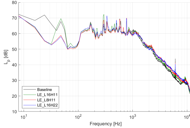
Figure 1.42 – Narrowband sound pressure spectra at outlet for the BEP q_v = 2200 \text{ m}^3/\text{h} , N=1440 rpm, \Delta f = 8 Hz
