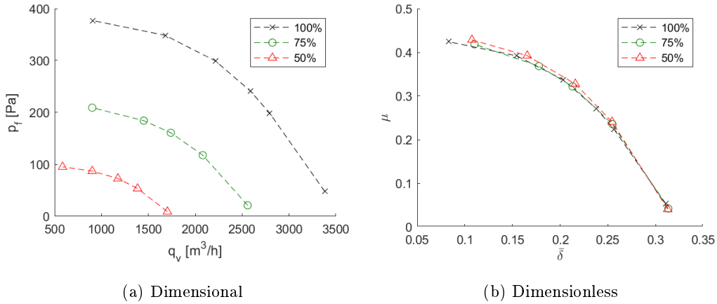
Figure 1.9 – Baseline fan pressure curves
