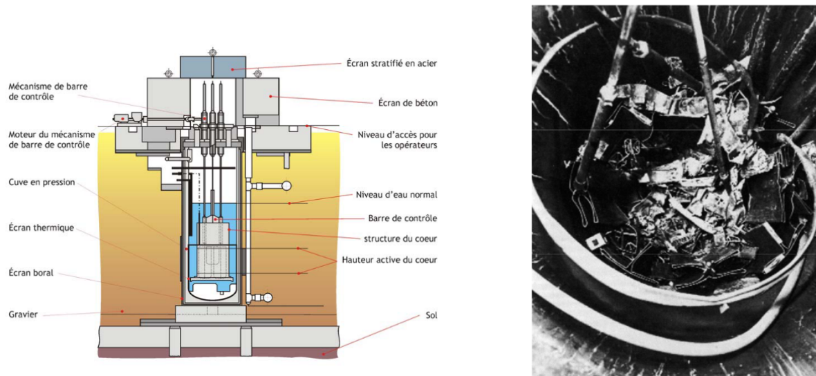
Figure 1: Schematic view of reactor SL-1 (left); three mechanism of control rods ("mécanisme de barre de contrôle" on the left figure) were damaged (right) after the BORAX-type accident in 1961 [Couturier, 2011].
