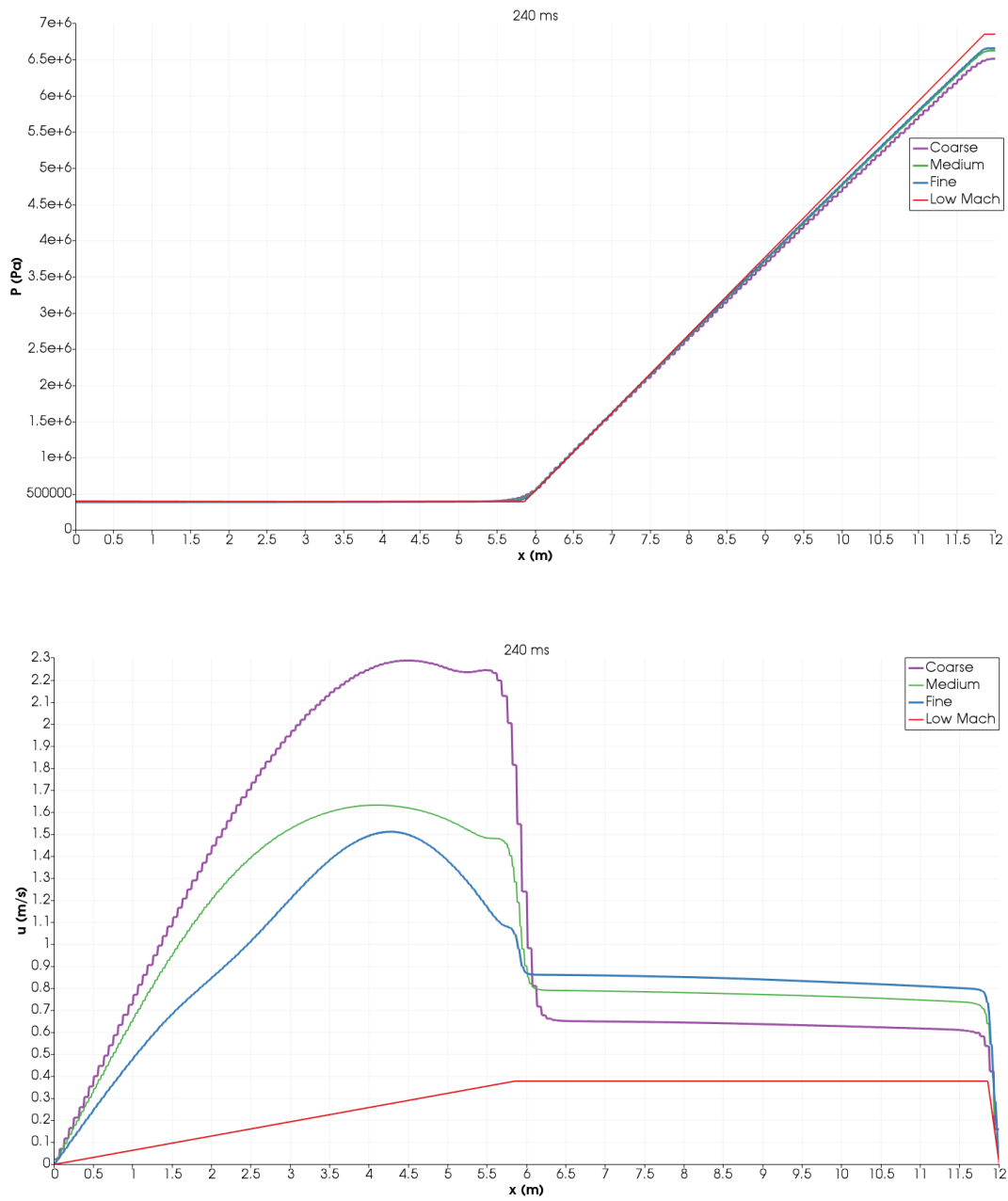
Figure 4.16: Weak bubble expansion problem (10 bars). Comparison between DEM and bubble (low-Mach) model. Pressure and velocity fields at 240 ms. Limited linear space reconstruction for primitive variables and 2-stage Runge-Kutta time discretization, CFL = 0.5 .
