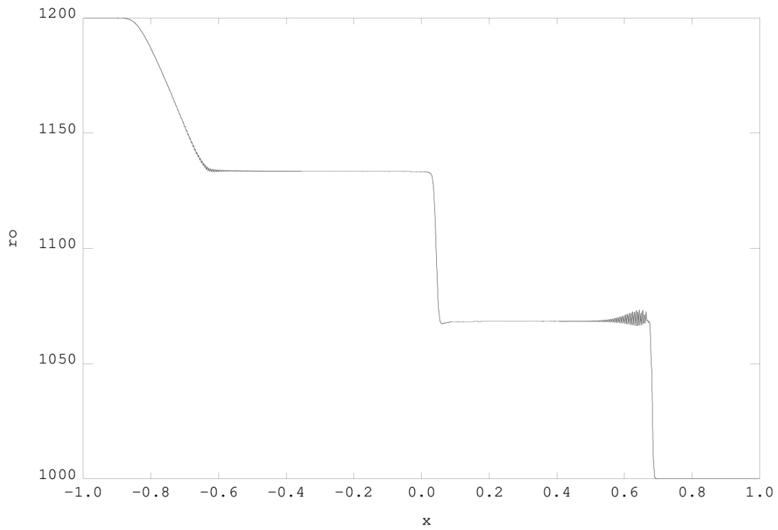
Figure 2.31: Computed density distribution for the 1D low-Mach shock tube problem. M_{\text{ref}} = 1 \times 10^{-1} . 4 \times (400 \times 1) elements. Triangular mesh. HLLCDL. Limited second order reconstruction in space, second order in time. Top t = 1 \times 10^{-4} . Bottom t = 4 \times 10^{-4} .
