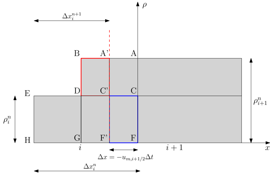
Figure D.2: Verification for the density solution: Density solution at t = t^{n+1} before taking the cell average
