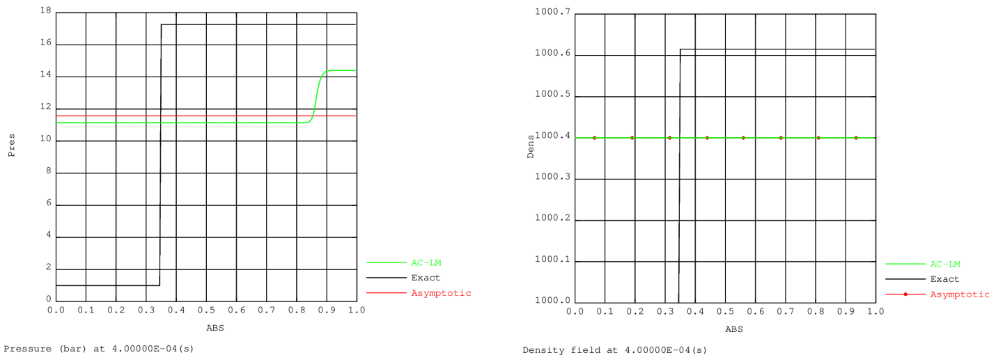
Figure 3.5: 1D planar piston problem. Comparison between the fully compressible solution (black), the asymptotic solution (red) and the new AC (AC-LM, 200 cells, green) solution. Pressure (left) and density (right) fields at t = 4.0 \times 10^{-4} s.
