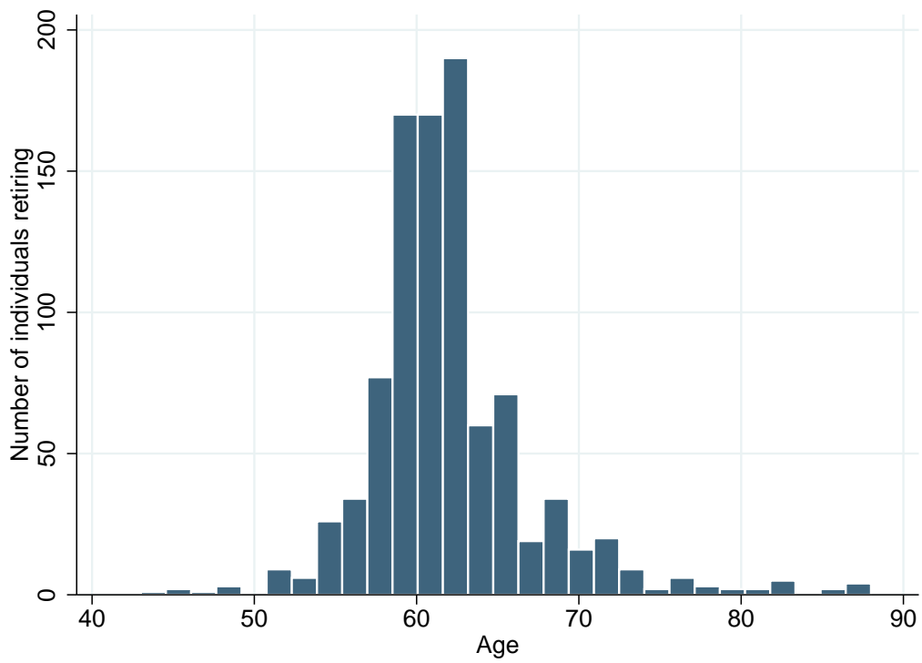
Figure A1. Number of individuals retiring by age
