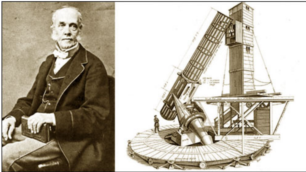
Figure 3.2: English astronomer William Lassell, Triton's discoverer. The 24 inch reflecting telescope depicted here was the instrument used in the discovery. It was completed in 1845, and was the first telescope to be mounted equatorially.
