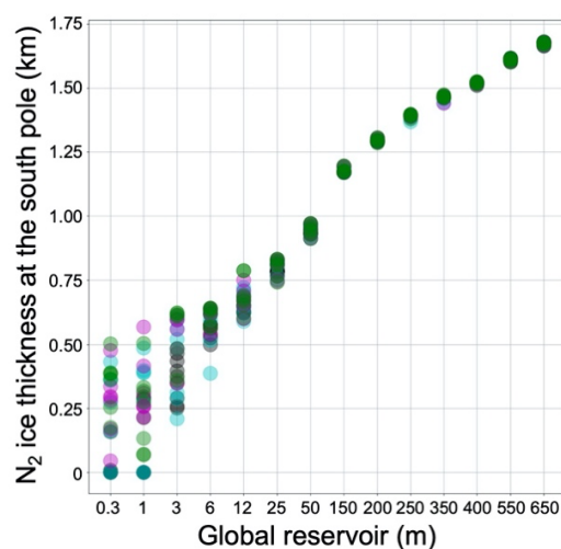
Figure 18: Modeled maximum \text{N}_2 ice thickness at the south pole in 1989 vs initial global \text{N}_2 ice reservoirs for all simulations performed with north-south \text{N}_2 ice albedo asymmetry, no internal heat flux. Colors indicate the thermal inertia (black: 200 SI; cyan: 500 SI; magenta: 1000 SI; green: 2000 SI). For large reservoirs greater than 25 m in global average, the maximum thickness of the ice at the south pole mostly depend on the reservoir (and not on the thermal inertia or albedo of the bedrock).
