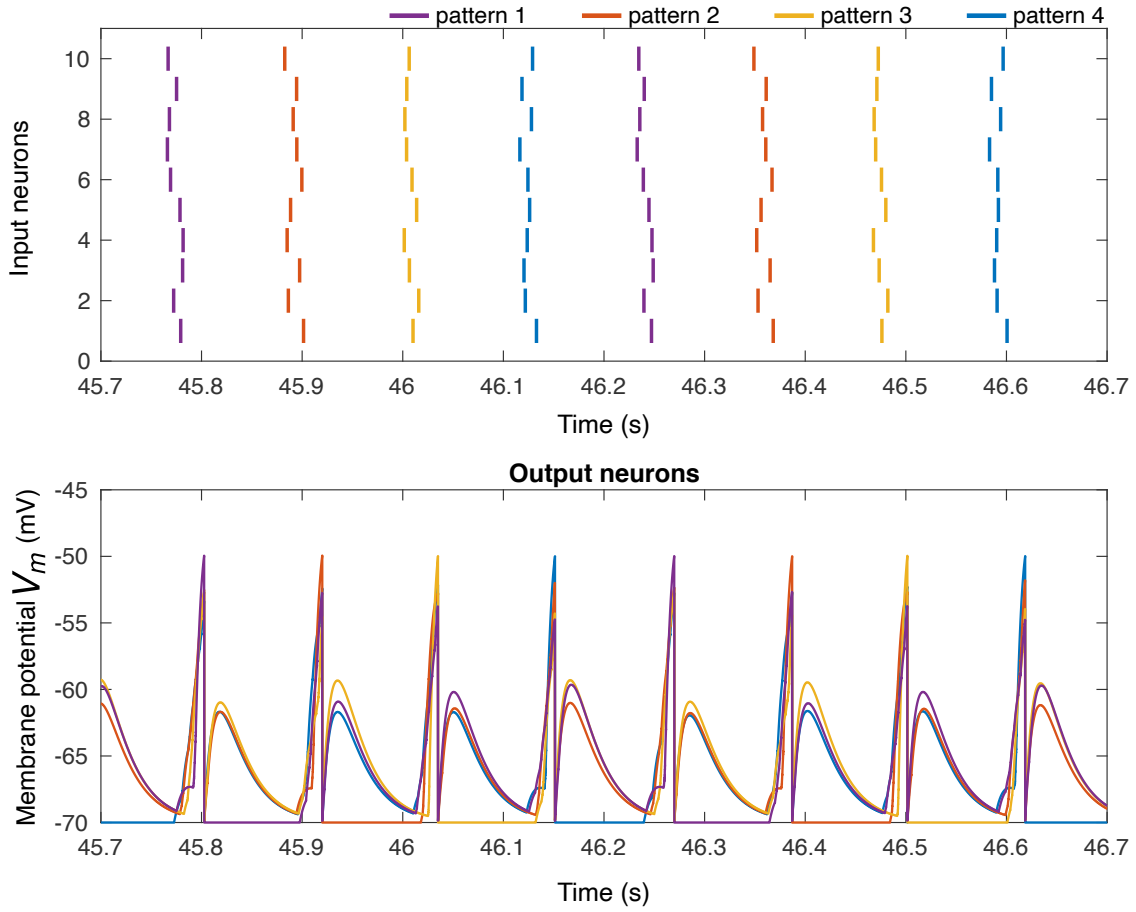
Fig. 2.3 Myelin plasticity learning rule on a one-dimensional pattern recognition tasks consisting of four different patterns, each with ten input neurons that fire at different times within a 20ms time window. ( Top ) Raster plot representing the four patterns in different colours. ( Bottom ) Membrane potential V_m for the four output neurons after training with the myelin plasticity rule. Each output neuron has maximised its membrane potential to a particular temporal pattern.
