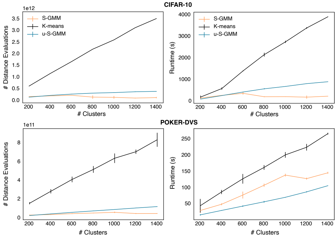
Fig. 4.6 Operations and Time Complexity analysis on CIFAR-10 and POKER-DVS for an increasing number of clusters. For a fair comparison with K-means , all algorithms were measured without any coresets on the full datasets. (Left) Operations complexity measure according to the number of distance evaluations. (Right) Time complexity in seconds.
