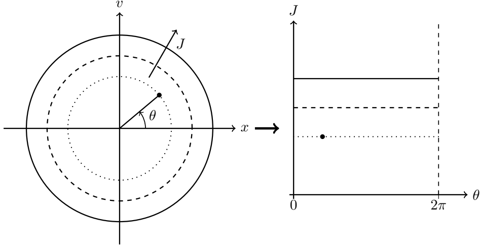
Figure 1.9: Extracted from Fouvy (2016) . Phase space diagrams of a unidimensional harmonic oscillator. Left panel: Particle's trajectories in (x, v) coordinates (position and velocity). In these coordinates, the dynamics is described in terms of trigonometric functions of time. The action (essentially the energy), however, is related to the size of the phase space circle, and is a constant of the motion. The angle runs over the circle. Right panel: Same phase space diagrams in the (\theta, J) plane. The angle being 2\pi -periodic, this plane is homeomorphic to a cylinder. In higher dimensions, the angle-action space is therefore homeomorphic to a torus.
