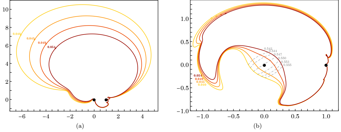
Figure 4.6: Nyquist diagram of the fastest growing mode of the model (\alpha, q) = (1, -6) , as given by the curves \omega_0 \mapsto \det[\mathbf{I} - \widehat{\mathbf{M}}(\omega_0 + i\eta)] , using the matrix method. (a) Nyquist diagram without rescaling. (b) Nyquist diagram after logarithmic rescaling (see the caption of Fig. 2.10 for details). Different colours are associated with different growth rates, while the changes in \omega_0 along each curve are indicated with the gray dashed lines. This diagram shows that the cluster supports an unstable mode with a growth rate, 0.045 \leq \eta \leq 0.049 , and oscillation frequency, 0.547 \leq \omega_0 \leq 0.550 .
