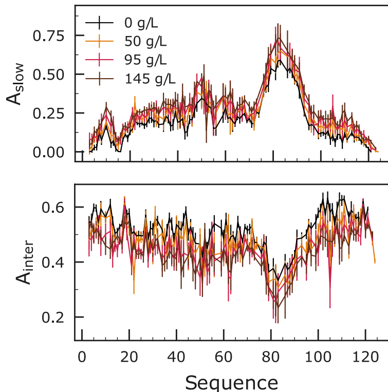
Figure 5.4: Amplitudes of slow and intermediate motions estimated from independent Model-Free analyses for different admixtures with Dextran40 at 298K, each optimizing two timescales, two amplitudes of motions with timescales of fast motions equal to 50 ps and CSA-DD angle \theta to 25°.
