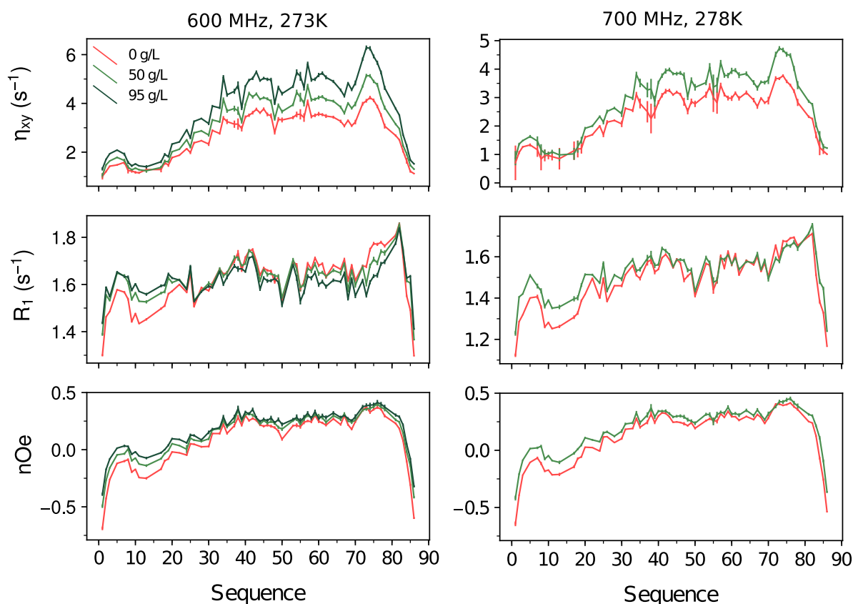
Figure 6.1: ^{15}\text{N} backbone relaxation rates of MKK4 for different admixtures with Dextran40, at magnetic field strengths of 14.1 and 16.4T at 273 and 278K.
