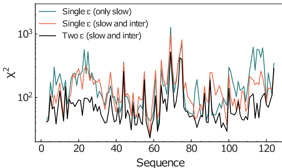
Figure 5.6: Comparison of \chi^2 for Einstein Model-Free analysis of relaxation rates of NTail at 298K, 600 and 850 MHz in admixtures with Dextran40 ranging from 0 to 195 g/L, optimizing two amplitudes, two timescales of motions at infinite dilution, CSA-DD angle \theta and one or two \epsilon for slow and intermediate motions.
