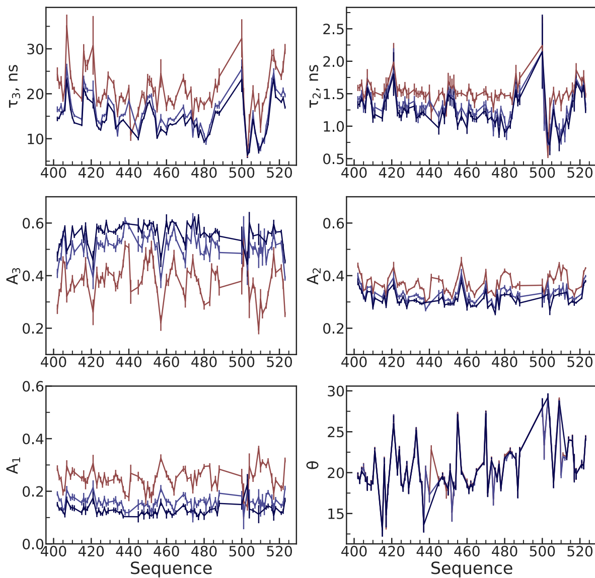
Figure 6.9: Comparison of the dynamic modes estimated using 5 parameter Model-Free analysis of relaxation rates in concentrated phase optimizing two amplitudes, two timescales and CSA-DD angle, assuming constant value of fast timescales of motions equal to 50, 75 or 100 ps (red, light-blue and blue respectively).
