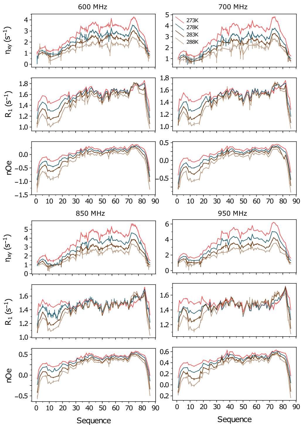
Figure 4.2: ^{15}\text{N} backbone relaxation rates of MKK4 at multiple field strengths (ranging from 14.1 to 22.3T here marked with respect to the proton Larmor frequency at which spectrometer operates) and temperatures (ranging from 273 to 288K).
