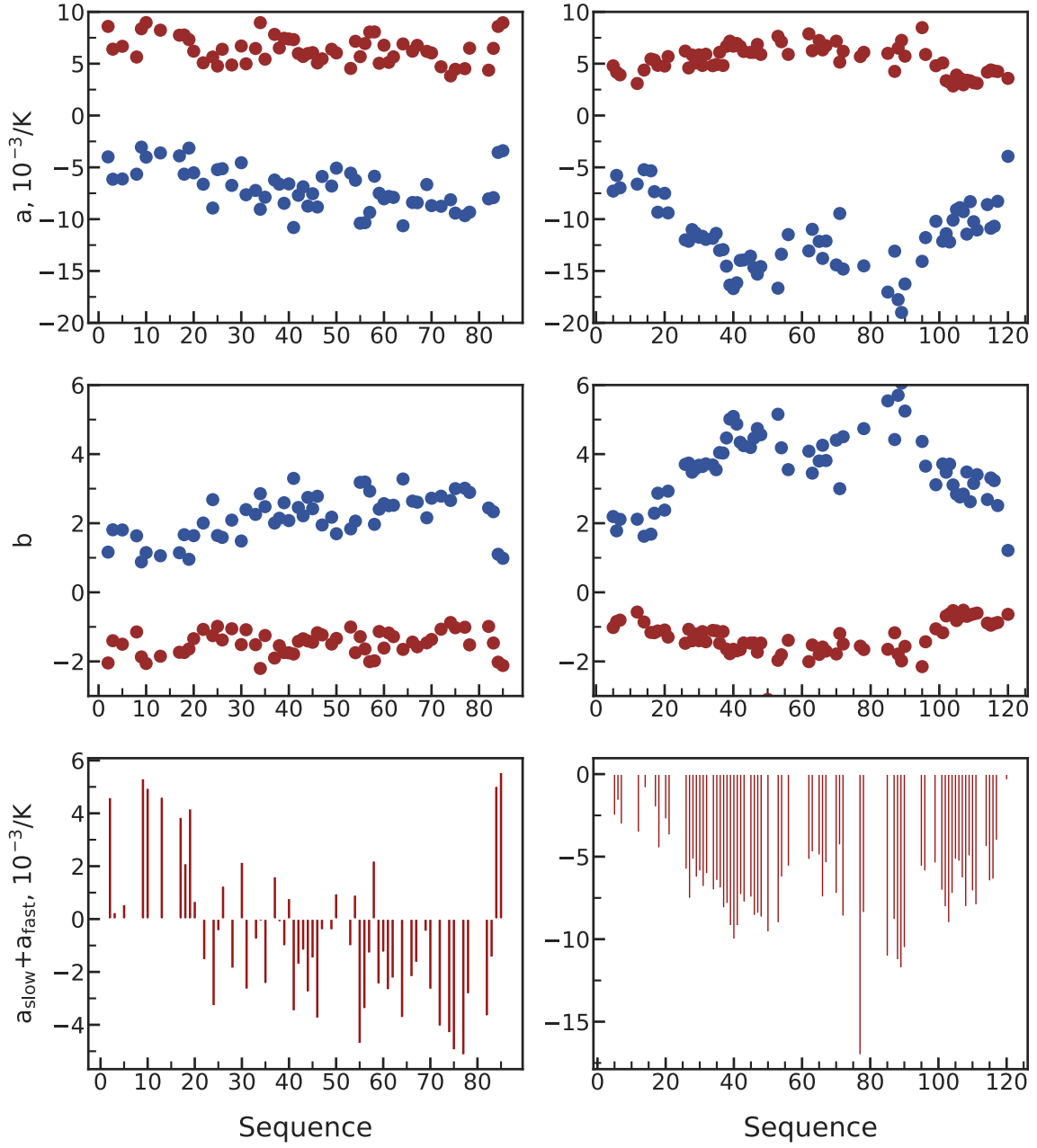
Figure 4.10: Comparison of parameters characterizing rate of change of amplitudes of motions with temperature for MKK4 and NTail model systems in temperature range of 273 to 288K and 274 to 288K for MKK4 and NTail respectively, brown and blue points represent parameters for fast and slow motions respectively.
