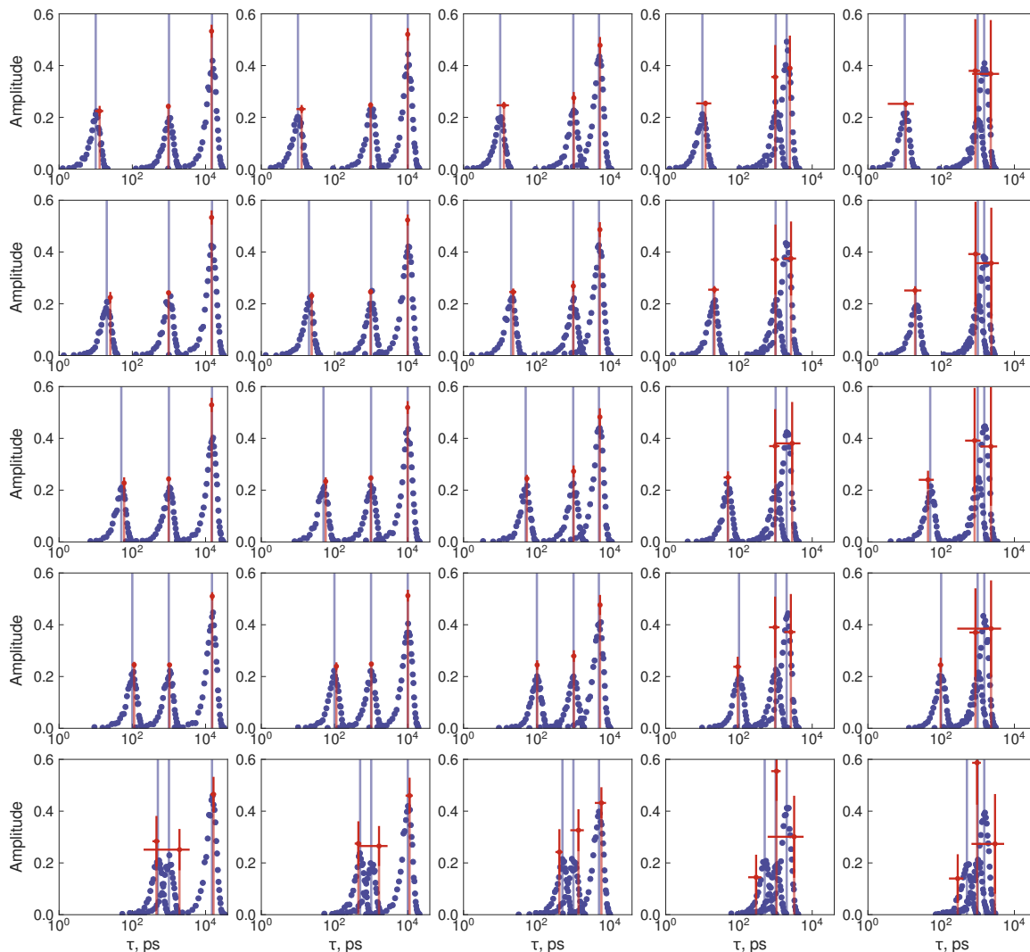
Figure App.5: Comparison of simulated distributions of correlation times used for calculation of relaxation rates with apparent dynamic modes estimated from Model-Free analysis of relaxation rates calculated on the basis of simulated correlation times (Population ratio: 1:1:2, \Omega = 0.3 ). Blue points represent distribution of simulated correlation times for each motion with average represented by blue bar. Orange points and bars represent average and standard deviation of estimated apparent dynamic modes on the basis of Model-Free analysis of relaxation rates calculated from simulated distributions of correlation times.
