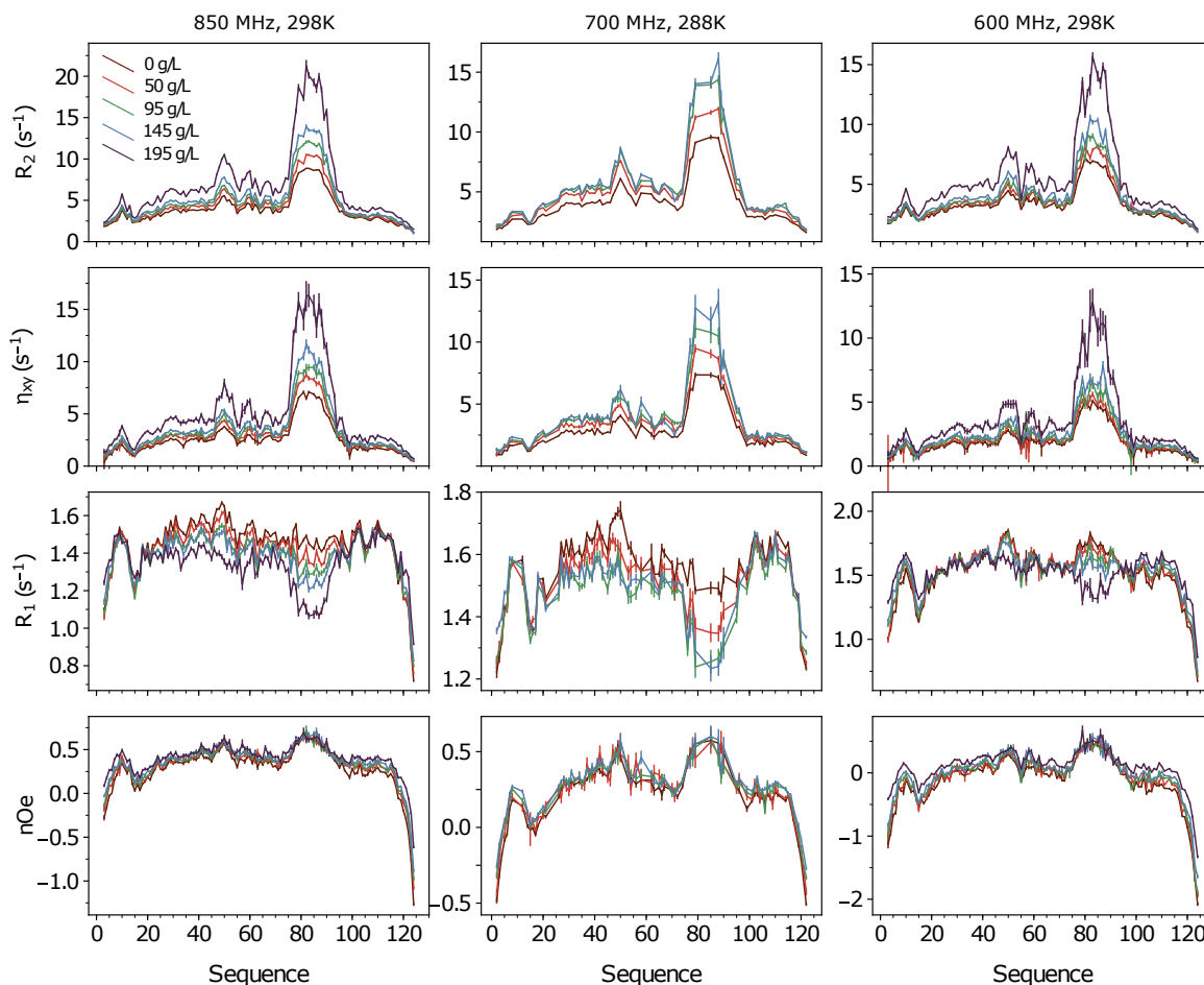
Figure 5.2: ^{15}\text{N} backbone relaxation rates of NTail measured in range of admixtures with Dextran40 (0 - 195g/L) at three magnetic fields and two temperatures.
