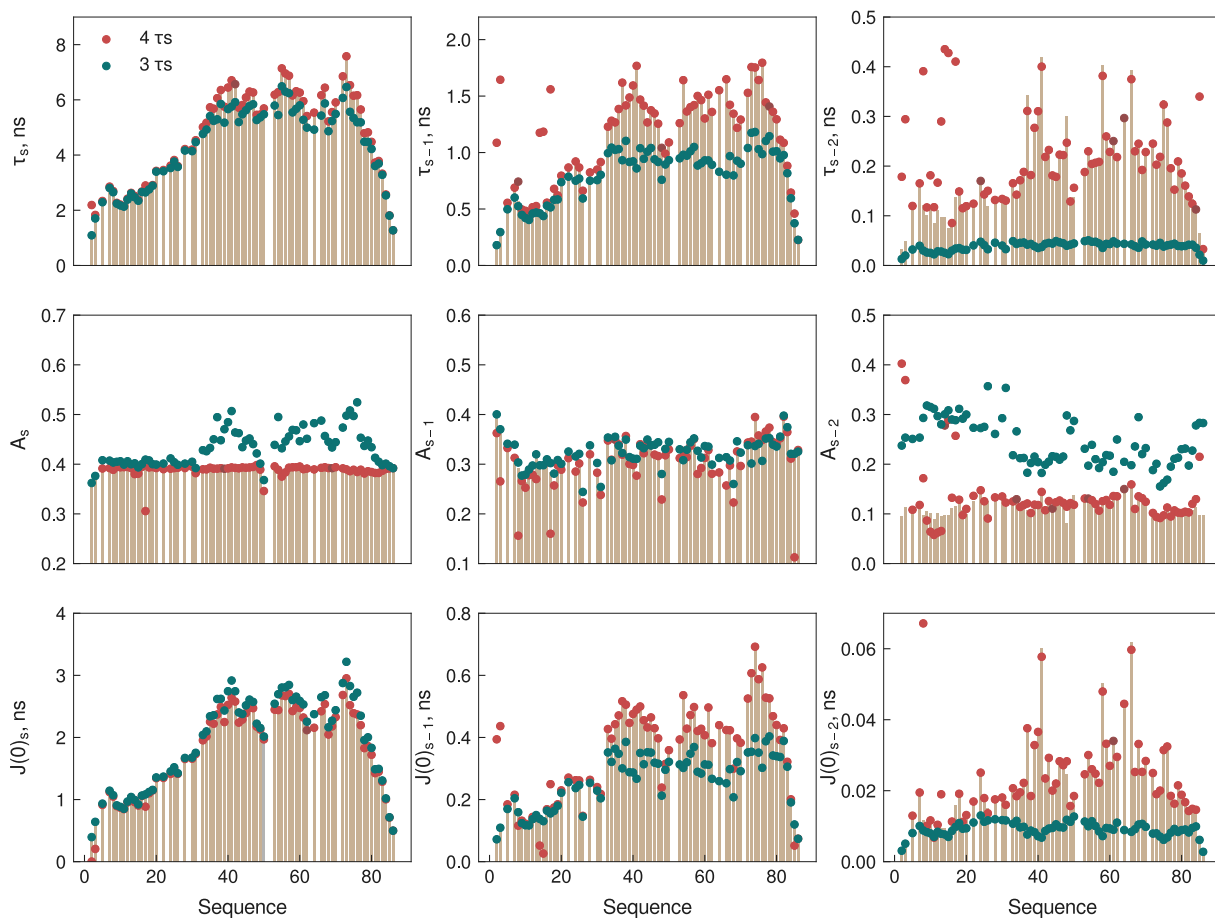
Figure 3.10: Comparison of dynamic modes for MKK4 (amplitudes and timescales of motions as well as their product - J(0) components, starting from the slowest one ( s ) obtained from the fit of average NH-backbone correlation function representing average over 40, 50 ns blocks of trajectories, and Model-Free analysis with three or four apparent dynamic modes of relaxation rates calculated on the basis of MD-derived NH-backbone dynamics with magnetic field strength ranging from 14.1 to 22.3T, at 278K.
