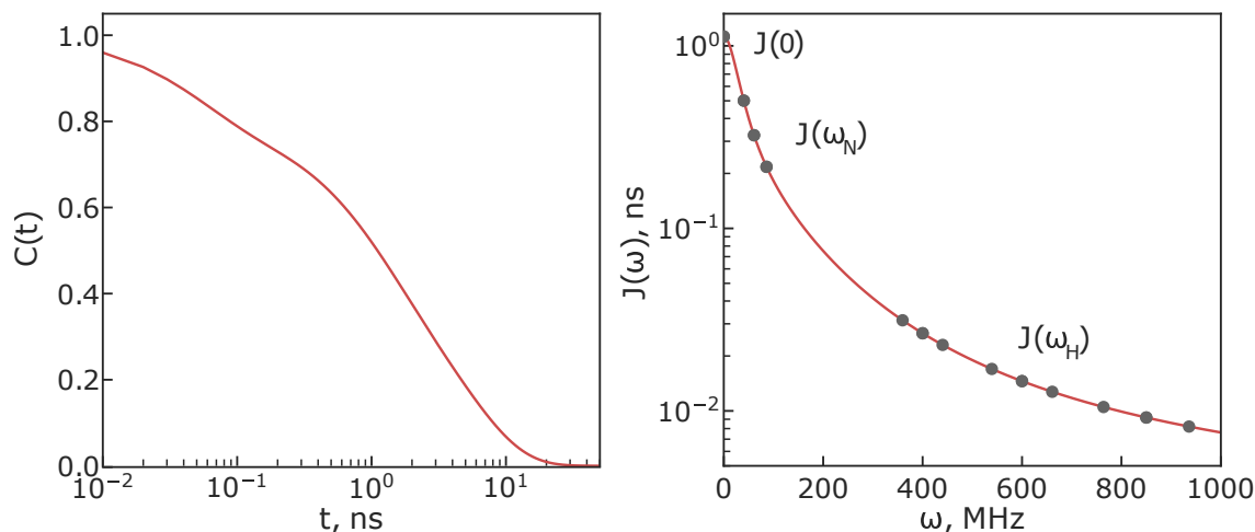
Figure 2.1: Comparison of exemplary correlation function and corresponding SDF. Points represent SDF at frequencies associated with nuclear spin interactions, i.e. Larmor frequencies of ^{15}\text{N} and ^1\text{H} at different magnetic field strengths of 9.4, 14.1 and 20T.
