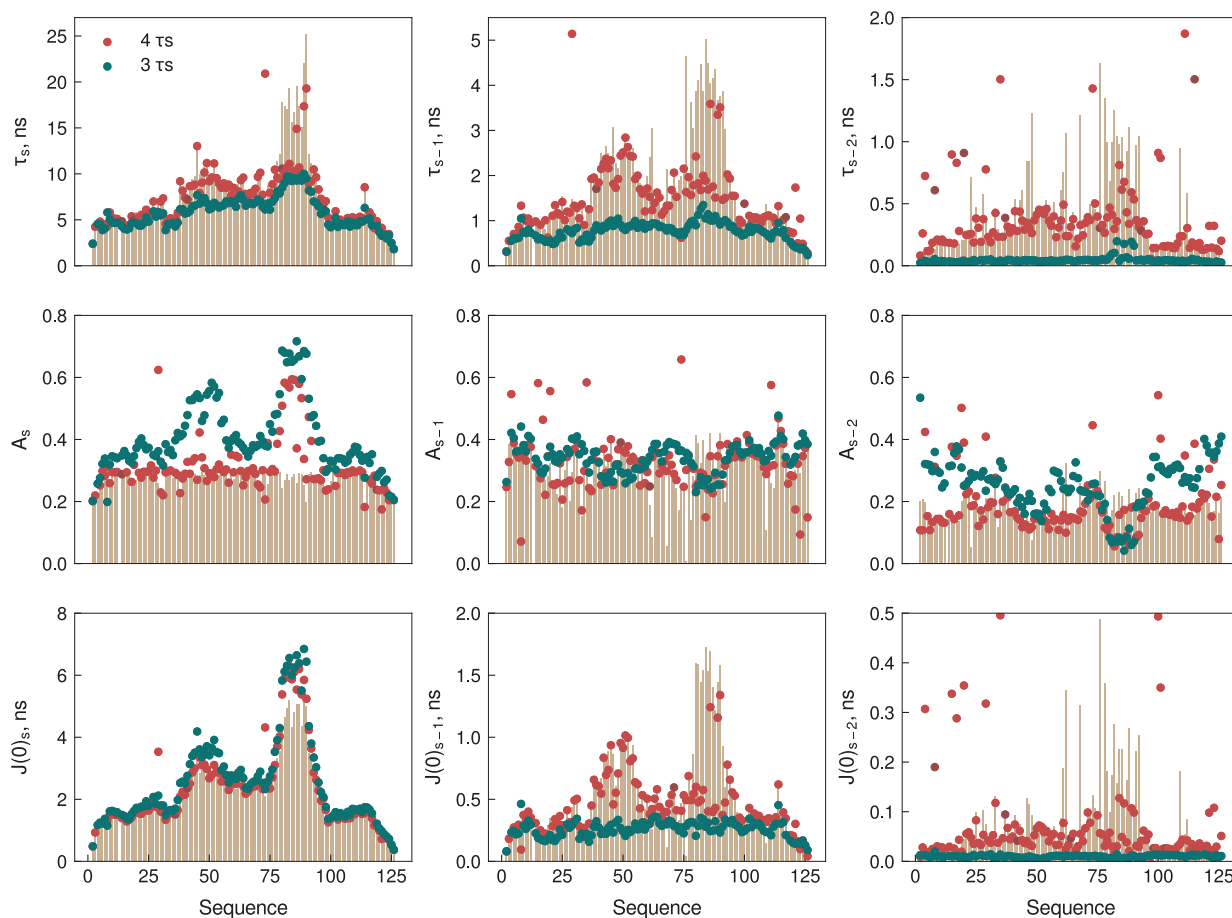
Figure 3.11: Comparison of dynamic modes for NTail (amplitudes and timescales of motions as well as their product - J(0) components, starting from the slowest one ( s ) obtained from the fit of average NH-backbone correlation function representing average over 54, 100 ns blocks of trajectories, and Model-Free analysis with three or four apparent dynamic modes of relaxation rates calculated on the basis of MD-derived NH-backbone dynamics with magnetic field strength ranging from 14.1 to 22.3T, at 298K.
