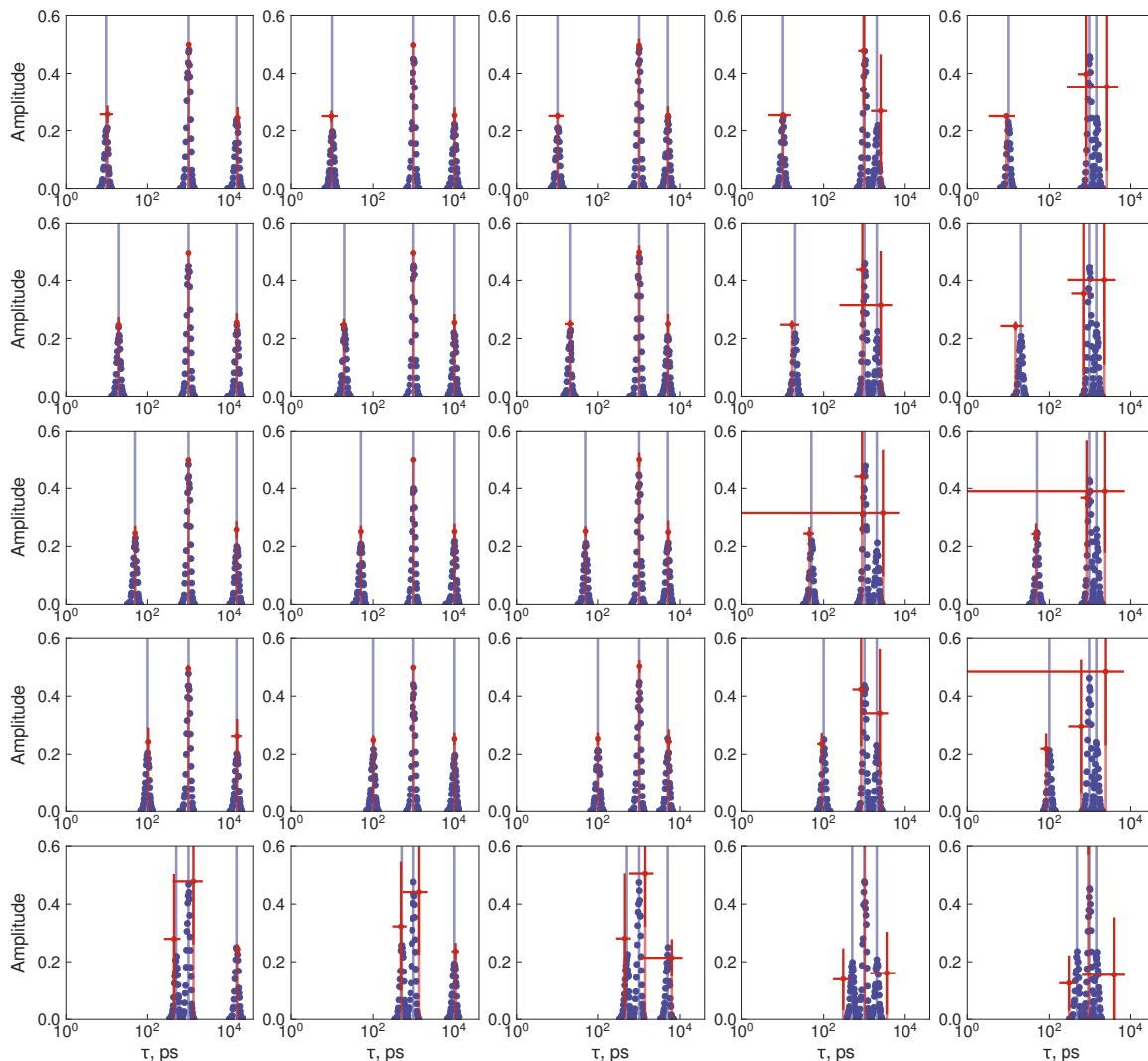
Figure App.3: Comparison of simulated distributions of correlation times used for calculation of relaxation rates with apparent dynamic modes estimated from Model-Free analysis of relaxation rates calculated on the basis of simulated correlation times (Population ratio: 1:2:1, \Omega = 0.1 ). Blue points represent distribution of simulated correlation times for each motion with average represented by blue bar. Orange points and bars represent average and standard deviation of estimated apparent dynamic modes on the basis of Model-Free analysis of relaxation rates calculated from simulated distributions of correlation times.
