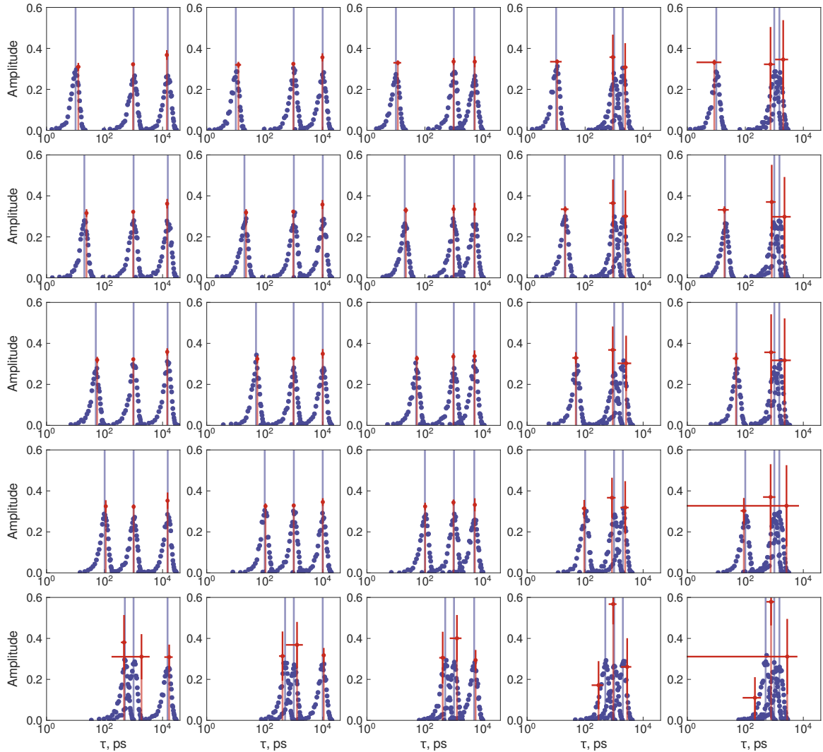
Figure App.4: Comparison of simulated distributions of correlation times used for calculation of relaxation rates with apparent dynamic modes estimated from Model-Free analysis of relaxation rates calculated on the basis of simulated correlation times (Population ratio: 1:1:1, \Omega = 0.3 ). Blue points represent distribution of simulated correlation times for each motion with average represented by blue bar. Orange points and bars represent average and standard deviation of estimated apparent dynamic modes on the basis of Model-Free analysis of relaxation rates calculated from simulated distributions of correlation times.
