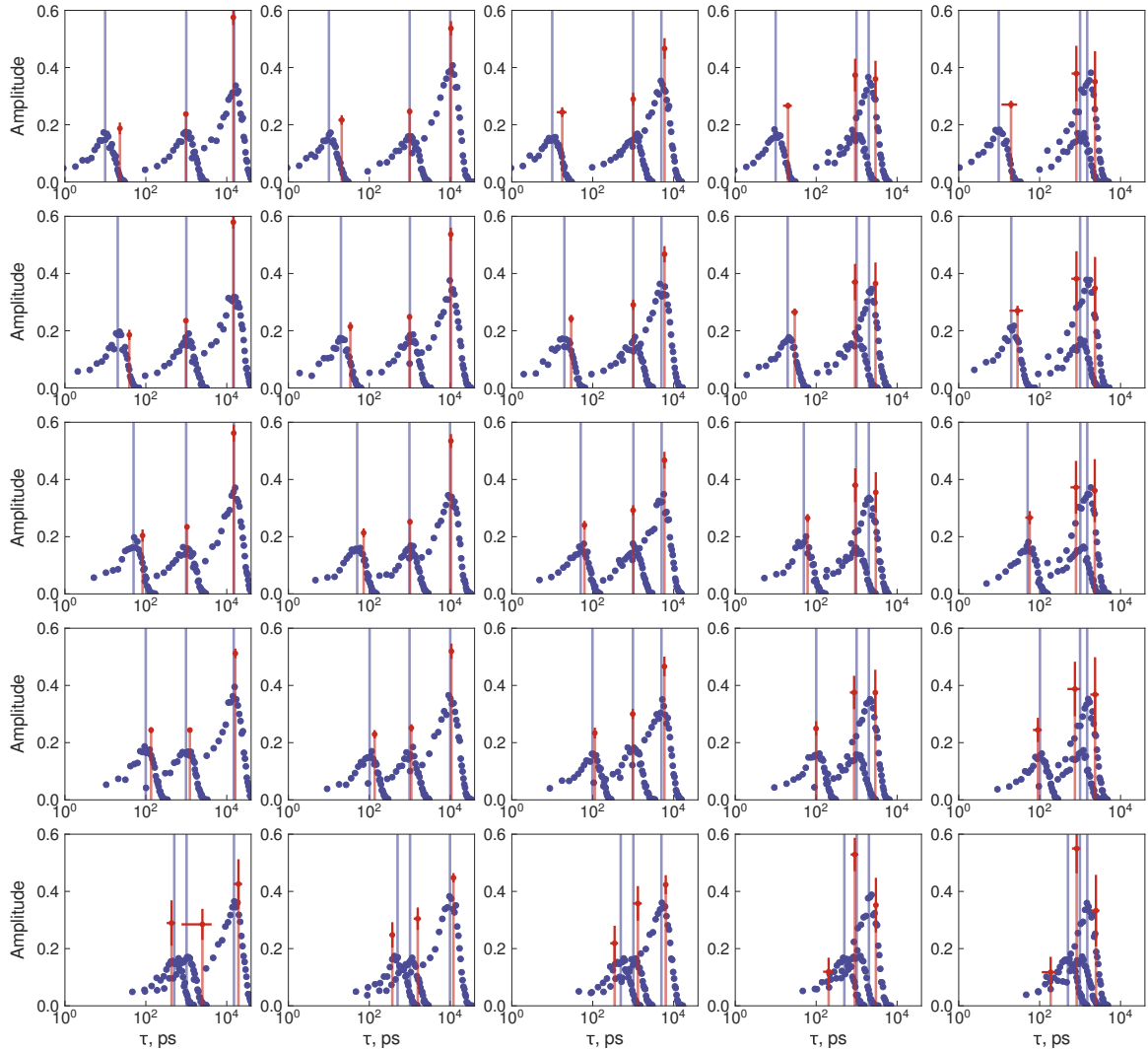
Figure App.8: Comparison of simulated distributions of correlation times used for calculation of relaxation rates with apparent dynamic modes estimated from Model-Free analysis of relaxation rates calculated on the basis of simulated correlation times (Population ratio: 1:1:2, \Omega = 0.6 ). Blue points represent distribution of simulated correlation times for each motion with average represented by blue bar. Orange points and bars represent average and standard deviation of estimated apparent dynamic modes on the basis of Model-Free analysis of relaxation rates calculated from simulated distributions of correlation times.
