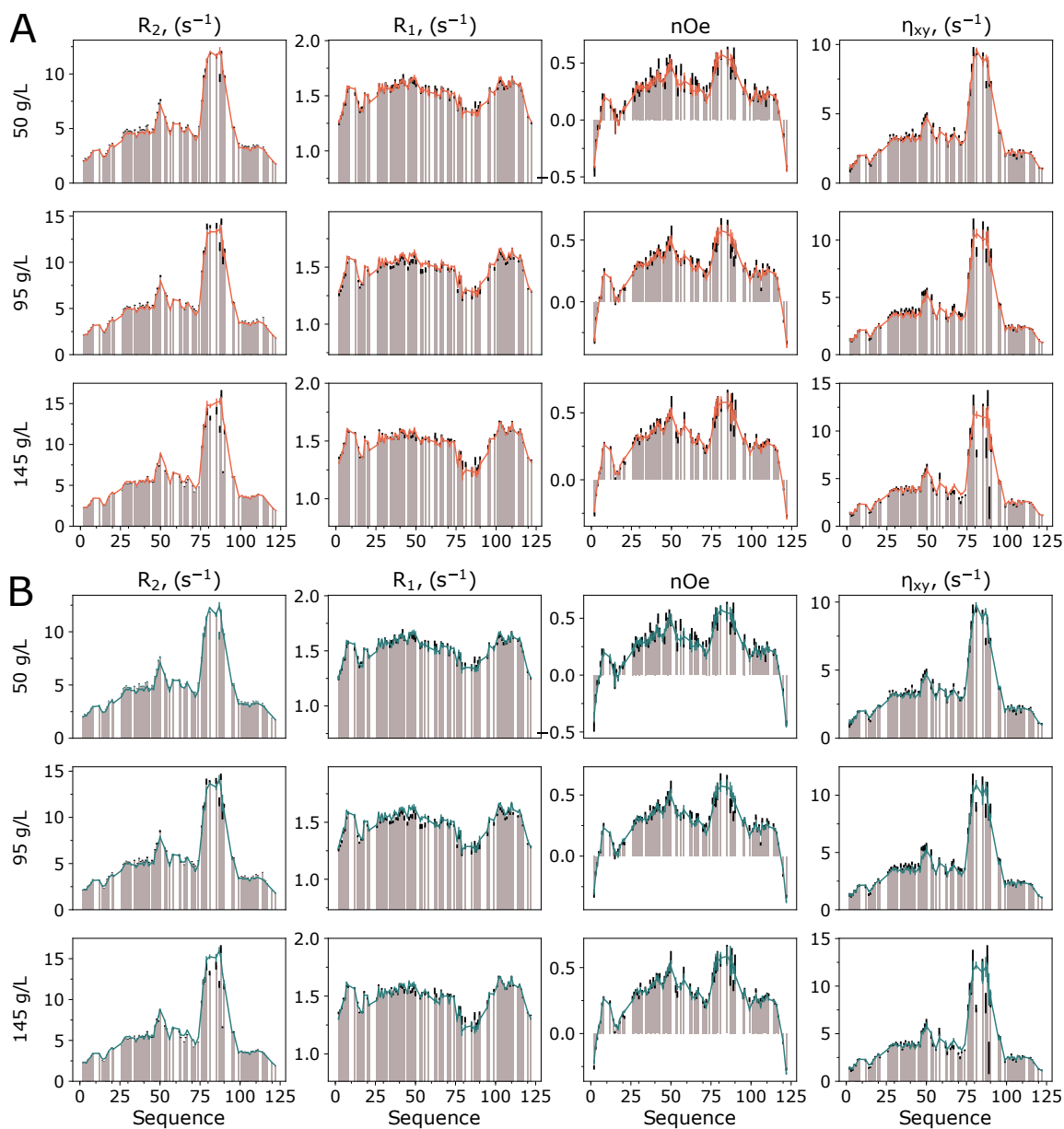
Figure 5.10: Comparison of active fit of ^{15}\text{N} backbone relaxation rates of NTail in admixtures with Dextran40 with concentrations ranging from 50 to 145 g/L at 288K (A) with prediction of the same relaxation rates from analysis of data composed of relaxation rates at dilute conditions (0 g/L) at four temperatures, and in admixtures with Dextran40 concentrations ranging from 50 to 195 g/L at 298K (B). Bars represent experimental values, red and green lines mark calculated values from active fit and prediction respectively.
