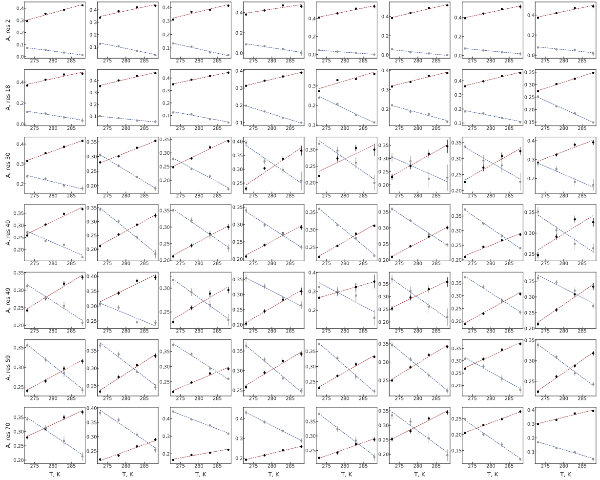
Figure 4.8: Temperature dependence of amplitudes of motion of MKK4. Black and grey points denote values derived from Arrhenius Model-Free analysis of MKK4, brown and blue lines represent fit to two parameter linear equation for fast and slow motions respectively. The fits have been performed in temperature range of 273 to 288K.
