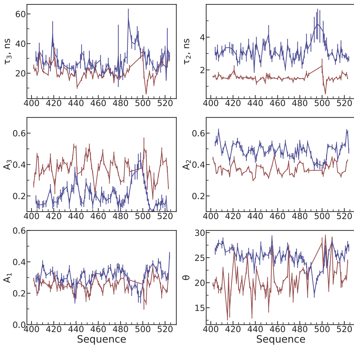
Figure 6.8: Comparison of the dynamic modes estimated using 5 parameter Model-Free analysis of relaxation rates in concentrated phase assuming constant value of fast timescales of motions equal to 50 ps (two amplitudes, two timescales and CSA-DD angle, red) with prediction from the combined Einstein-Arrhenius Model Free analysis and \rho = 3.44 from longitudinal relaxation rate of water molecules in the concentrated phase (blue).
