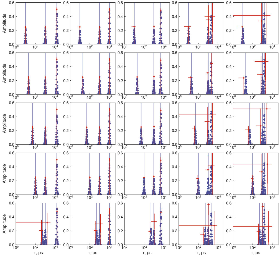
Figure App.2: Comparison of simulated distributions of correlation times used for calculation of relaxation rates with apparent dynamic modes estimated from Model-Free analysis of relaxation rates calculated on the basis of simulated correlation times (Population ratio: 1:1:2, \Omega = 0.1 ). Blue points represent distribution of simulated correlation times for each motion with average represented by blue bar. Orange points and bars represent average and standard deviation of estimated apparent dynamic modes on the basis of Model-Free analysis of relaxation rates calculated from simulated distributions of correlation times.
