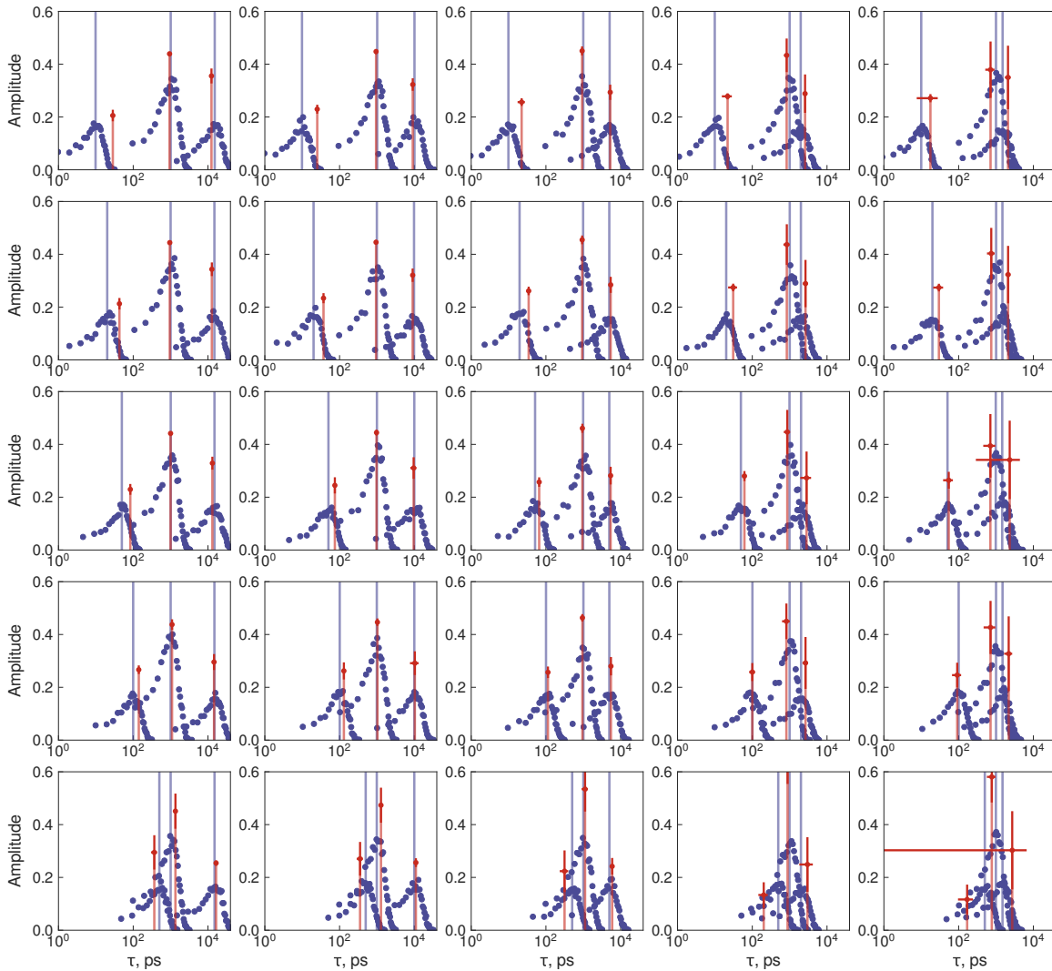
Figure App.9: Comparison of simulated distributions of correlation times used for calculation of relaxation rates with apparent dynamic modes estimated from Model-Free analysis of relaxation rates calculated on the basis of simulated correlation times (Population ratio: 1:2:1, \Omega = 0.6 ). Blue points show simulated values classified in 33 bins for each dynamic mode with average value represented by blue bar. Orange points and bars show average and standard deviation of estimated apparent dynamic modes on the basis of Model-Free analysis of relaxation rates calculated from simulated distributions of correlation times.
