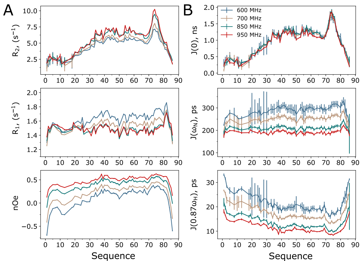
Figure 3.8: Residue resolved ^{15}\text{N} backbone relaxation rates of MKK4 at 273K (A) and associated with it SDF values estimated from RSDM (B) at frequencies associated with spin interactions (B).
