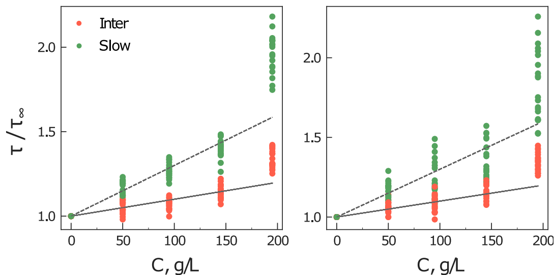
Figure 5.5: Comparison of relative changes of backbone amide correlation times as a function of viscogen concentration with changes in solvent reorientation rate for a few chosen residues within the range 20-40 and 100-120: solid line \rho+1 , dotted line: 3\rho(C)+1 .
