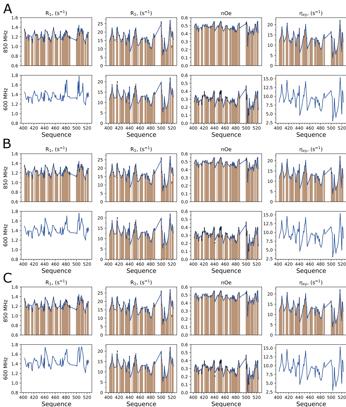
Figure App.14: Best-fit values of independent Model-Free analysis of ^{15}\text{N} -backbone relaxation of C-terminal part of Measles Nucleoprotein in the concentrated phase using Model 3, optimizing two timescales, two amplitudes and CSA-DD angle, assuming constant average value of timescales of fast motions equal to 50, 75 or 100 ps (panels A, B and C respectively).
