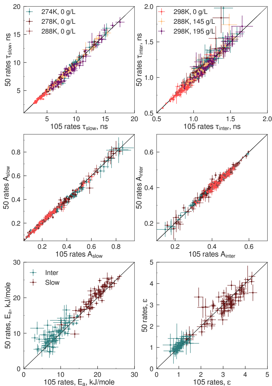
Figure 5.11: Accuracy of determination of apparent dynamic modes and site and mode-specific energies of activation ( E_a ) and friction coefficients ( \epsilon_i ) with less than half of the dataset: relaxation rates at infinite dilution at four temperatures, relaxation rates at 145 and 195 g/L of Dextran40 at 298K. In all cases only data at two magnetic fields was used (600 and 850 MHz).
