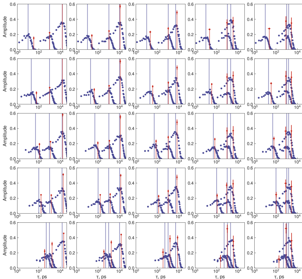
Figure App.11: Comparison of simulated values of dynamic modes used for calculation of relaxation rates with values estimated from Model-Free analysis of relaxation rates calculated on the basis of simulated ones (Population ratio: 1:1:2, \Omega = 0.9 ). Blue points represent distribution of simulated correlation times for each motion with average represented by blue bar. Orange points and bars represent average and standard deviation of estimated apparent dynamic modes on the basis of Model-Free analysis of relaxation rates calculated from simulated distributions of correlation times.
