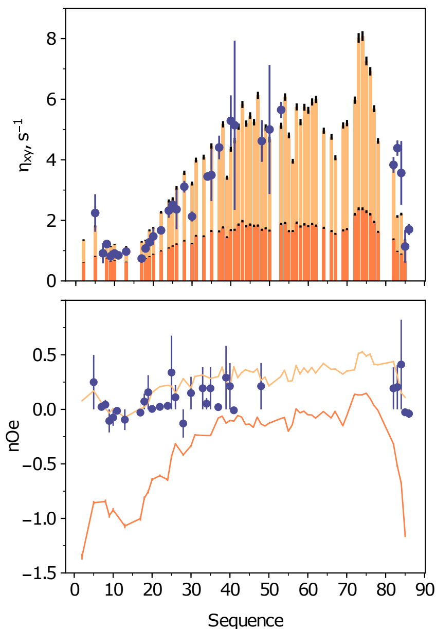
Figure 6.5: Comparison of experimental relaxation rates ( \eta_{xy} and heteronuclear nOe at 700 and 600 MHz respectively) at 292K acquired in oocytes (blue) with prediction at infinite dilution ( \rho = 0.0 , dark orange) and nanoscale viscosity according to the values of R_{1,water} ( \rho = 1.00 , pale orange). Experimental values of \eta_{xy} show average and standard deviation of two biological replica, heteronuclear nOe shows boot-strap average and standard deviation for single biological replica. For prediction of relaxation rates from simultaneous viscosity and temperature-dependent Model-Free analysis, amplitudes were obtained by linear extrapolation to 292K, while timescales of apparent dynamic modes were obtained using Einstein-Arrhenius relationship and value of relative solvent viscosity (defined by \rho ) at given temperature.
