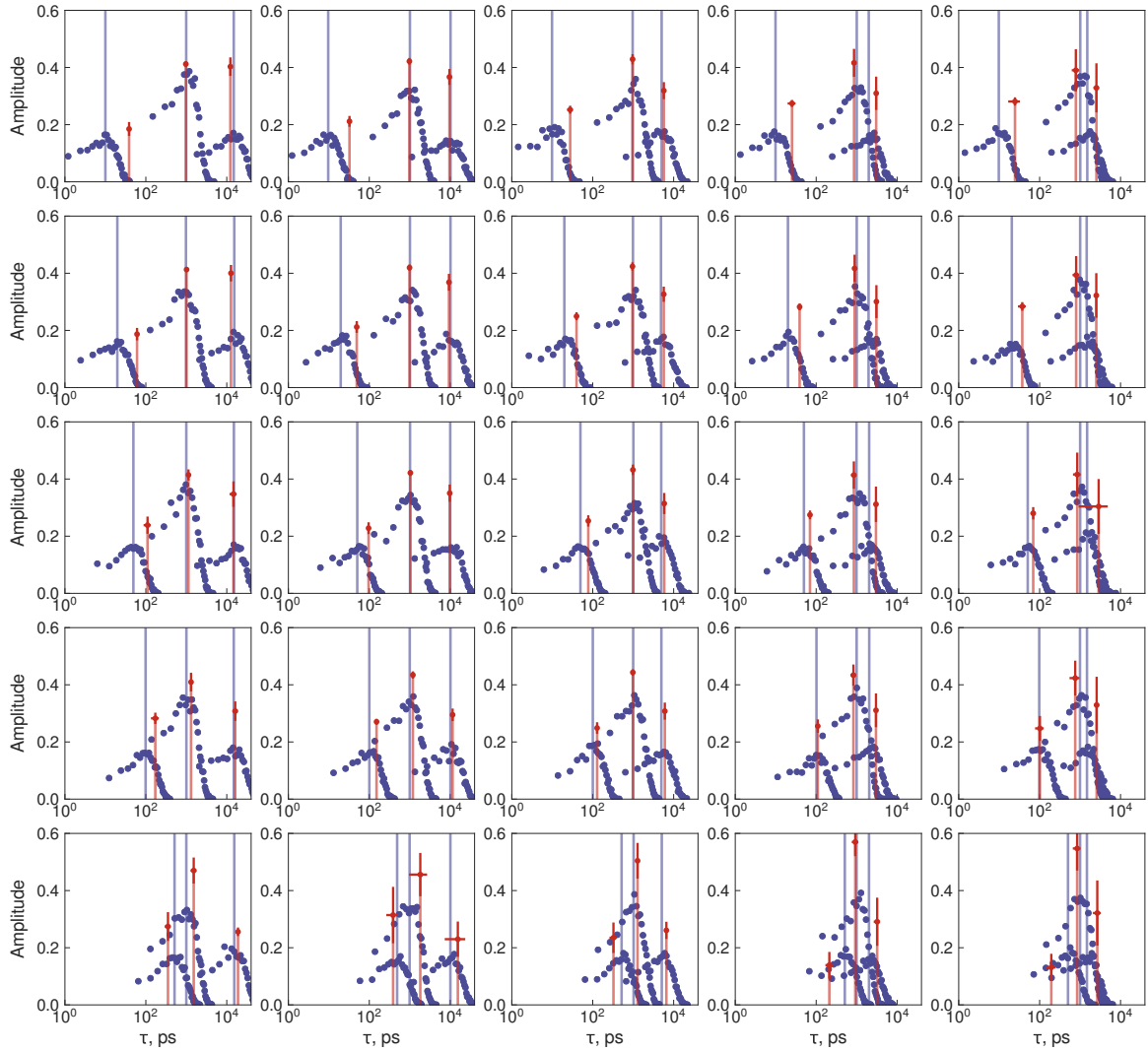
Figure App.12: Comparison of simulated distributions of correlation times used for calculation of relaxation rates with apparent dynamic modes estimated from Model-Free analysis of relaxation rates calculated on the basis of simulated correlation times (Population ratio: 1:2:1, \Omega = 0.9 ). Blue points represent distribution of simulated correlation times for each motion with average represented by blue bar. Orange points and bars represent average and standard deviation of estimated apparent dynamic modes on the basis of Model-Free analysis of relaxation rates calculated from simulated distributions of correlation times.
