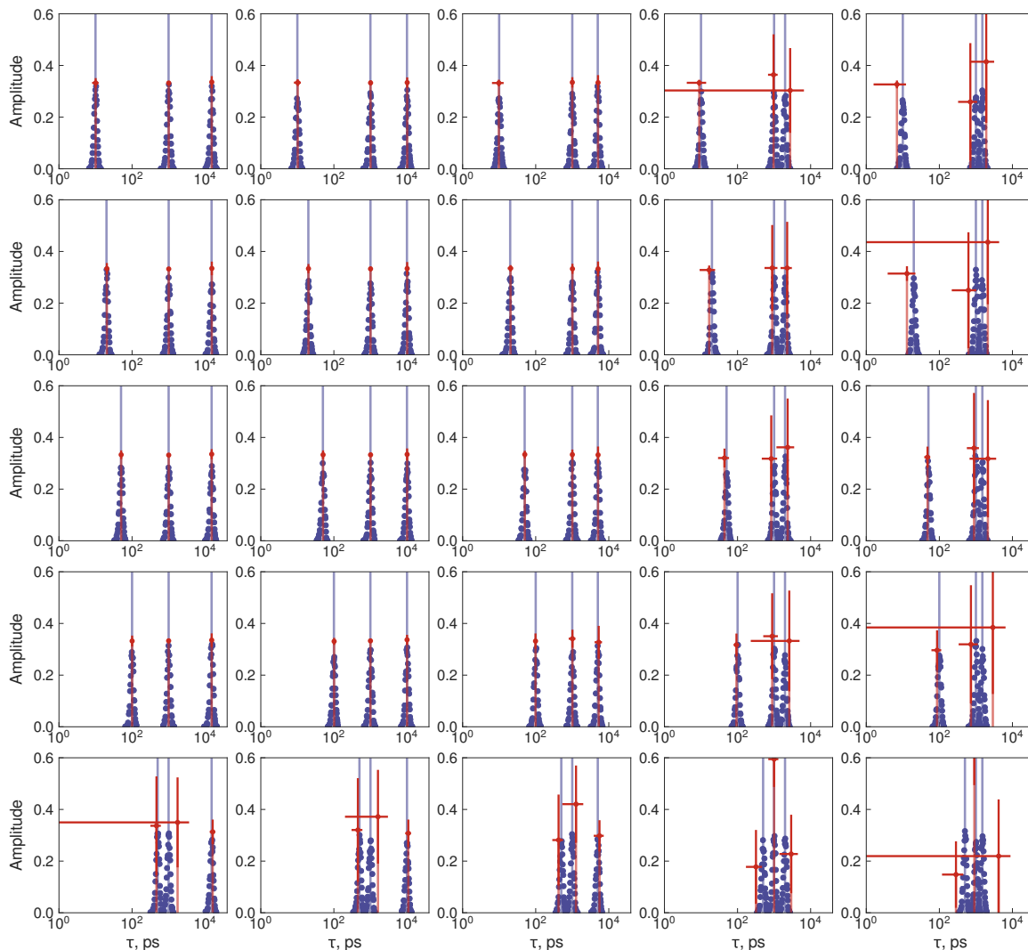
Figure App.1: Comparison of simulated distributions of correlation times used for calculation of relaxation rates with apparent dynamic modes estimated from Model-Free analysis of relaxation rates calculated on the basis of simulated correlation times (Population ratio: 1:1:1, \Omega = 0.1 ). Blue points represent distribution of simulated correlation times for each motion with average represented by blue bar. Orange points and bars represent average and standard deviation of estimated apparent dynamic modes on the basis of Model-Free analysis of relaxation rates calculated from simulated distributions of correlation times.
