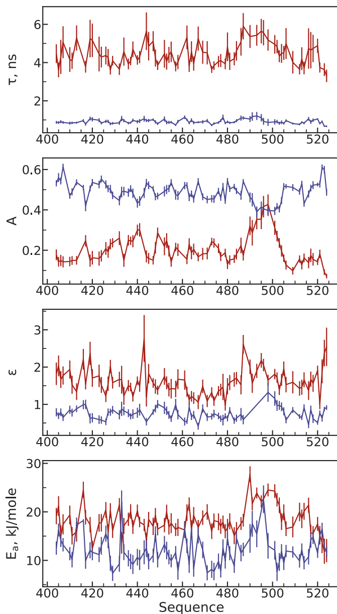
Figure 6.7: Result of the combined Einstein-Arrhenius type Model Free analysis of ^{15}\text{N} backbone relaxation rates of Measles NTail using Model 3 with equation 5.4 as described previously. The spin relaxation rates as a function of temperature and viscosity are represented by site-specific activation energies ( E_{a,i} ) and friction coefficients ( \epsilon_i ), as well as, amplitudes and timescales of motions ( A_i and \tau_i ) at 298K and at infinite temperature and dilution respectively for slow and intermediate motions. Values of the apparent fast dynamic mode have been constrained to 50 ps, while the amplitudes of fast motions have been estimated from the normalization condition of amplitudes of motions. Red and blue mark values of slow and intermediate modes respectively.
