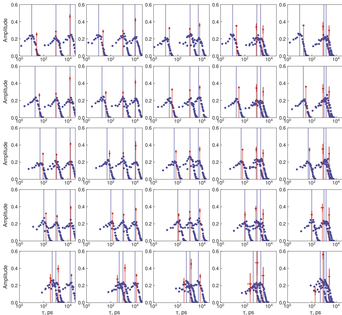
Figure App.10: Comparison of simulated distributions of correlation times used for calculation of relaxation rates with apparent dynamic modes estimated from Model-Free analysis of relaxation rates calculated on the basis of simulated correlation times (Population ratio: 1:1:1, \Omega = 0.9 ). Blue points show distribution of simulated correlation times for each motion with average represented by blue bar. Orange points and bars show average and standard deviation of calculated apparent dynamic modes from Model-Free analysis of relaxation rates calculated on the basis of simulated distribution of timescales and amplitudes of motion.
