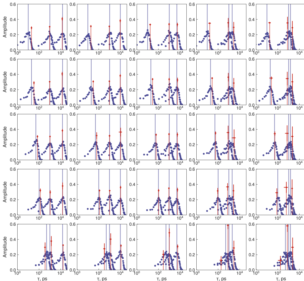
Figure App.7: Comparison of simulated distributions of correlation times used for calculation of relaxation rates with apparent dynamic modes estimated from Model-Free analysis of relaxation rates calculated on the basis of simulated correlation times (Population ratio: 1:1:1, \Omega = 0.6 ). Blue points represent distribution of simulated correlation times for each motion with average represented by blue bar. Orange points and bars represent average and standard deviation of estimated apparent dynamic modes on the basis of Model-Free analysis of relaxation rates calculated from simulated distributions of correlation times.
