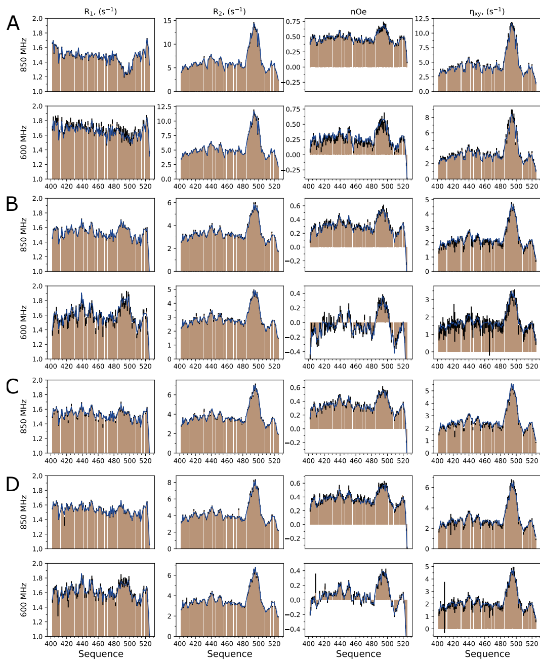
Figure App.13: Best-fit values of the combined Einstein-Arrhenius Model-Free analysis of ^{15}\text{N} -backbone relaxation of C-terminal part of Measles Nucleoprotein using Model 3 with equation 5.4. Panels A-D show experimental (bars) and calculated (line) values of relaxation rates at 278K, 0 g/L, 298K 0, 37.5 and 75 g/L.
