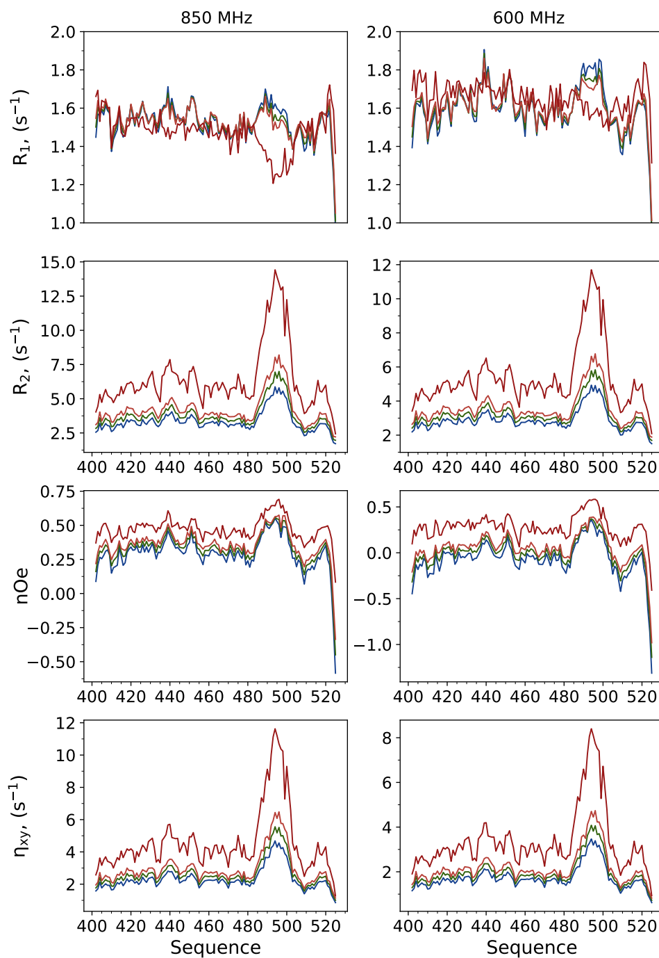
Figure 6.6: ^{15}\text{N} backbone relaxation rates of NTail measured in the range of admixtures with Dextran40 0 (blue), 37.5 (green), 75 g/L (orange) at 298K and 0 g/L (red) at 278K and two magnetic fields strengths - 14.1 and 20.0T.
