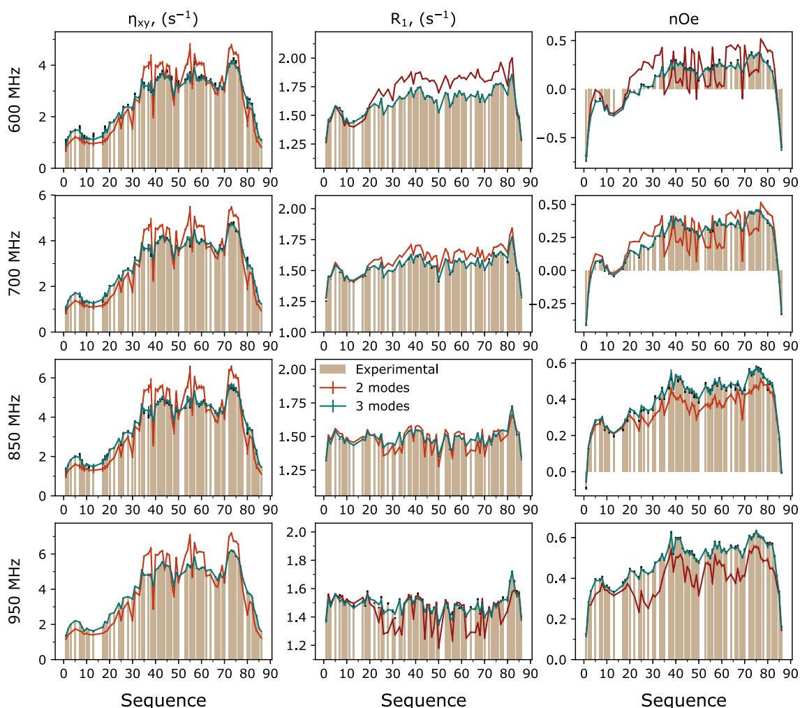
Figure 3.9: Reproduction of the experimental data (bars) using Model-Free analysis assuming two (orange) or three (green) statistically independent, timescale separated reorientation processes.
