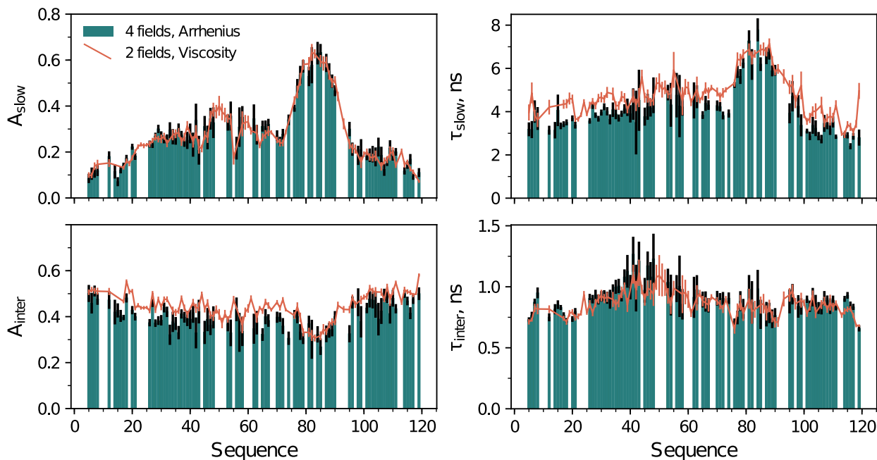
Figure 5.7: Comparison of apparent dynamic modes and associated amplitudes obtained from Einstein (viscosity-dependent) and Arrhenius (temperature-dependent) analysis at 298K and 0 g/L.
