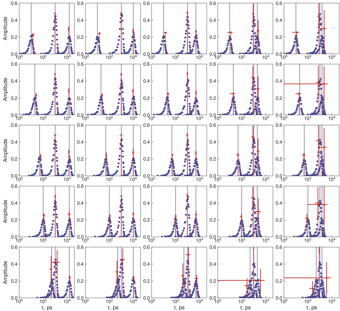
Figure App.6: Comparison of simulated distributions of correlation times used for calculation of relaxation rates with apparent dynamic modes estimated from Model-Free analysis of relaxation rates calculated on the basis of simulated correlation times (Population ratio: 1:2:1, \Omega = 0.3 ). Blue points represent distribution of simulated correlation times for each motion with average represented by blue bar. Orange points and bars represent average and standard deviation of estimated apparent dynamic modes on the basis of Model-Free analysis of relaxation rates calculated from simulated distributions of correlation times.
