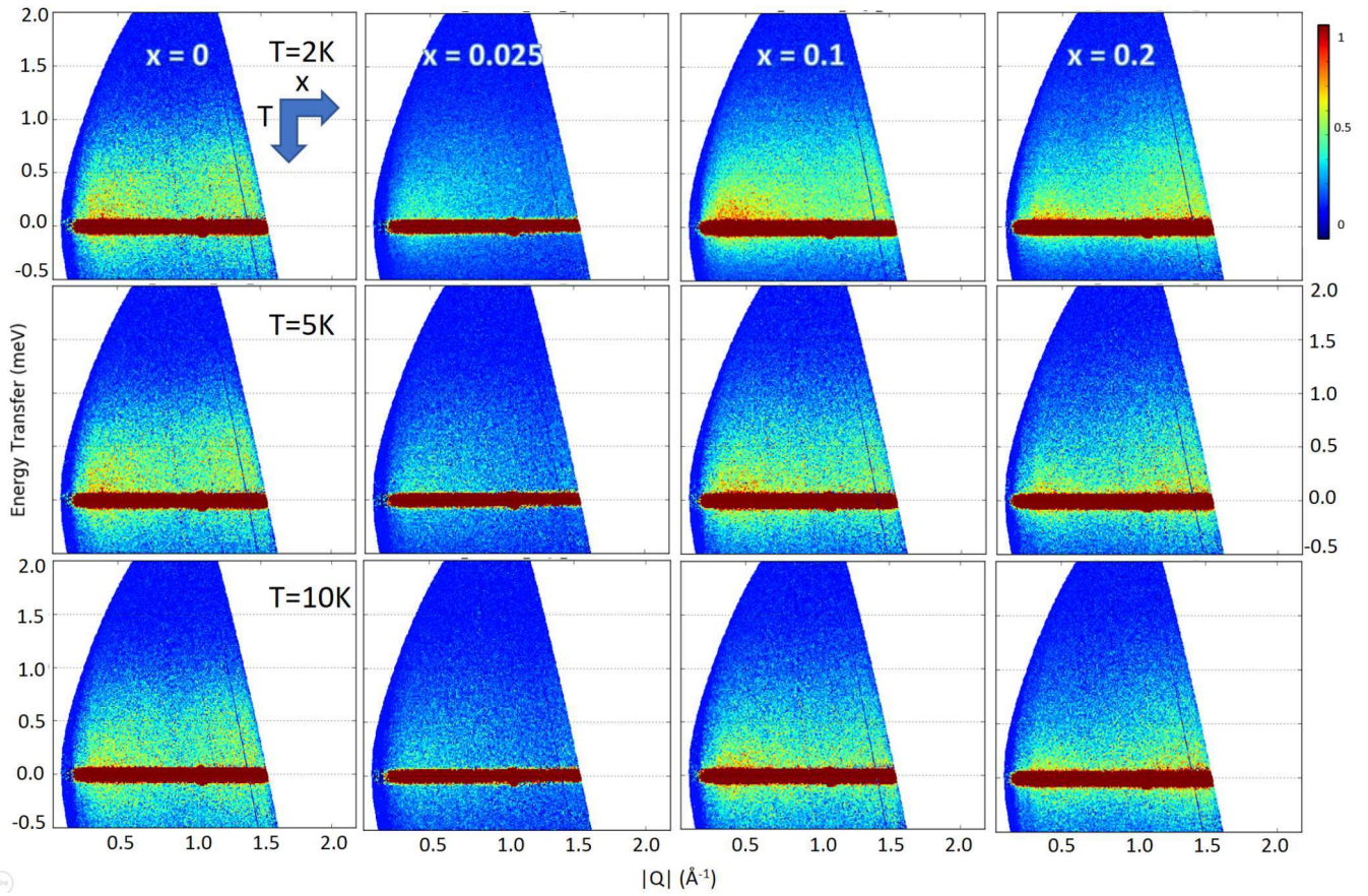
Figure 8.4: S(Q, \omega) intensity maps at T = 2\text{K} , 5\text{K} and 10\text{K} with E_i = 2.5\text{meV} , under zero applied field for \text{Yb}_2\text{Ti}_{2(1-x)}\text{Zr}_{2x}\text{O}_7 , with x = 0, 0.025, 0.1, 0.2 . S(Q, \omega) intensity is normalized to the number of incident neutrons and a common scale is used for clarity of comparison. Note that the sample mass is not the same for different x , in particular for the x=0.025 and x=0.1 samples. The overall intensity of the x=0.025 measurement is weaker due to the reduced scattering cross section because of a lower mass. (see Tab.8.1)
