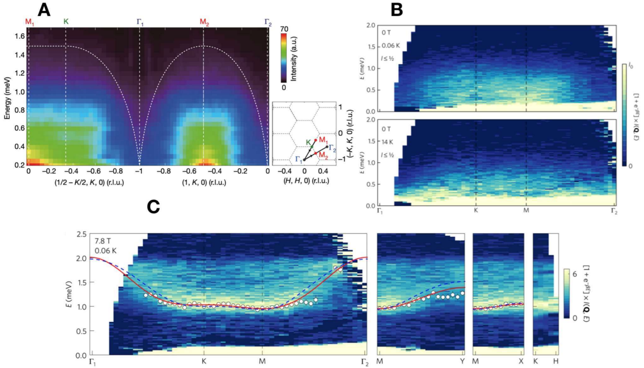
Figure 3.6: A. INS intensity plots [55] on \text{YbMgGaO}_4 . The plot shows a broad continuum of the intensity along the M - K - \Gamma - M - \Gamma directions. The contour direction is shown by the black lines in the subplot. B In the INS experiment [55] on \text{YbMgGaO}_4 , at T = 60\text{mK} and 14\text{K} , a continuum of scattering intensity is observed along the high symmetry direction in reciprocal space. The red and blue lines show a fit to the spin-wave dispersion relation. C. The continuum of excitation persists at 60\text{mK} in the presence of an applied field of 7.8\text{T} .
