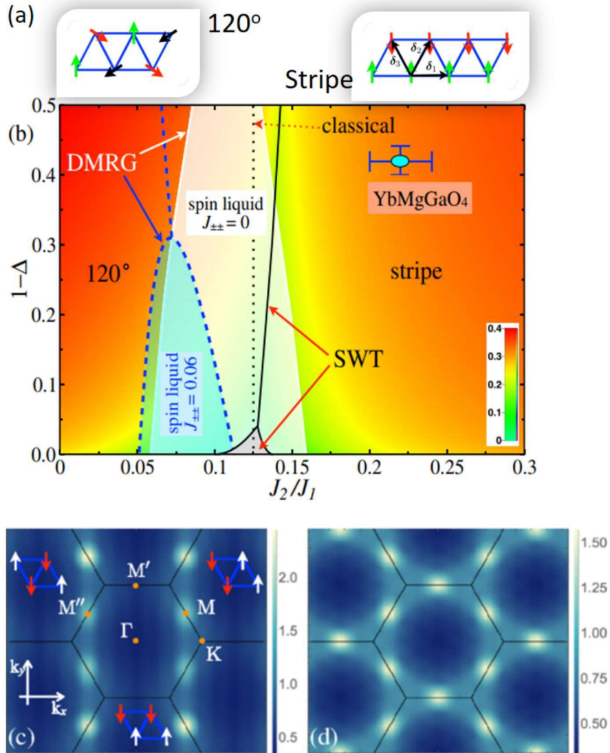
Figure 4.11: Phase diagram of a 2D THAF as estimated by Zhu et al.[47]. The top panel (a), shows the 2 ordered phases of the triangular lattice, the striped and the the 120° ordered phase. In (b) \Delta is the anisotropy( \Delta = 2J_{zz}/(J_{xx} + J_{yy}) ) and J_1, J_2 are the parameters of the XXZ component of the spin Hamiltonian indicating the first and second nearest neighbor exchanges, (c) is the DMRG simulated structure factor with \Delta = 0.56 , and (d) is the symmetry averaged structure factor replicating the INS spectrum of YbMgGaO 4
