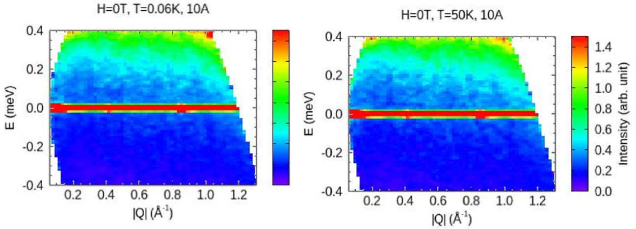
Figure 6.6: S(Q, \omega) scans under zero applied field at 60mK and 50K.
