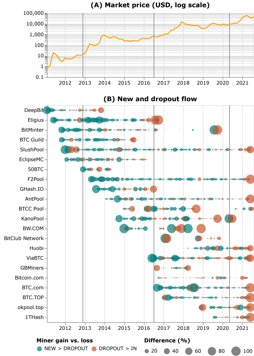
Figure 28: New and dropout flow. (A) The line chart displays the market price of Bitcoin in US Dollar on the log scale. (B) The size of the circle represents the absolute difference between new and dropout miners. New miners' positive (or negative) flow is encoded with the green (or red) color.
