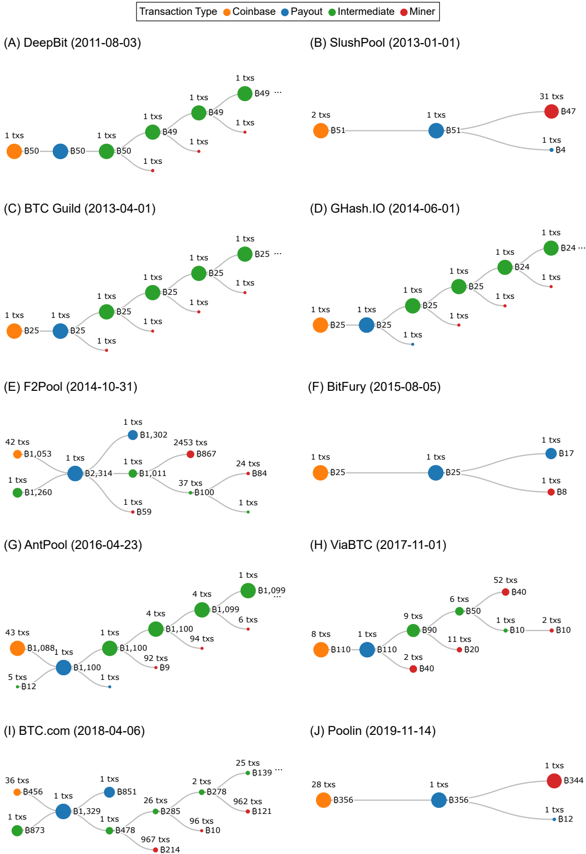
Figure 24: Reward payout flow patterns extracted from the top 10 mining pools in this study. Each node represents a transaction type with branches of similar patterns grouped together. The color of the node indicates the transaction type. The total value of transactions in each node is encoded by circle size in proportion to the tx_{payout} value.
