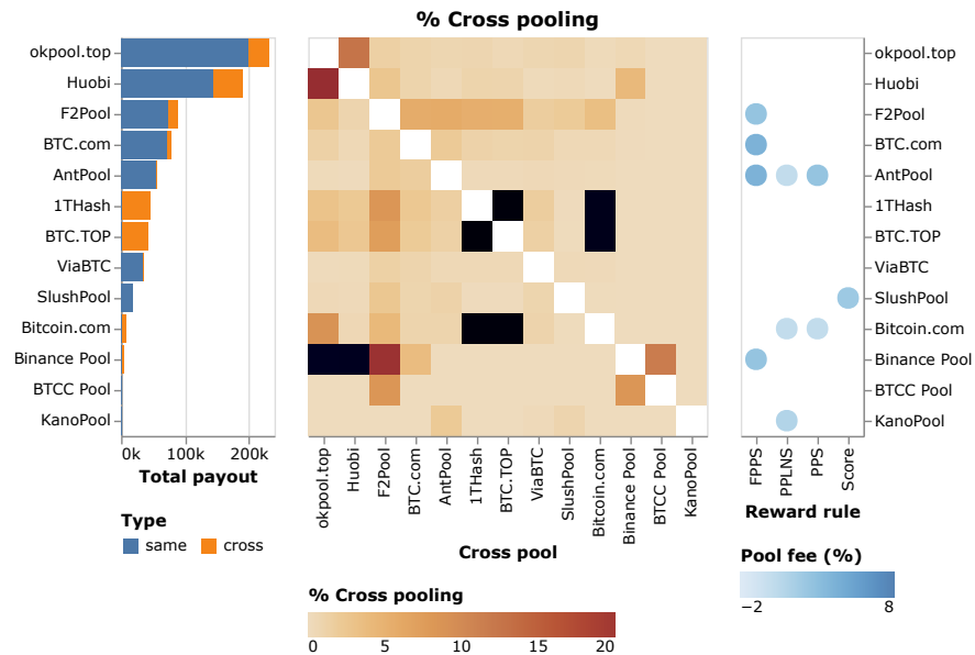
Figure 36: The compound chart displays the total payout (left), reward payout scheme (right), and cross-pooling between mining pools (middle) between January 2020 and December 2020.
