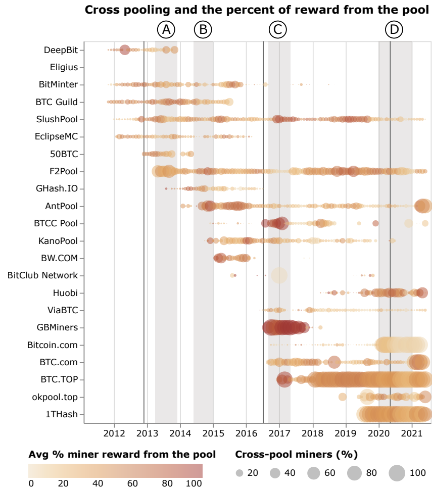
Figure 31: Cross pooling flow. The size of the circle corresponds to the percentage of cross-pooling of all miners in a given month. The percentage of reward that cross-pooling miners obtained from the pool is encoded using a brown color scale. Four periods with a high cross-pooling are highlighted in the grey background: (A) April 2013 – November 2013, (B) June 2014 – December 2014, (C) September 2016 – April 2017, and (D) January 2020 – December 2020.
