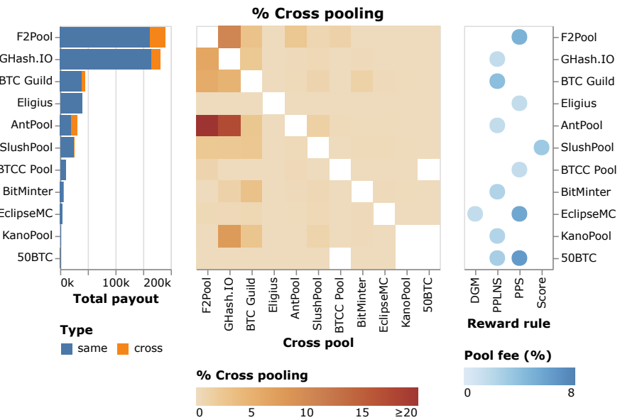
Figure 33: The compound chart displays the total payout (left), reward pay-out scheme (right), and cross-pooling between mining pools (middle) between June 2014 and December 2014.
