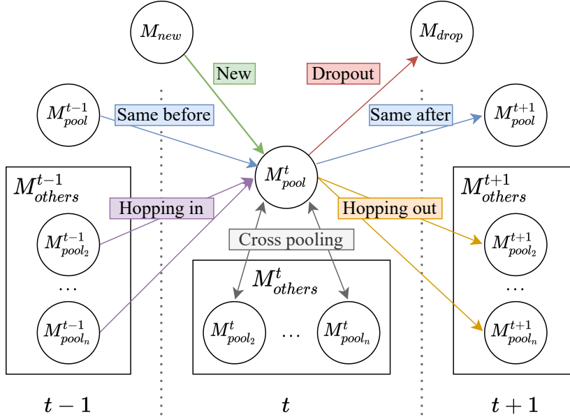
Figure 25: The miners' migration flow model of pool at time interval t . t-1 ( t+1 ) is the time interval before (resp. after) t . M_{new} ( M_{drop} ) is the list of miners not in any pool at t-1 (resp. is not found in any mining pool at t+1 ). The union of the list of miners from other pools is M_{others} .
