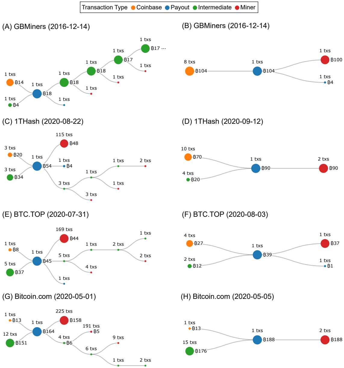
Figure 35: Reward payout flow patterns of mining pools that has high cross-pooling miners: (A–B) GBMiners, (C–D) 1THash, (E–F) BTC.TOP, and (G–H) Bitcoin.com. I detected that these mining pools has two payout flow patterns: (Left) mining pools pay reward directly to miners; (Right) mining pools forward the reward to their own addresses.
