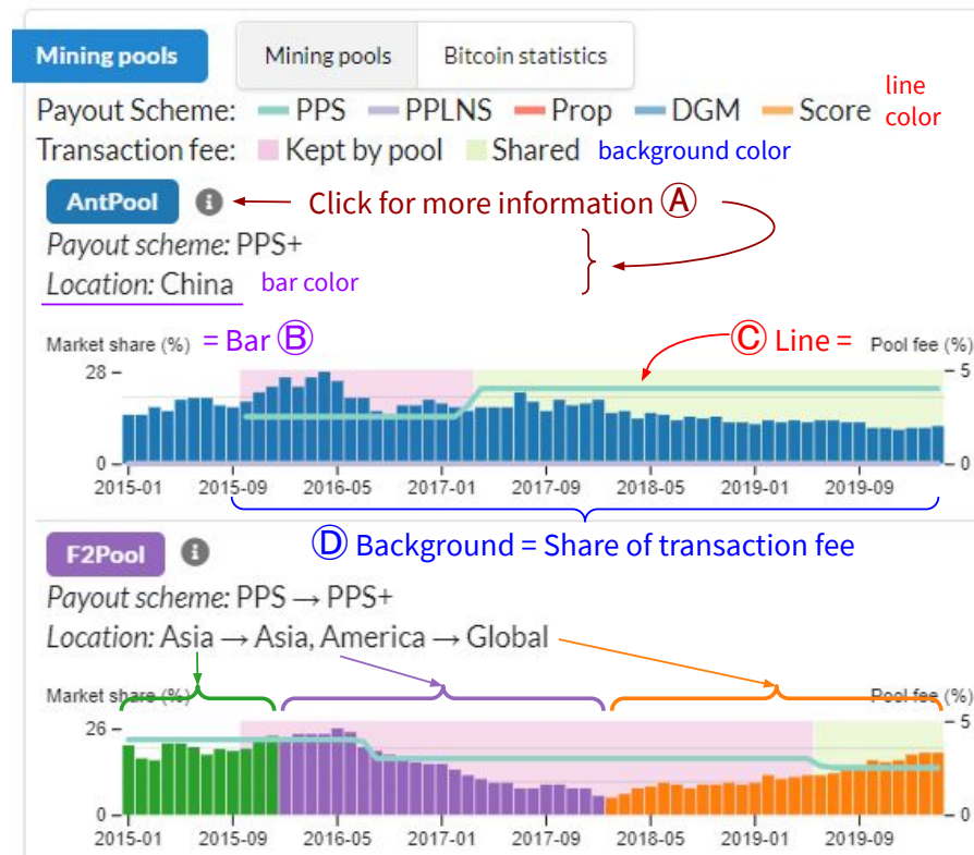
Figure 39: The mining pool details view (V3) shows the details of each mining pool as a dual-axis chart. The measure on the left y-axis and the bar color are selected from V2: Measure: Market share (%) and Color by: Location , respectively.
