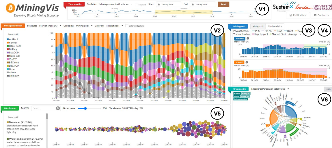
Figure 37: The MiningVis tool consists of six coordinated views: (V1) the time filter view, (V2) the mining distribution view, (V3) the mining pool details view, (V4) the Bitcoin statistics view (toggle with V3, see Figure 41), (V5) the Bitcoin news view, and (V6) the cross pooling view.
