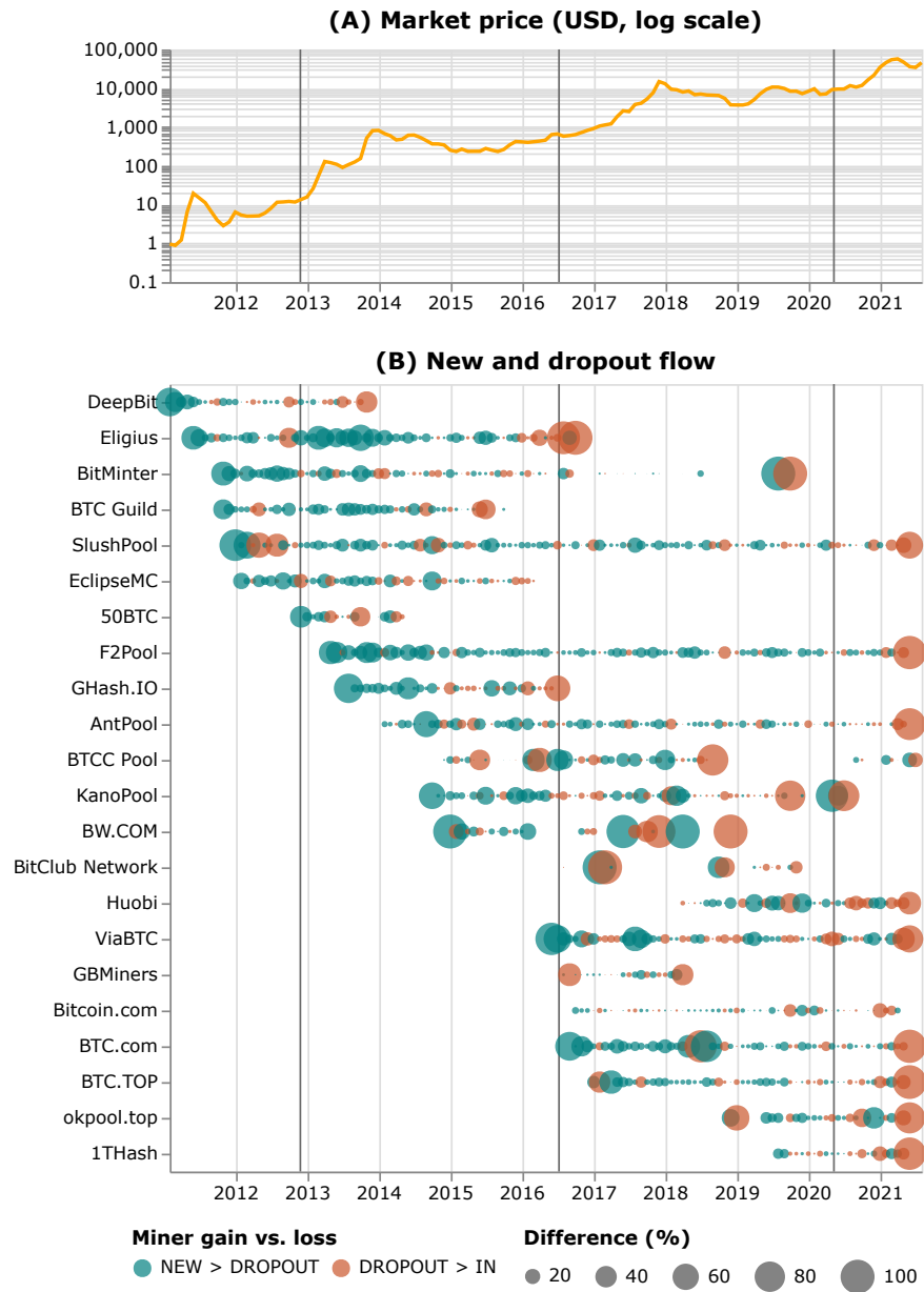
Figure 28: New and dropout flow. (A) The line chart displays the market price of Bitcoin in US Dollar on the log scale. (B)The size of the circle represents the absolute difference between new and dropout miners. New miners’ positive (or negative) flow is encoded with the green (or red) color.
