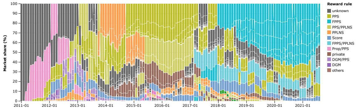
Figure 21: The market share distribution according to payout schemes.
