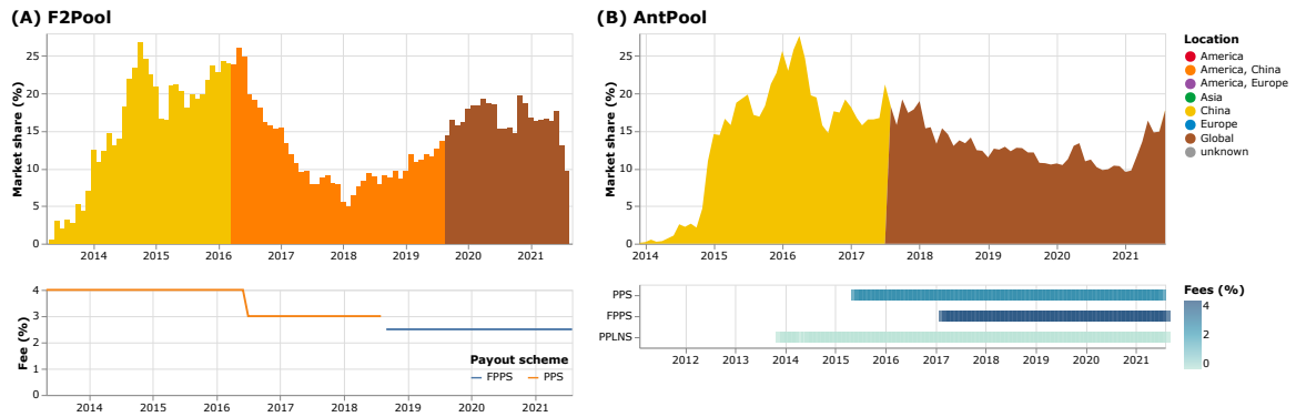
Figure 40: Design alternatives for the mining pool details view: (A) F2Pool—The bar chart displays market share, and the line chart below shows pool fees; (B) AntPool—The area chart displays market share, and the heat map below encodes pool fees for each payout scheme.
