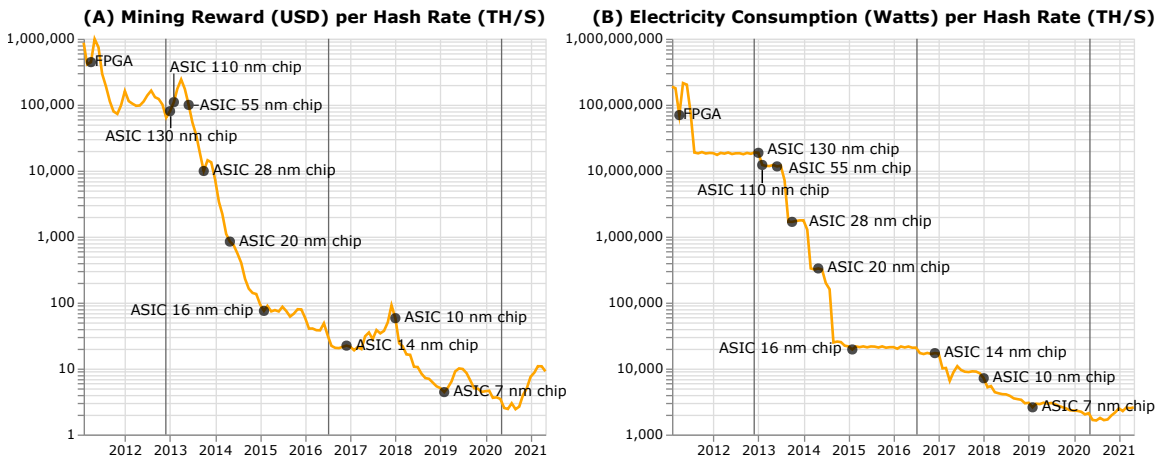
Figure 23: (A) Mining revenue in US Dollars per hash rate (TH/s). (B) Electricity consumption in Watts per hash rate (TH/s). I annotated new mining technology evolution as a dot on the charts.
