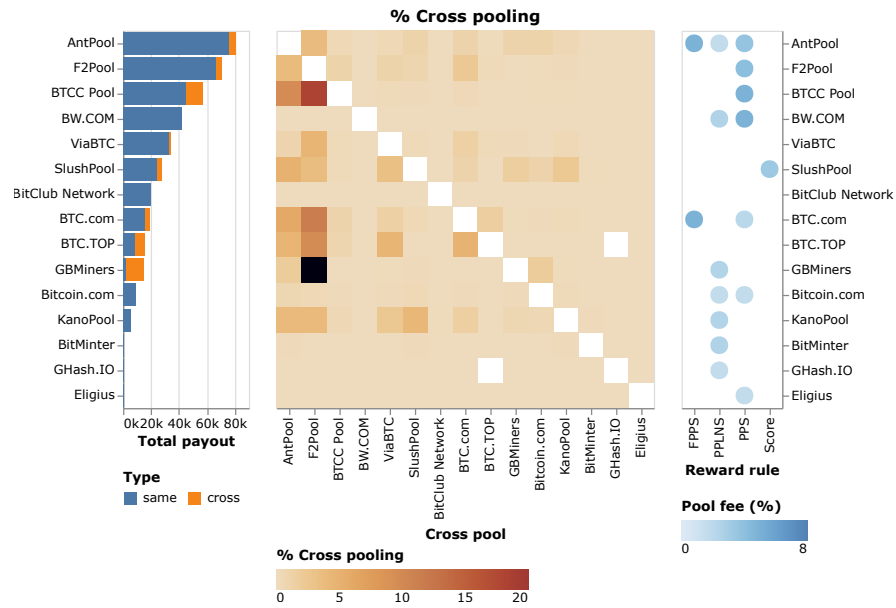
Figure 34: The compound chart displays the total payout (left), reward payout scheme (right), and cross-pooling between mining pools (middle) between September 2016 and April 2017.
