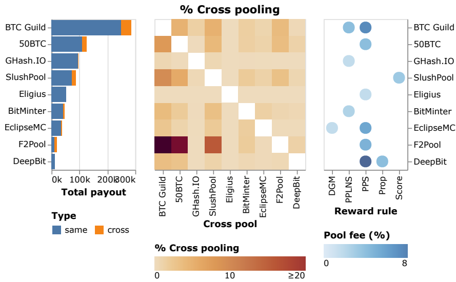
Figure 32: The compound chart displays the total payout (left), reward pay-out scheme (right), and cross-pooling between mining pools (middle) between April 2013 and November 2013.
