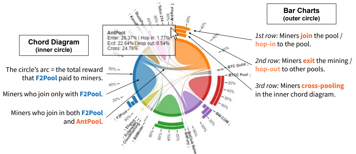
Figure 44: The miners' migration flows are represented as a chord diagram to visualize the amount of cross-pool miners between pools. For each pool, the bar chart displays the percentage of new, pool hopping, cross pooling, and dropout miners.
