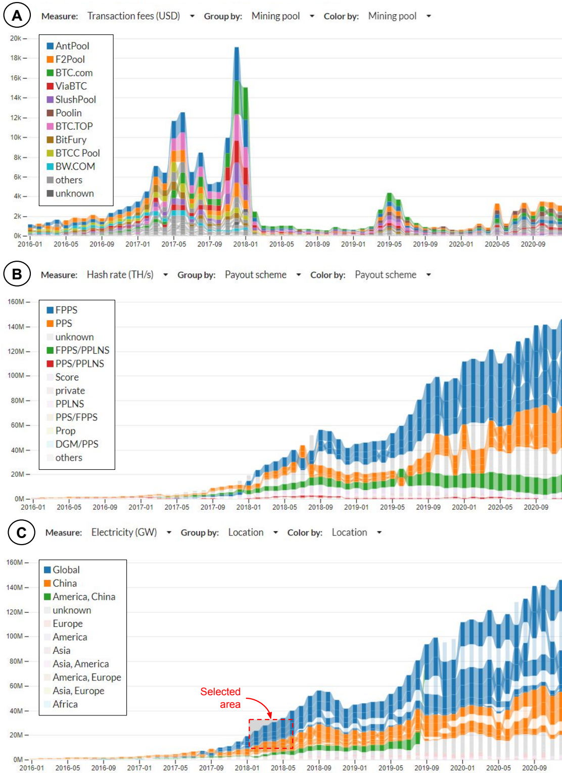
Figure 38: The mining pool distribution view (V2) with different configurations. (A) Measure: Transaction fees (USD), Group by Mining pool, and Color by: Mining pool. (B) Measure: Hash rate (TH/s), Group by: Payout scheme, and Color by: Payout scheme with label selection. (C) Measure: Electricity (GW), Group by: Location, Color by: Location with brush selection.
