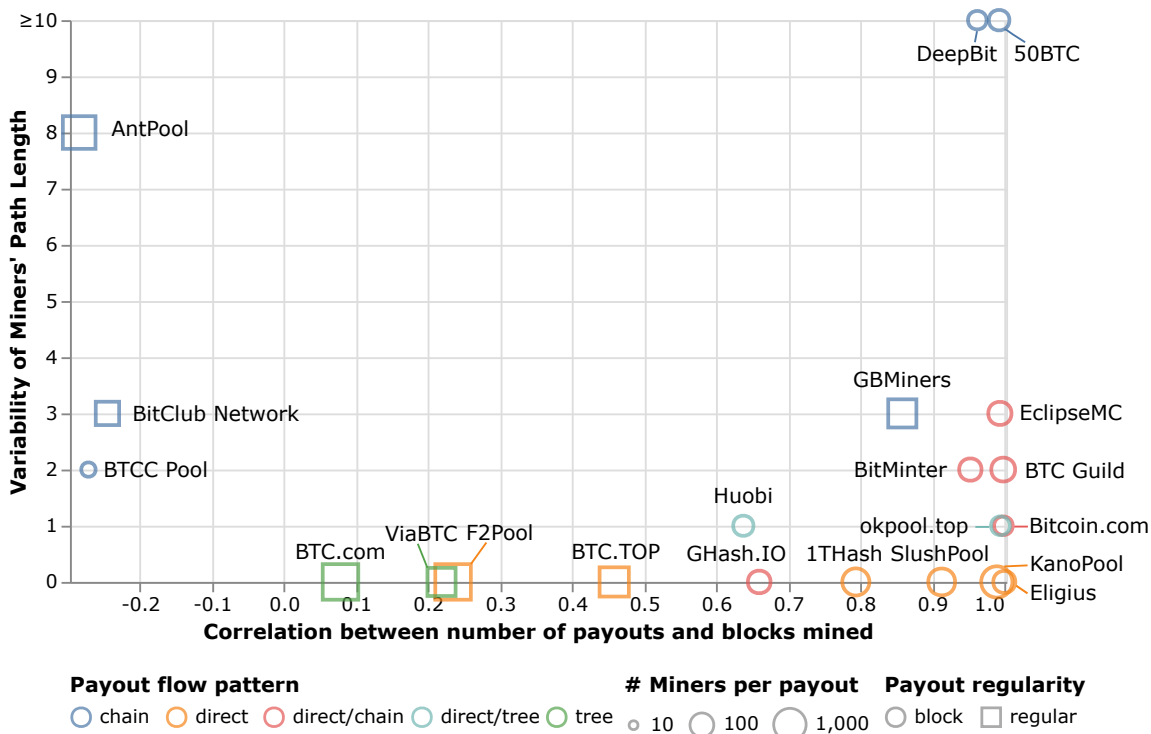
Figure 26: The scatter plot shows the payout flow pattern of mining pools regarding the payout regularity and payout flow structure. The color indicates the payout flow structure for each mining pool. The shape suggests whether a mining pool pay per block (round) or regularly (e.g., daily). The size of each point is Proportional to the median number of miners per payout on the logarithmic scale.
