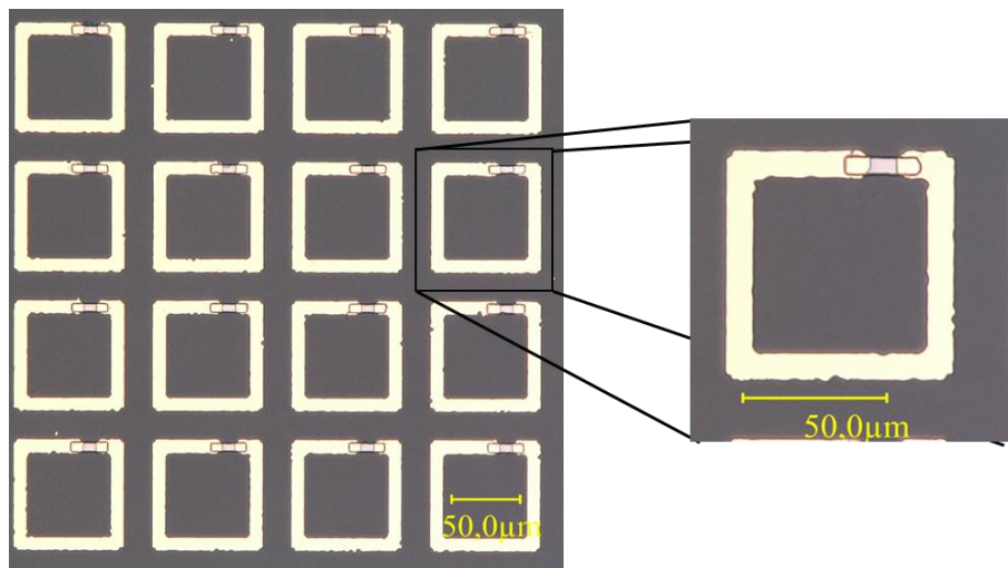
Figure III-29: Optical image of the fabricated hybrid SRR metamaterial and the corresponding unit cell with an asymmetric structure
