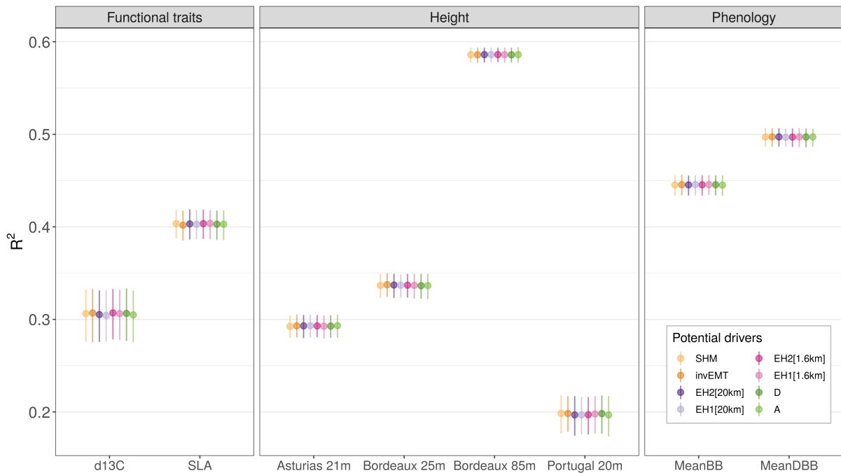
Figure X.11. Median and 95% intervals of the posterior distributions of the total variance explained by the models ( \mathcal{R}^2 ).
