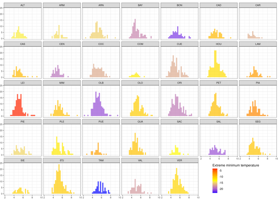
Figure X.8. Population-specific distributions of the specific leaf area (SLA) in Portugal. The color gradient corresponds to the extreme minimum temperature in the population location over the period 1901-1950.
