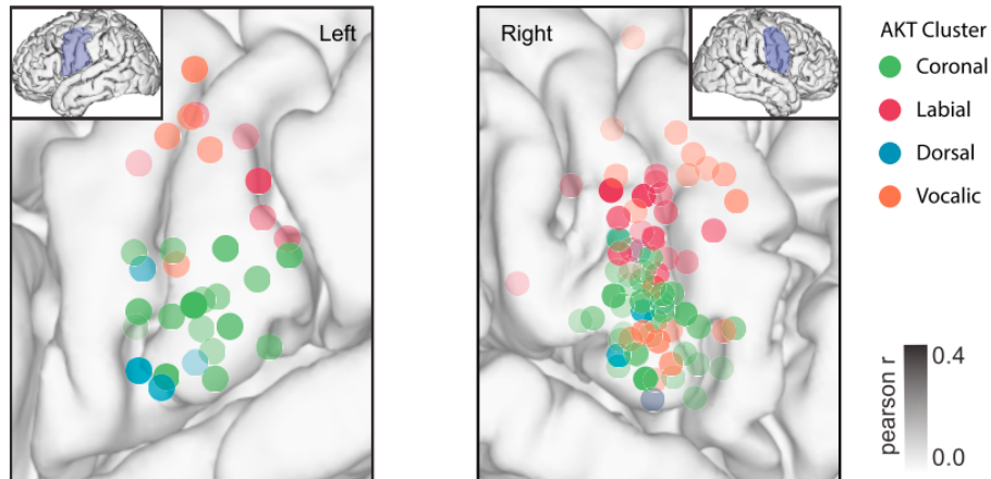
Figure 9. ECoG electrodes from five participants colored by type of vocal tract gesture mapped on common MRI-reconstructed brain. Opacity of electrode varies with Pearson's correlation coefficient from an encoding model of articulatory kinematic trajectory (AKT). This result shows that there is an overall subject-independent somatotopic organization of the articulatory gestures on the vSMC. Coronal and dorsal gestures refer to the front and back of the tongue. Vocalic gesture refers to voicing activity. Reprinted from Chartier et al. (2018).
