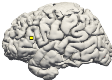
Figure 24. Localization of the Utah array on the reconstruction of the brain of participant P3. The reconstruction was obtained from pre-operative MRI.
