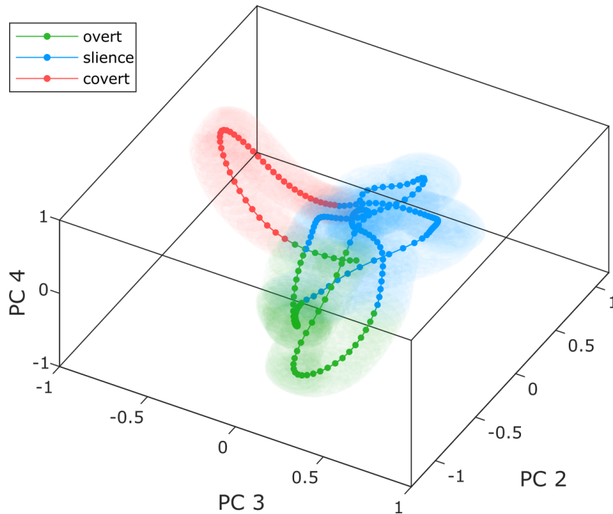
Figure 30. Trial-averaged projection of the firing rates of condition-modulated units using PCA. The firing rates of the 9 modulated units were projected in a 3-dimensional space using PCA. The components 2, 3, 4 were considered as they produced a nicely visible separation of the conditions. The projected trajectories were averaged while preserving the different phases of the trial (see section 6.2.2). The shaded areas are semi-transparent spheres whose radius is equal to the standard error of the mean (SEM). SEM was chosen instead of standard deviation in order to improve readability.
