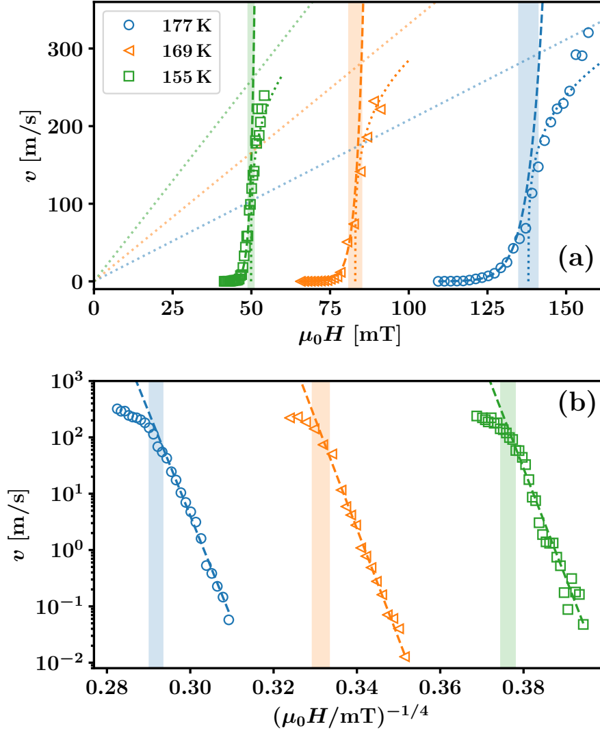
Figure 4.13: Depinning field determination for velocity curves below T_M and above 100 K. Velocity v vs. field \mu_0 H curves for T = 177 , 169 and 155 K, in (a) linear scale and (b) creep scale. We plot the creep fits at each temperature as dashed curves, and we indicate as vertical shaded areas the ranges in which we determine the depinning field occurs. For T = 177 K, we estimate \mu_0 H_d = (138 \pm 3) mT; for T = 169 K, \mu_0 H_d = (83 \pm 2) mT; and for T = 155 K, \mu_0 H_d = (49.9 \pm 0.9) mT. In the linear scale plot, zero-temperature depinning regime (equation (2.82)) with \beta = 0.25 corresponding to each of the temperatures are plotted as dotted curves. Resulting v_H values are v_H = 440 m/s for T = 177 K, v_H = 420 m/s for T = 169 K, and v_H = 400 m/s for T = 155 K. Calculations of flow regime mobilities permit us to indicate as dotted straight lines the predictions for the flow regime. Obtained mobilities are m = 2.1 , 3.3 and 5.2 (m/s)/mT for T = 177 , 169 and 155 K respectively.
