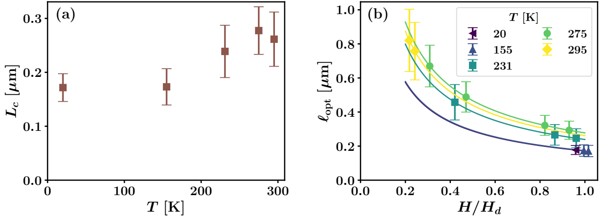
Figure 5.7: Calculated Larkin length L_c and optimal event size \ell_{\text{opt}} . (a) L_c vs. T for the considered set of temperatures. (b) \ell_{\text{opt}} vs. the reduced field H/H_d for the different temperatures, indicating the full dependence (5.12) and values corresponding to the analyzed domain walls.
