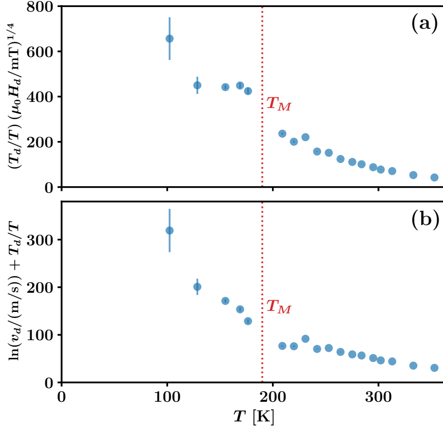
Figure 4.12: Creep fit parameters as a function of the temperature in the whole temperature range. (a) Slope S = (T_d/T)(\mu_0 H_d/\text{mT})^{1/4} and (b) intercept I = \ln(v_d/(\text{m/s})) + T_d/T resulting from the linear fits of the type y = Sx + I with y = \ln(v/(\text{m/s})) and x = (\mu_0 H/\text{mT})^{-1/4} . We indicate the position of magnetic compensation at T = 190 K as a vertical dotted line.
