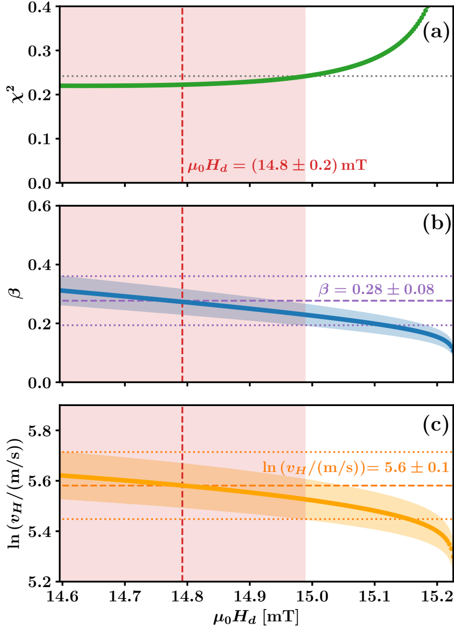
Figure 4.20: Depinning fit parameters as a function of \mu_0 H_d in the range (\mu_0 H_{d,\min}, H_{d,\max}) for T = 20 K. (a) \chi^2 vs. \mu_0 H_d . We indicate as an horizontal dotted line the limiting value 1.1 \chi^2_{\min} , which permits to define the range [\mu_0 H_d - \mu_0 \delta H_d, \mu_0 H_d + \mu_0 \delta H_d] in which \chi^2 < 1.1 \chi^2_{\min} . The depinning field is determined as \mu_0 H_d = (14.8 \pm 0.2) mT and indicated as a vertical dashed line and a shaded area. (b) Slope \beta vs. \mu_0 H_d , indicating the uncertainty in its determination in all the range as a shaded region around the mean value dependence. The final determination \beta = 0.28 \pm 0.08 is made taking into account this uncertainty, as indicated by the horizontal lines. (c) Intercept \ln(v_H/(m/s)) vs. \mu_0 H_d , indicating the uncertainty in its determination in all the range as a shaded region around the mean value dependence. The final determination \ln(v_H/(m/s)) = 5.6 \pm 0.1 is made taking into account this uncertainty, as indicated by the horizontal lines.
