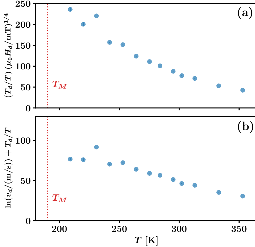
Figure 4.5: Creep fit parameters above T_M as a function of the temperature. (a) Slope S = (T_d/T)(\mu_0 H_d/\text{mT})^{1/4} and (b) intercept I = \ln(v_d/(\text{m/s})) + T_d/T resulting from the linear fits of the type y = Sx + I with y = \ln(v/(\text{m/s})) and x = (\mu_0 H/\text{mT})^{-1/4} . We indicate the position of magnetic compensation at T = 190 K as a vertical dotted line.
