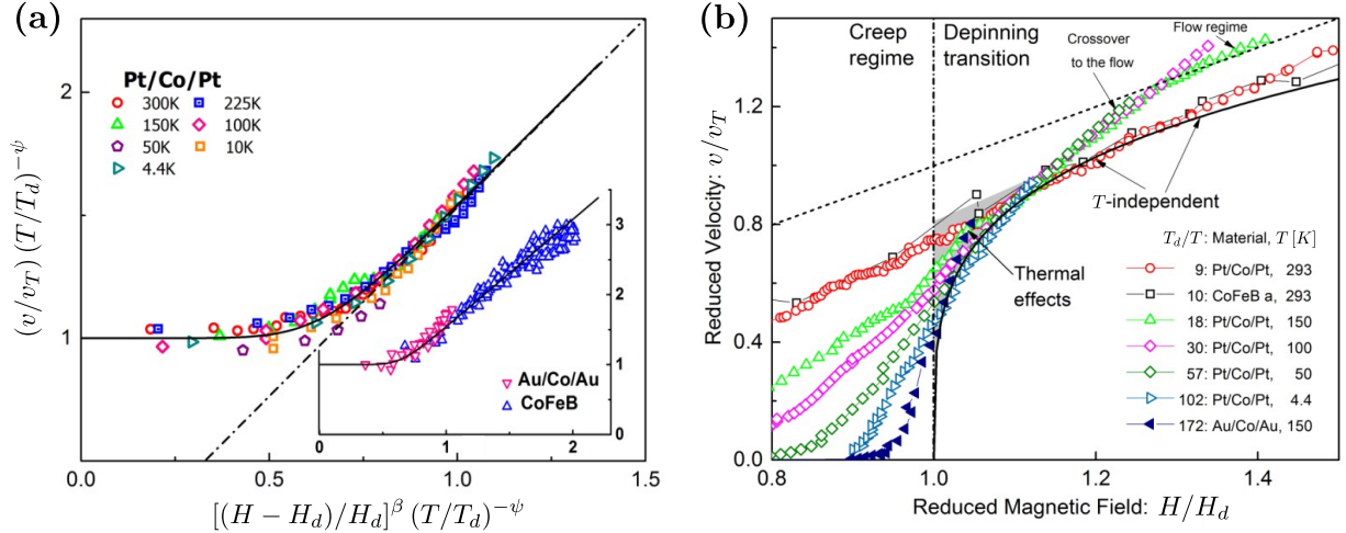
Figure 2.15: Universality of the depinning transition at finite temperature. (a) Universal depinning function plotted as a continuous line, and experimental data relating (v/v_T) (T/T_d)^{-\psi} vs. [(H - H_d)/H_d]^\beta (T/T_d)^{-\psi} , for Pt/Co/Pt at different temperatures (main panel) and for Au/Co/Au and CoFeB (inset). The dot-dashed straight line corresponds to the zero-temperature depinning law (2.82). (b) Reduced velocity v/v_T vs. reduced field H/H_d for different materials at different temperatures. The continuous line is the zero-temperature depinning law (2.82) with v_H = v_T/0.65 , and the dashed line corresponds to the flow regime with a mobility m = v_T/H_d . The limit at H_d between the universal creep regime and the universal depinning transition is indicated as a dot-dashed line. Thermal effects occur close to H_d due to the thermal rounding. A T -independent behavior is observed in a limited range in which the zero-temperature depinning law successfully describes experimental data. Above this range, a crossover occurs until v = m H , corresponding to the flow regime, is satisfied for sufficiently high H . Both figures are adapted from [18].
