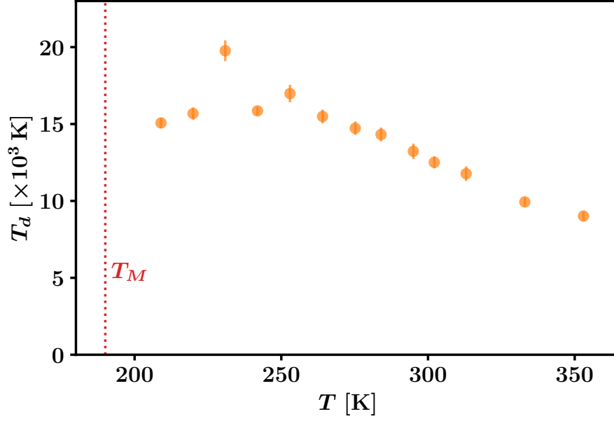
Figure 4.8: Depinning temperature vs. temperature for T > T_M . We indicate the position of magnetic compensation at T = 190 K as a vertical dotted line.
