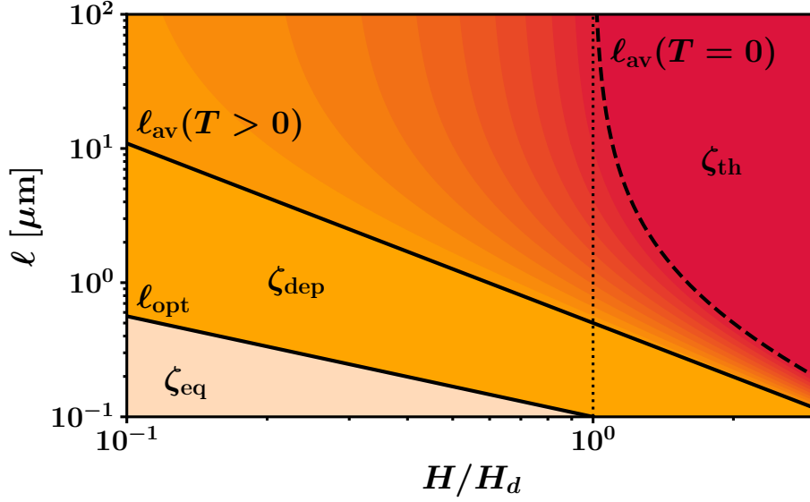
Figure 2.16: Crossover diagram showing the field-dependence of characteristic length-scales and associated roughness exponents. Optimal length \ell_{\text{opt}} and depinning avalanche length \ell_{\text{av}} as a function of the reduced field H/H_d in log-log scale. The expected behavior of \ell_{\text{av}} for T = 0 and for finite temperatures is indicated. A typical Larkin-length value L_c = 0.1 \mu\text{m} is considered. Different roughness exponents correspond to different length scale ranges: \zeta_{\text{eq}} corresponds to L_c < \ell < \ell_{\text{opt}} , \zeta_{\text{dep}} to \ell_{\text{opt}} < \ell < \ell_{\text{av}} , and \zeta_{\text{th}} to \ell > \ell_{\text{av}} .
