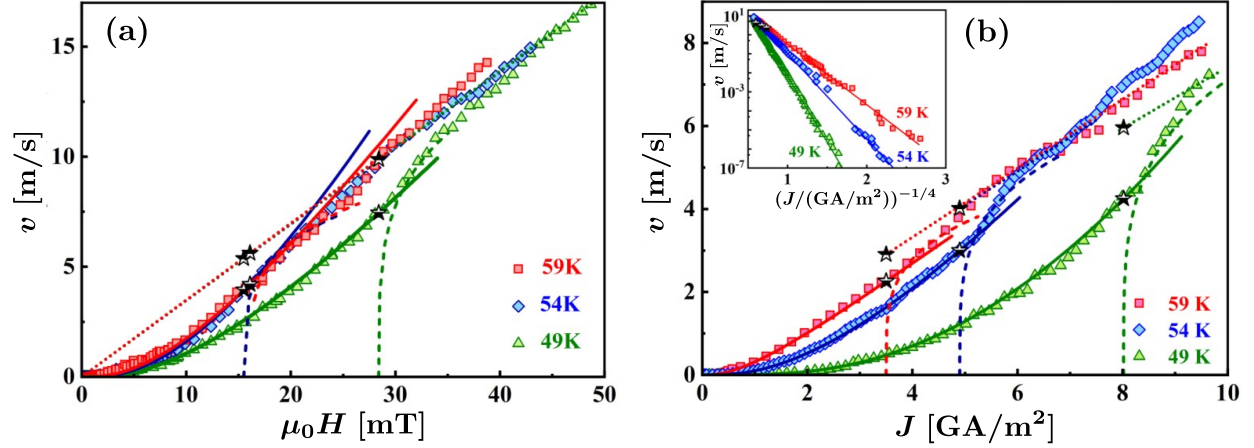
Figure 2.21: Field- and STT-driven domain wall motion in perpendicularly magnetized (Ga,Mn)(As,P)/(Ga,Mn)As. (a) Domain wall velocity v as a function of (a) the applied field \mu_0 H and (b) the current density J for different fixed temperatures. Solid lines indicate creep regime fits with a creep exponent \mu = 1/4 , while dashed lines correspond to the zero-temperature depinning transition and dotted lines to the flow regime. Inset of (b): creep-type plot of v in logarithmic scale vs. J^{-1/4} . Both figures are adapted from [27].
