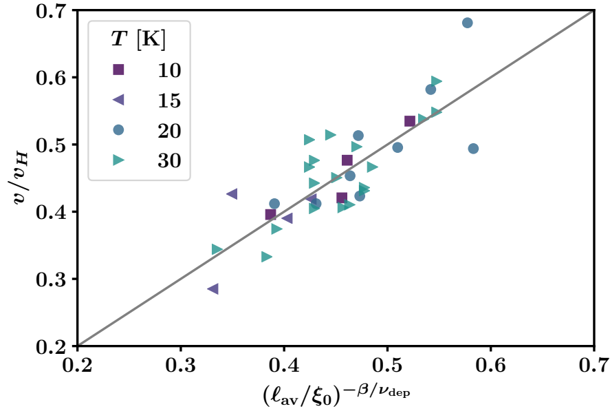
Figure 4.27: Common dependence of reduced parameters relating the mean domain wall velocity and the depinning avalanche length for different temperatures. We plot v/v_H vs. (\ell_{av}/\xi_0)^{-\beta/\nu_{dep}} , using the best values of v_H , \xi_0 , \beta and \nu_{dep} obtained for each temperature. Despite considerable fluctuations, the observed common dependence validates the relation given by (4.11).
