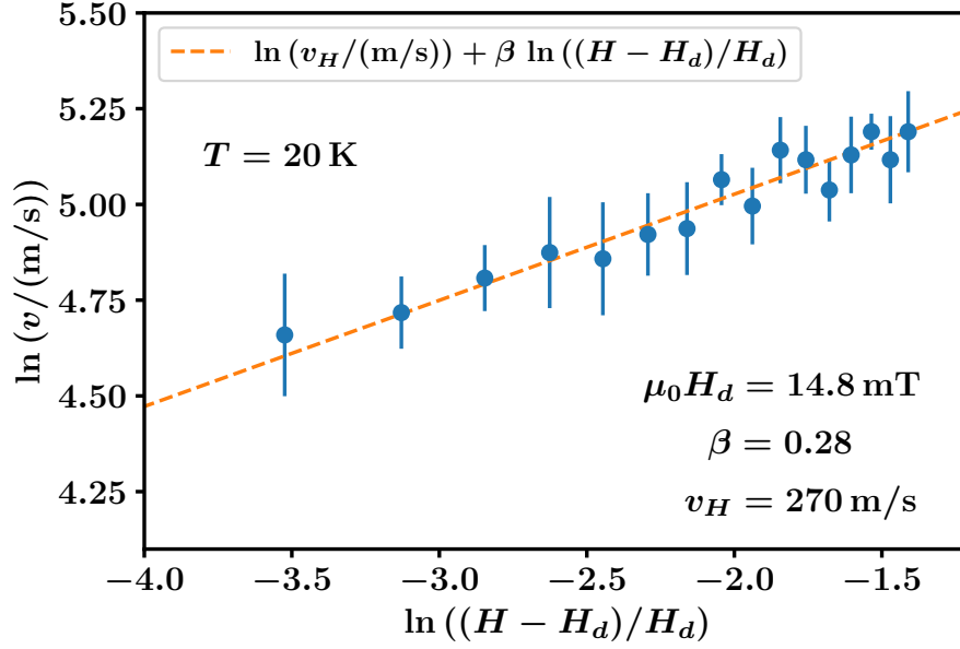
Figure 4.21: Log-log velocity vs. reduced field dependence corresponding to the athermal depinning transition for T = 20 K. \ln(v/(\text{m/s})) vs. \ln((H - H_d)/H_d) , considering \mu_0 H_d = 14.8 mT. We plot only the data points taken into account for the linear fits of the depinning law, i.e. those corresponding to \mu_0 H \geq \mu_0 H_{d,\text{max}} . The straight dashed line corresponds to the depinning law with our best determined parameters, \beta = 0.28 and v_H = 270 m/s.
