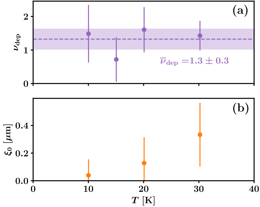
Figure 4.28: Depinning correlation length parameters \nu_{\text{dep}} and \xi_0 as a function of T for the lowest temperatures. (a) \nu_{\text{dep}} vs. T , indicating the mean obtained value \bar{\nu}_{\text{dep}} = 1.3 \pm 0.3 as a dashed horizontal line and a shaded area illustrating the uncertainty. (b) \xi_0 vs. T , where the value \xi_0 = (1 \pm 2) \mu\text{m} corresponding to T = 15 K has been omitted due to its out of scale value and uncertainty.
