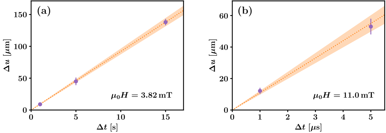
Figure 3.5: Domain wall displacement as a function of the pulse time. (a) Wall displacements \Delta u resulting from the application of pulses with a magnitude \mu_0 H = 3.82 \text{ mT} in the studied GdFeCo sample at T = 295 \text{ K} . The pulse durations \Delta t are 1, 5 and 15 s. All measured displacements are consistent with a domain wall velocity v = \Delta u / \Delta t = (9.2 \pm 0.4) \mu\text{m/s} , represented by the dotted line and the shaded region. (b) Fast wall displacements \Delta u resulting from the application of short pulses with a magnitude \mu_0 H = 11.0 \text{ mT} in the same sample, at the same temperature. The pulse durations are \Delta t = 1 and 5 \mu\text{s} . Both measured displacements are consistent with a wall velocity v = \Delta u / \Delta t = (11 \pm 1) \text{ m/s} which is represented by the dotted line and the shaded region.
