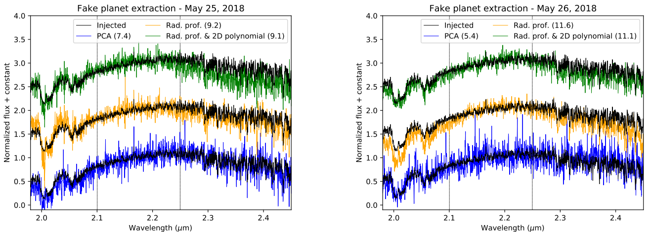
Fig. B.1. Comparison of the injected (black lines) and extracted simulated planet spectra (color lines) using the methods described in Sect. 2: PCA (blue), the removal of a circular profile at each wavelength (orange), and the removal of a 2D polynomial at each wavelength at the position of the simulated planet (green). The S/N of the recovered spectra is computed from 2.1 to 2.25 μm (dashed vertical lines) and given in parentheses.
