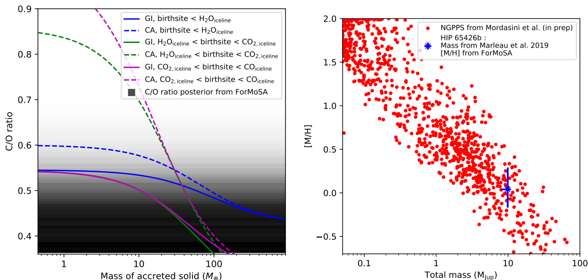
Fig. 10. Exploitation of our C/O and [M/H] to constrain the formation pathway. Left : comparison of the posterior of the C/O ratio given by ForMoSA (gradient; black: high likelihood) and different scenario of formation as a function of the accreted solid mass. The solid lines correspond to the GI scenario, and the dashed lines correspond to the CA scenario. The blue, green, and purple curves represent a formation within the water-ice line, between the water and CO 2 ice lines, and between CO 2 and CO ice lines, respectively. Right : comparison of the bulk enrichment of the NGPPS (red dots) and the estimated properties of HIP 65426 b (blue dot). We show here the NGPPS with a mass higher than 0.05 M_{\text{Jup}} (approximately the mass of Neptune).
