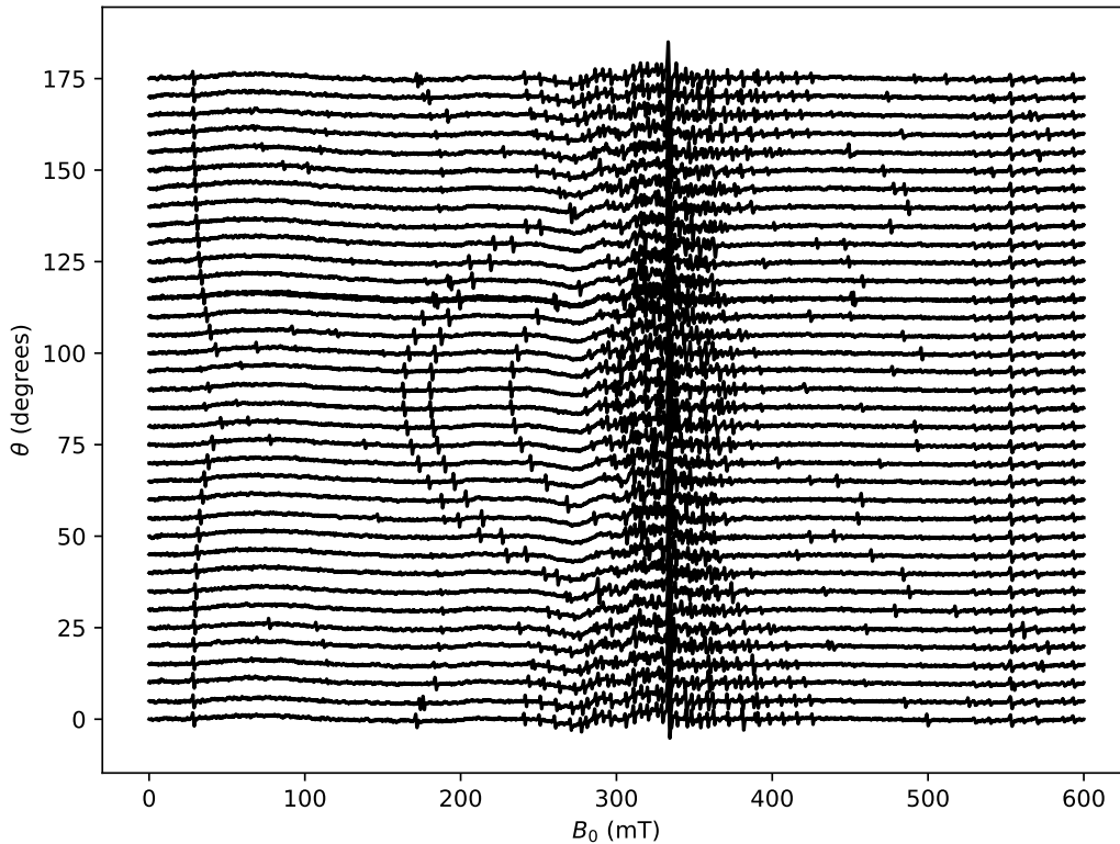
Figure 5.3 – ESR spectroscopy of sample 3 at room temperature with a Bruker spectrometer operating at \omega_0/2\pi = 9.63 GHz . The spectrum is measured at high power. We attribute most of the spin transitions to \text{Mn}^{2+} and \text{Gd}^{3+} [HB60], although we did not attempt to fit the spectrum.
