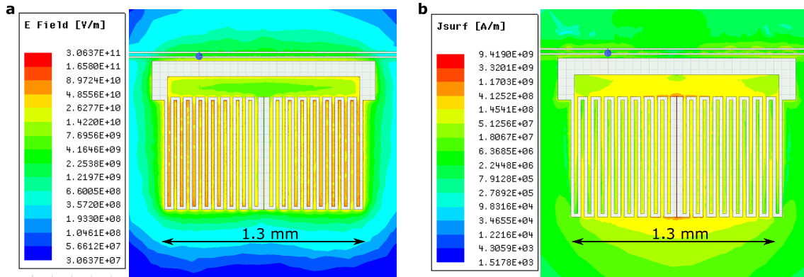
Figure 9.2 – HFSS simulations. a. Electric field in logarithmic scale with 1 Joule applied in the resonator mode. b. Surficial current in logarithmic scale with 1 Joule applied in the resonator mode. The blue dot on the feedline is simply the z -axis of the simulation pointing out of plane.
