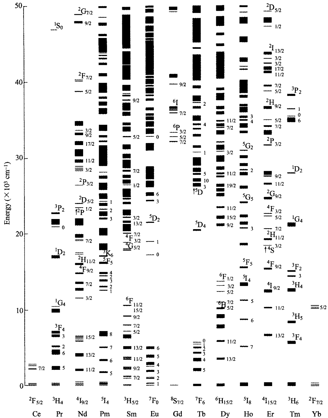
Figure 2.2 – Theoretical energy level structure of trivalent lanthanide ions in \text{LaF}_3 . This diagram, taken from [Car+89], labels each state with 2S+1L and/or J, depending on the dominant character of the levels, whether rather pure LS state or not. The tickness of each level depends on the crystal field splitting of the free-ion multiplets.
