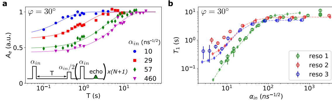
Figure 1.4 – Relaxation time of erbium ions in pure \text{CaWO}_4 and Purcell effect. a. Echo amplitude A_e generated by an inversion recovery sequence consisting of an inversion pulse of amplitude \alpha_{in} , followed after a delay T by a Hahn-echo sequence of same amplitude. The last pulse is repeated for enhanced signal averaging. The echo amplitude is plotted as a function of the delay T for several pulse amplitudes \alpha_{in} (colored symbols) and the data are fitted with exponential curves (solid lines). These measurements are performed at \varphi = 30^\circ . b. Fitted relaxation time as a function of the pulse amplitude \alpha_{in} , measured for the three resonators patterned on the sample (empty circles). Colored diamonds result from simulations where the only free parameters are the spin-lattice relaxation time and the input line attenuation.
