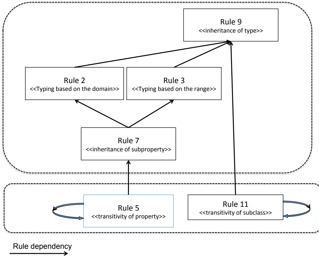
Figure 4.3: RDFS Ruleset Dependencies.
