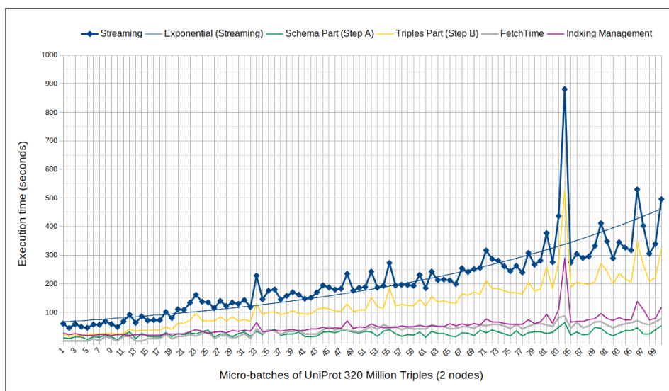
Figure 5.3: UniProt 320 Million Triples - Incremental Streaming (2 nodes)
