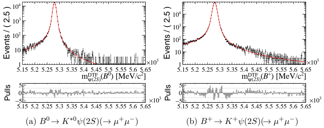
Figure E.6 – Fits to simulated muon \psi(2S) resonant modes B^0 \rightarrow K^{*0}\psi(2S)(\rightarrow \mu^+\mu^-) ( B^+ \rightarrow K^+\psi(2S)(\rightarrow \mu^+\mu^-) ) are shown on the left(right). The invariant mass is reconstructed with a DTF \psi(2S) mass constraint on the dimuon system. The fits shown above uses 15 + 16 simulation passing the muon LOL triggers.
