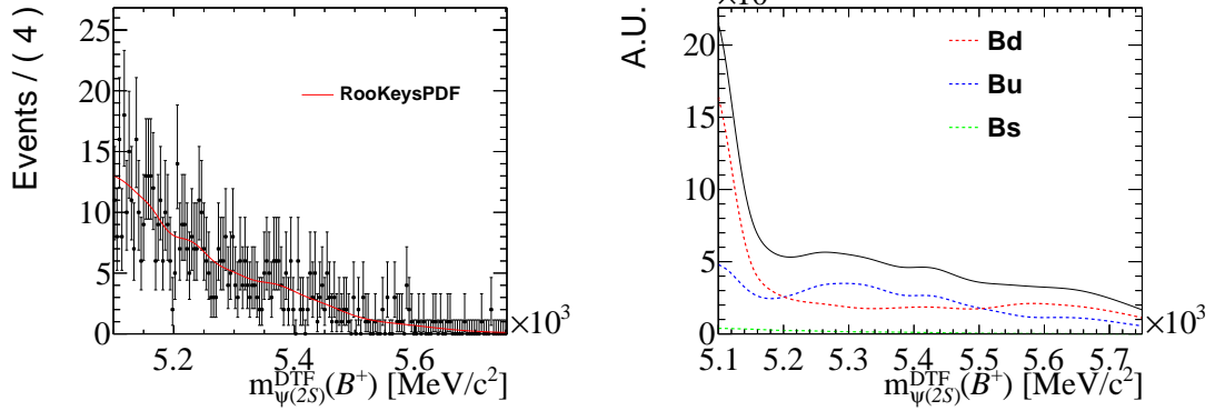
(c) B_s^0 \rightarrow XJ/\psi(\rightarrow e^+e^-) and B_s^0 \rightarrow X\psi(2S)(\rightarrow e^+e^-) (d) Inclusive B^0 , B^+ and B_s^0 decays combined
