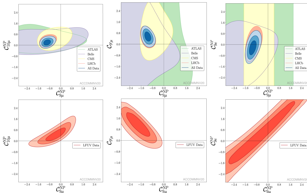
Figure 2.7 – From left to right: 2D fits to (\mathcal{C}_{9\mu}^{NP}, \mathcal{C}_{10\mu}^{NP}) , (\mathcal{C}_{9\mu}^{NP}, \mathcal{C}_{9\mu'}^{NP}) and (\mathcal{C}_{9\mu}^{NP}, \mathcal{C}_{9e}^{NP}) hypotheses using data from ”All” b \rightarrow s \ell^+ \ell^- observables (top) or ”LFUV” observables only (bottom). The allowed regions are bounded by 1, 2, 3 \sigma contour lines. The ”LFUV” fits deviate from SM at 2.9–3.7 \sigma while ”All” fits pulls, w.r.t. SM, are at 6.0 – 6.5 \sigma . Data from LHCb (dashed red) in the ”All” fit currently dominates the global fit. Figures extracted from Ref (67).
