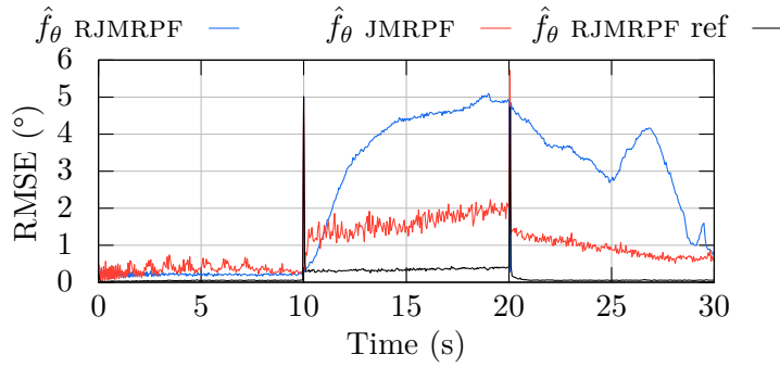
Figure 6.1: First 30s of the RMSE of the fault states of the simulation performed in Section 5.5.1 with a RJMPPF and a JMPPF with the transition probabilities set to 0.01 for \pi_{00} and \pi_{11} , and 0.99 for \pi_{10} and \pi_{01} . And with a RJMPPF reference (RJMPPF ref) which is the RMSE obtained in Section 5.5.1. Results based on 100 simulations.
