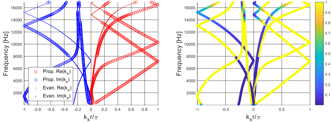
Figure 130: Dispersion curves computed for configuration 22 of Table 4.
