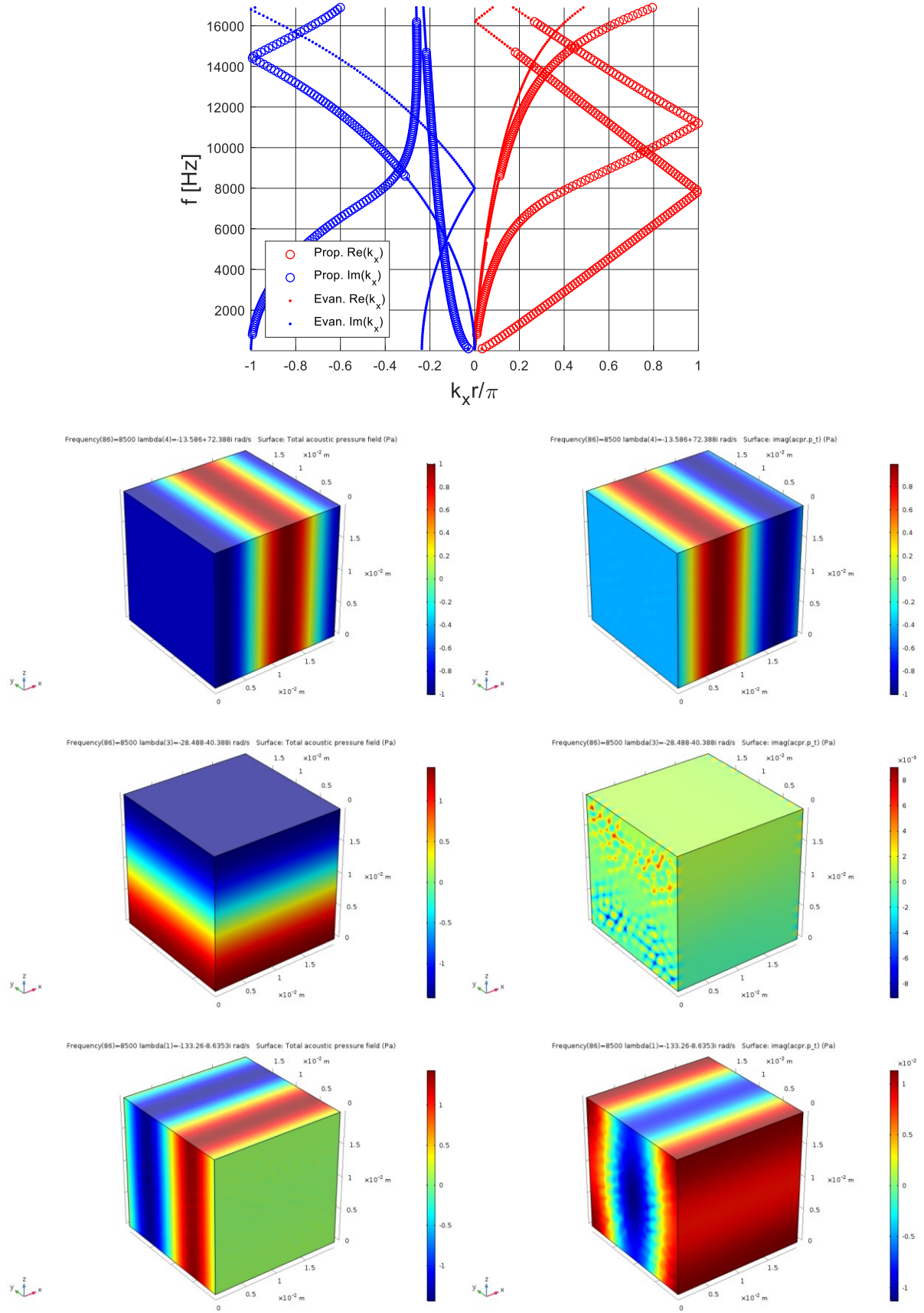
Figure 97: Dispersion curves for a homogeneous DB-modeled melamine 3D unit cell; from top to bottom, the 1 st , 2 nd and 3 rd branch eigenvectors are shown in terms of real (on the left) and imaginary (on the right) parts.
