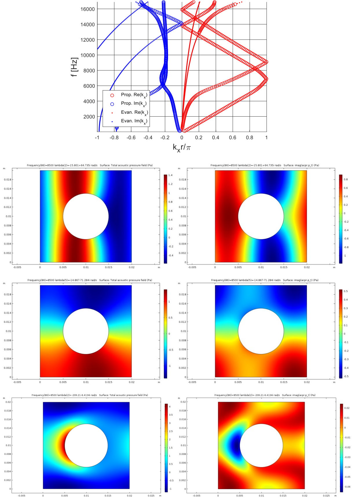
Figure 104: Dispersion curves for a JCA-modeled black PU 2D unit cell with a perfectly rigid inclusion; from top to bottom, the 1 st , 2 nd and 3 rd branch eigenvectors are shown in terms of real (on the left) and imaginary (on the right) parts.
