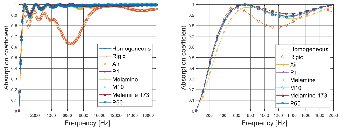
Figure 33: Comparison between the absorption coefficient curves for cases 17-24 of Table 4.
