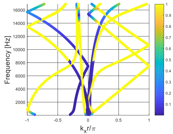
Figure 114: Dispersion curves computed for configuration 6 of Table 4.
