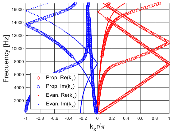
Figure 117: Dispersion curves computed for configuration 9 of Table 4.
