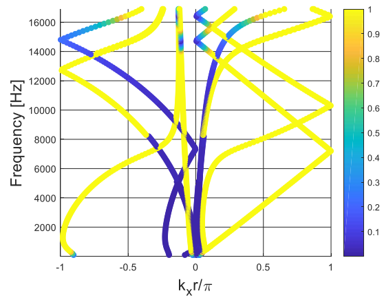
Figure 138: Dispersion curves computed for configuration 30 of Table 4.
