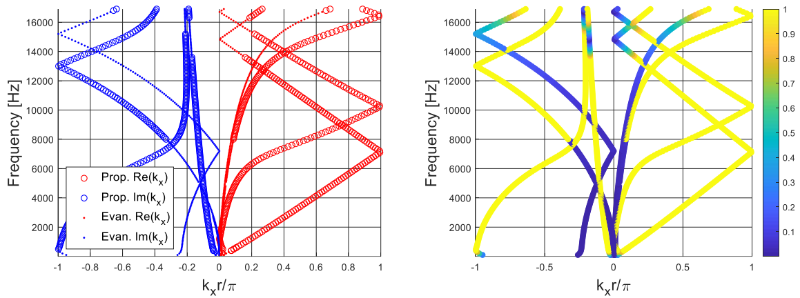
Figure 132: Dispersion curves computed for configuration 24 of Table 4.
