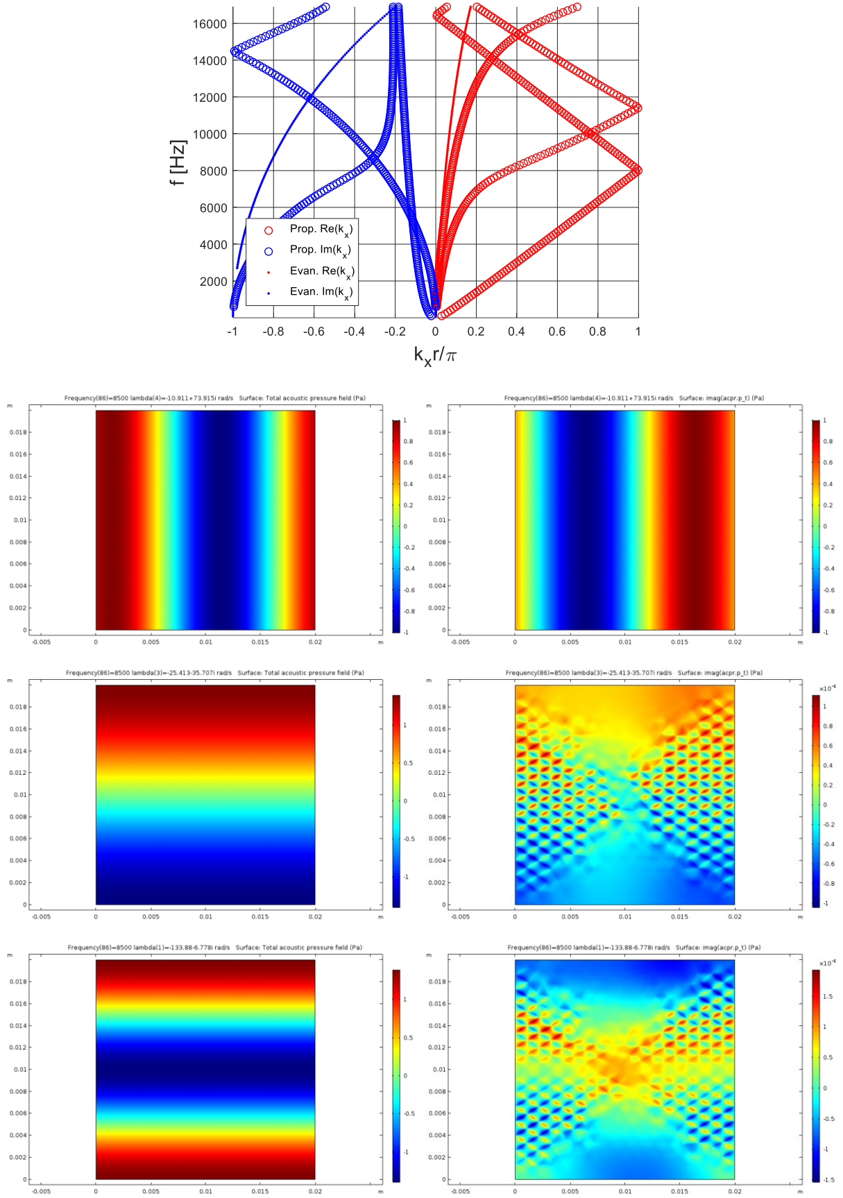
Figure 94: Dispersion curves for a homogeneous DB-modeled black PU 2D unit cell; from top to bottom, the 1 st , 2 nd and 3 rd branch eigenvectors are shown in terms of real (on the left) and imaginary (on the right) parts.
