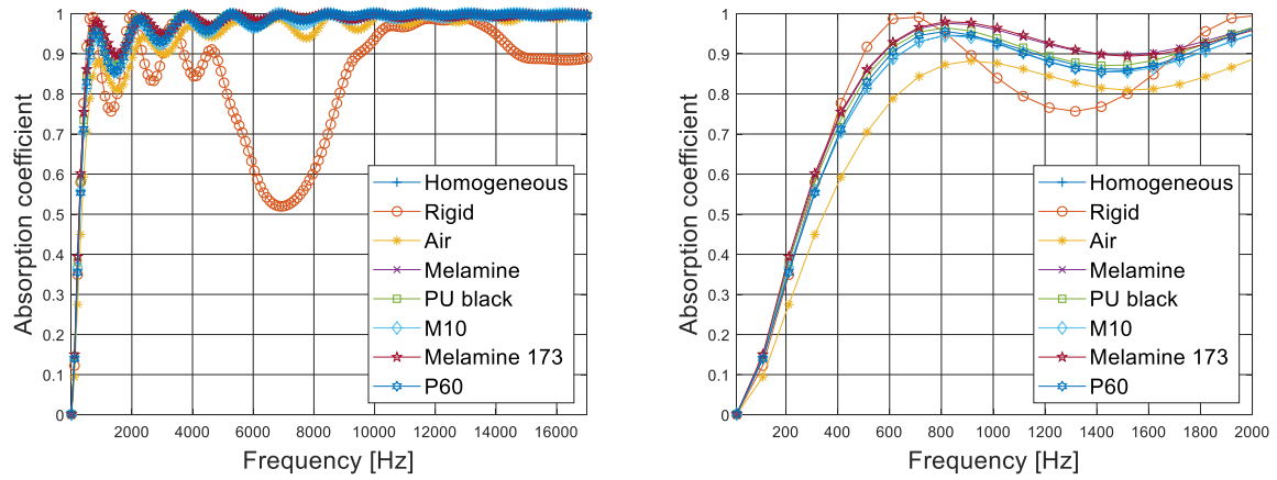
Figure 31: Comparison between the absorption coefficient curves for cases 9-16 of Table 4.
