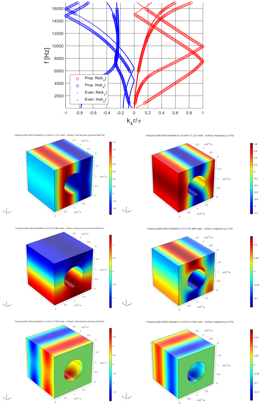
Figure 105: Dispersion curves for a DB-modeled melamine 3D unit cell with a perfectly rigid inclusion; from top to bottom, the 1 st , 2 nd and 3 rd branch eigenvectors are shown in terms of real (on the left) and imaginary (on the right) parts.
