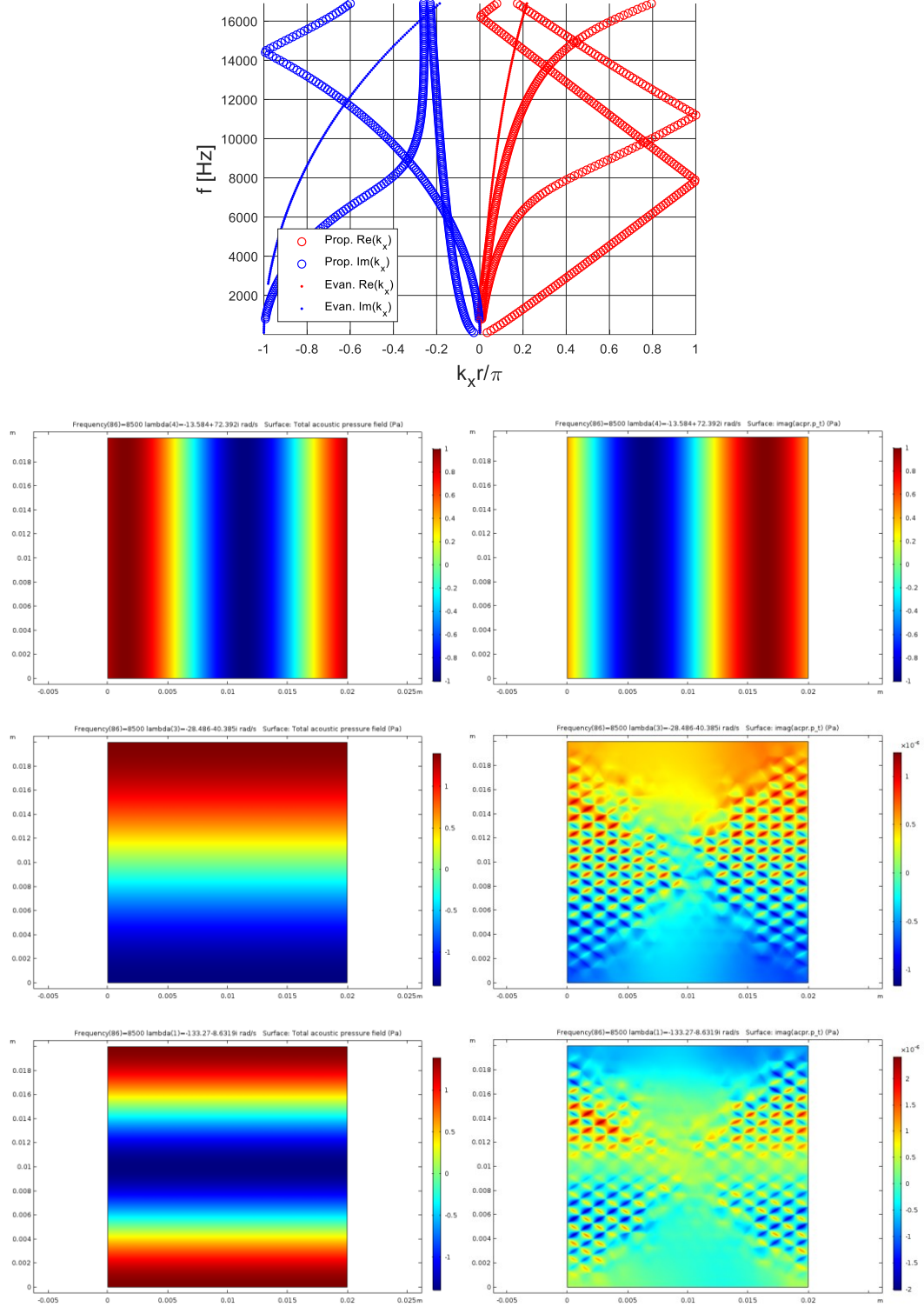
Figure 93: Dispersion curves for a homogeneous DB-modeled melamine 2D unit cell; from top to bottom, the 1 st , 2 nd and 3 rd branch eigenvectors are shown in terms of real (on the left) and imaginary (on the right) parts.
