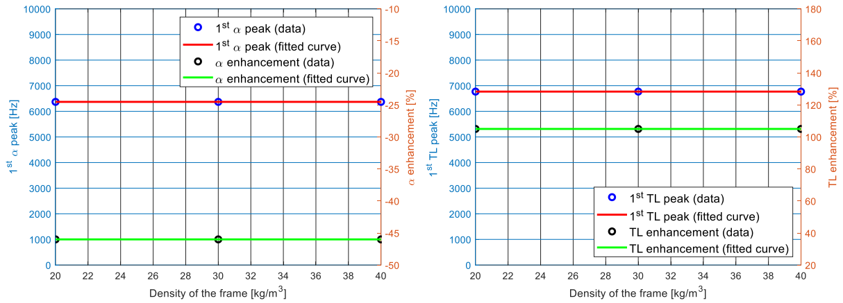
Figure 90: Absorption coefficient (on the left) and transmission loss (on the right) design curves as functions of the foam skeleton density.
