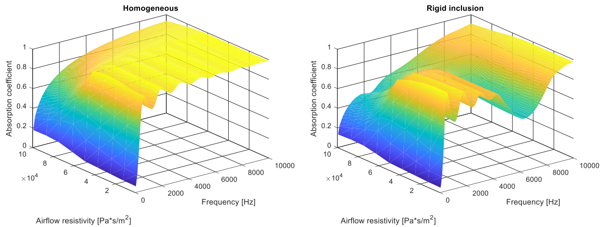
Figure 79: Absorption coefficient value as a function of frequency and foam airflow resistivity; homogeneous case (on the left) and case with a cylindrical perfectly rigid inclusion (on the right).
