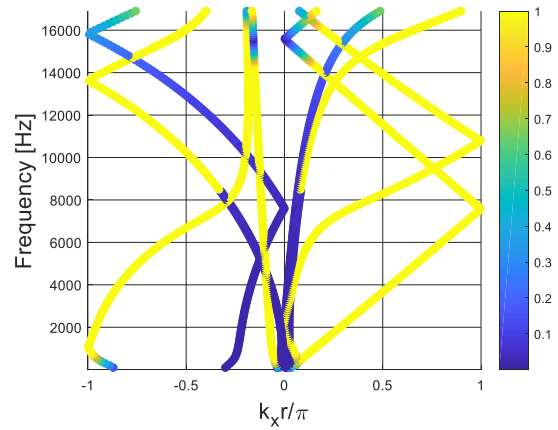
Figure 135: Dispersion curves computed for configuration 27 of Table 4.
