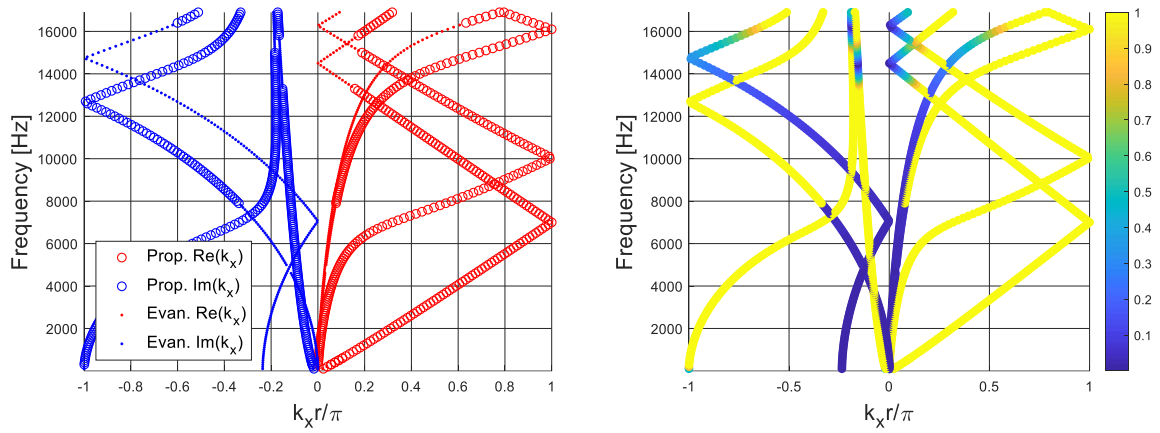
Figure 149: Dispersion curves computed for configuration 41 of Table 4.
