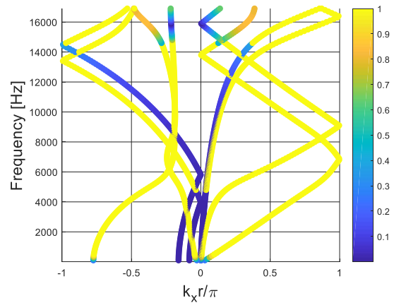
Figure 126: Dispersion curves computed for configuration 18 of Table 4.
