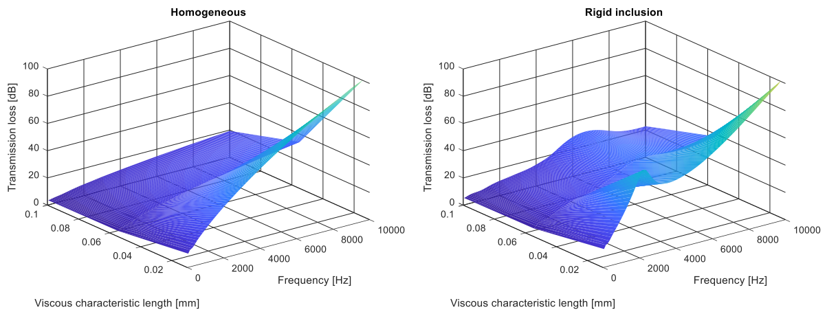
Figure 86: Transmission loss value as a function of frequency and foam viscous characteristic length; homogeneous case (on the left) and case with a cylindrical perfectly rigid inclusion (on the right).
