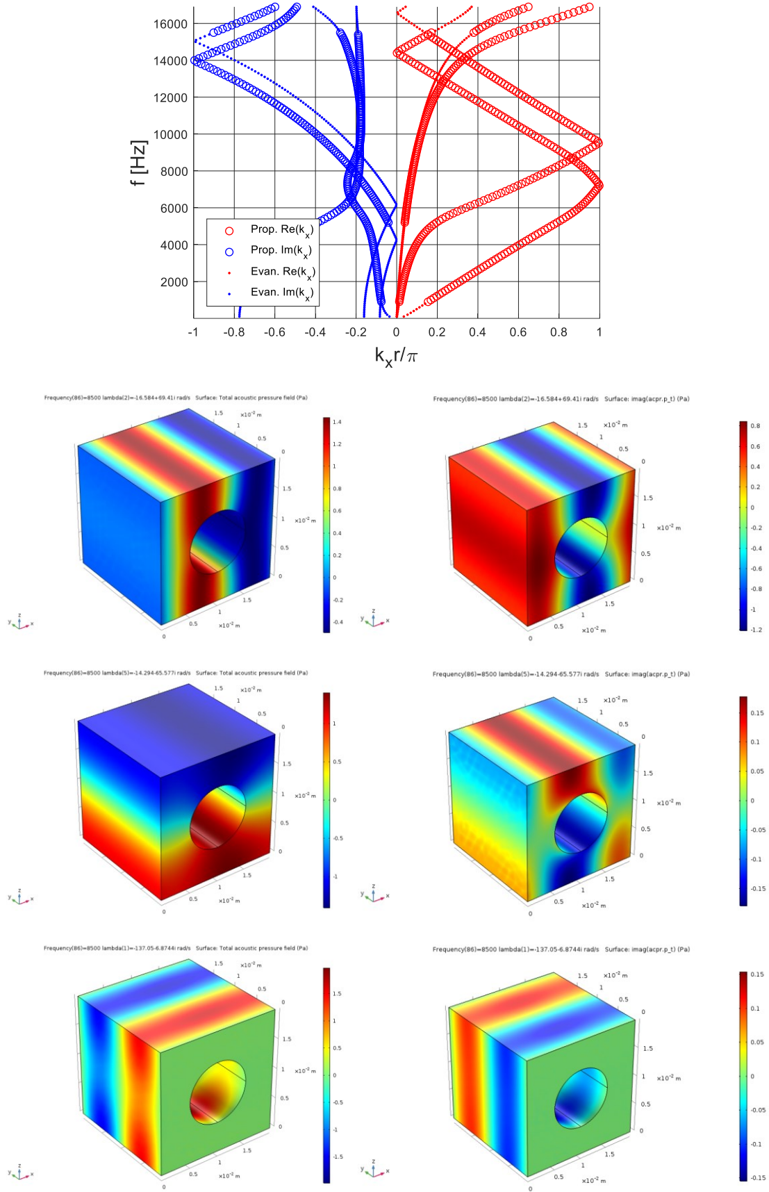
Figure 15: Dispersion curves for a JCA-modeled melamine 3D unit cell with a perfectly rigid inclusion; from top to bottom, the 1 st , 2 nd and 3 rd branch eigenvectors are shown in terms of real (on the left) and imaginary (on the right) parts.
