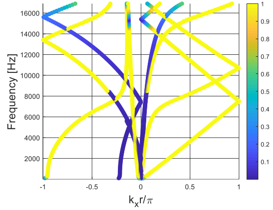
Figure 124: Dispersion curves computed for configuration 16 of Table 4.
