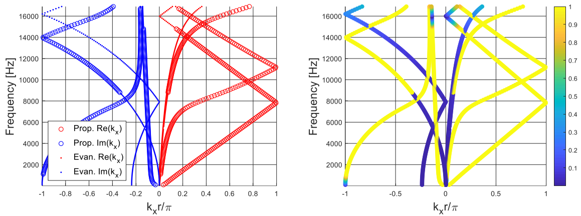
Figure 141: Dispersion curves computed for configuration 33 of Table 4.
