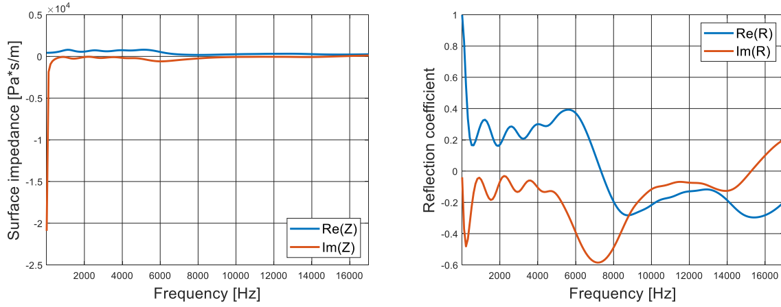
Figure 185: Surface impedance (on the left) and reflection coefficient (on the right) computed for a JCA-modeled melamine 3D unit cell with a perfectly rigid inclusion; \sigma = 7500 \frac{\text{Pa}\cdot\text{s}}{\text{m}^2} .
