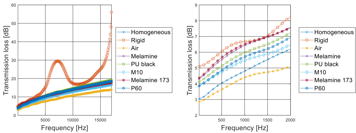
Figure 32: Comparison between the transmission loss curves for cases 9-16 of Table 4.
