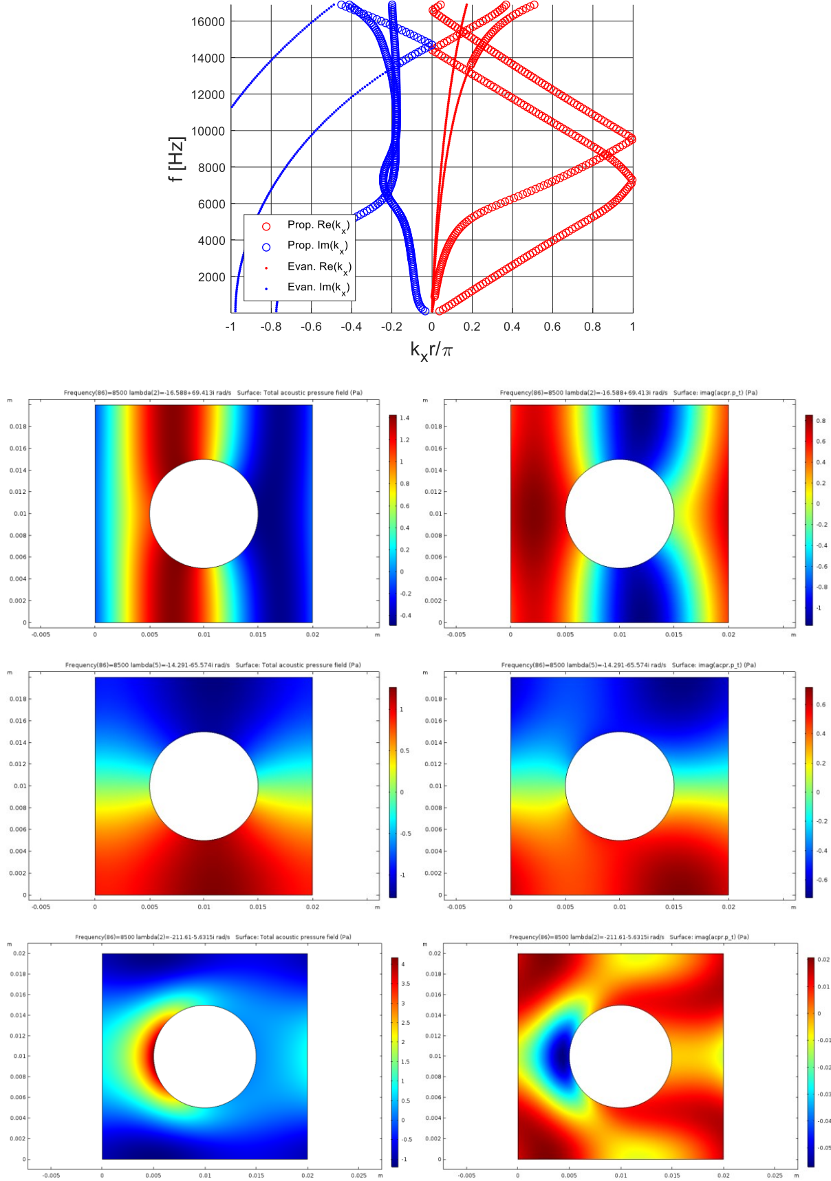
Figure 14: Dispersion curves for a JCA-modeled melamine 2D unit cell with a perfectly rigid inclusion; from top to bottom, the 1 st , 2 nd and 3 rd branch eigenvectors are shown in terms of real (on the left) and imaginary (on the right) parts.
