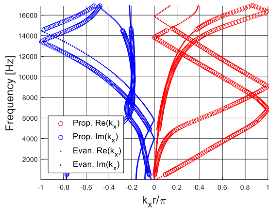
Figure 126: Dispersion curves computed for configuration 18 of Table 4.
