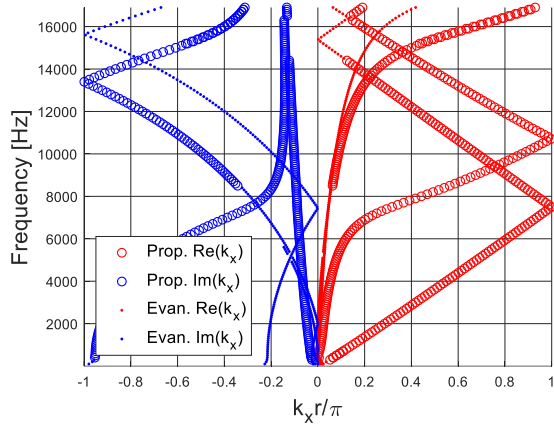
Figure 124: Dispersion curves computed for configuration 16 of Table 4.
