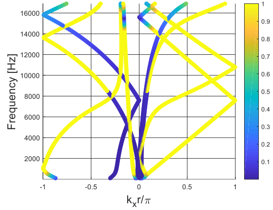
Figure 112: Dispersion curves computed for configuration 4 of Table 4.
