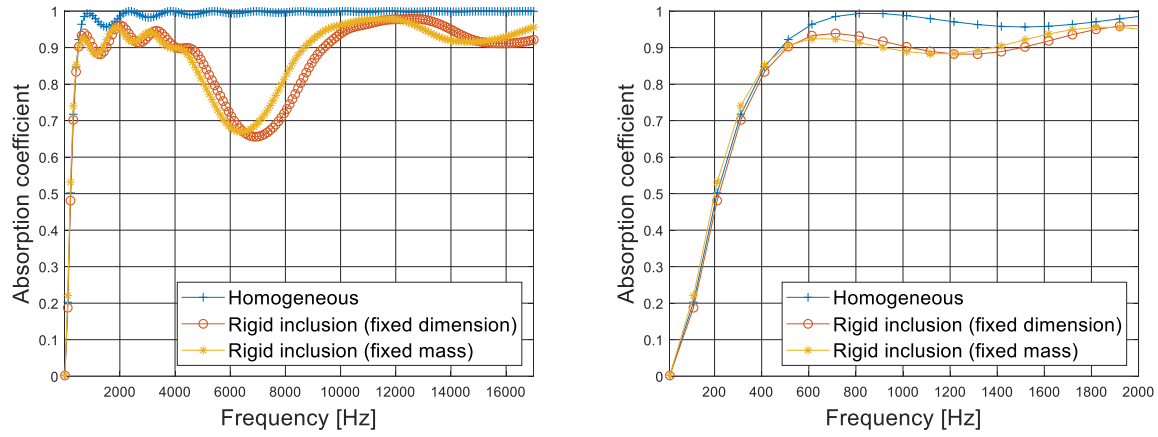
Figure 46: Comparison of absorption coefficient curves between the homogeneous case, the case with inclusion with fixed dimensions and the case with inclusion with fixed mass, computed for a 3D JCA-modeled melamine foam.
