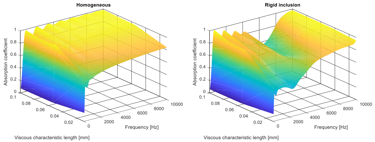
Figure 85: Absorption coefficient value as a function of frequency and foam viscous characteristic length; homogeneous case (on the left) and case with a cylindrical perfectly rigid inclusion (on the right).
