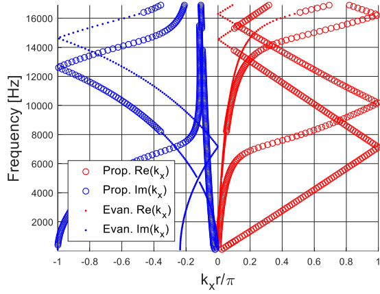
Figure 133: Dispersion curves computed for configuration 25 of Table 4.
