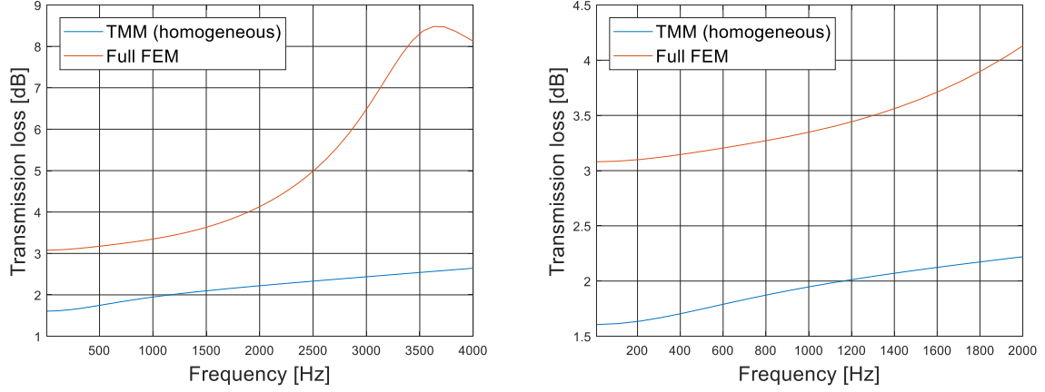
Figure 51: Transmission loss curve for the unit cell with Helmholtz resonators.
