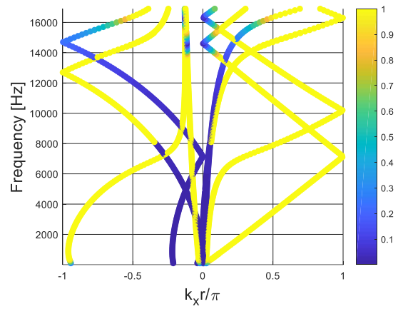
Figure 137: Dispersion curves computed for configuration 29 of Table 4.
