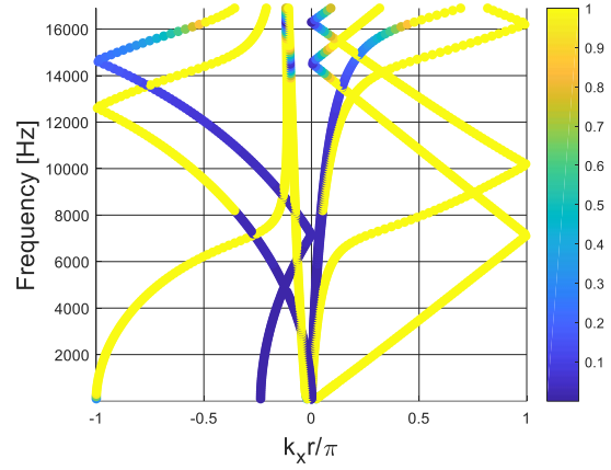
Figure 133: Dispersion curves computed for configuration 25 of Table 4.
