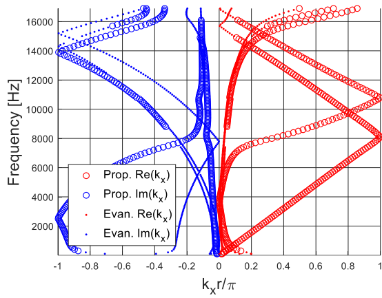
Figure 134: Dispersion curves computed for configuration 26 of Table 4.
