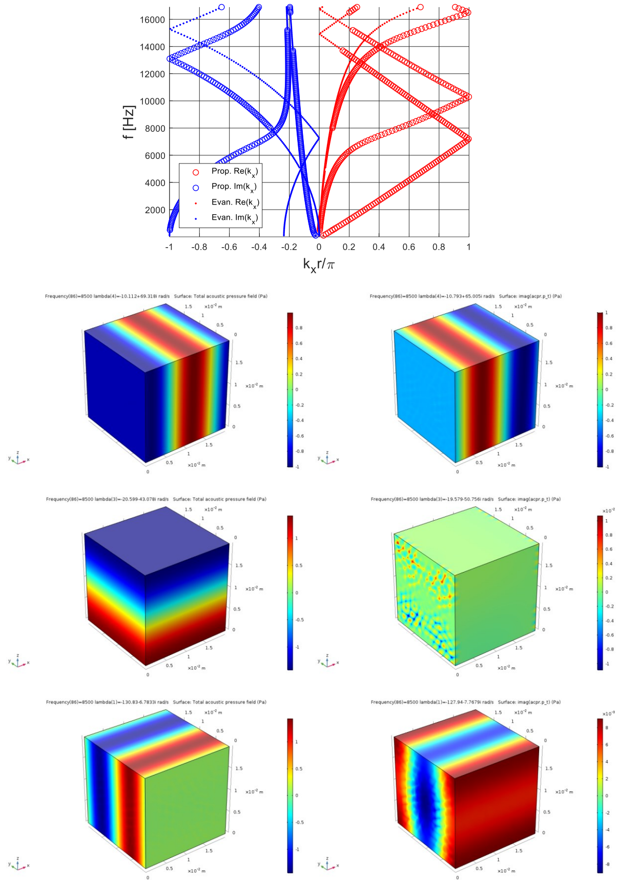
Figure 100: Dispersion curves for a homogeneous JCA-modeled black PU 3D unit cell; from top to bottom, the 1 st , 2 nd and 3 rd branch eigenvectors are shown in terms of real (on the left) and imaginary (on the right) parts.
