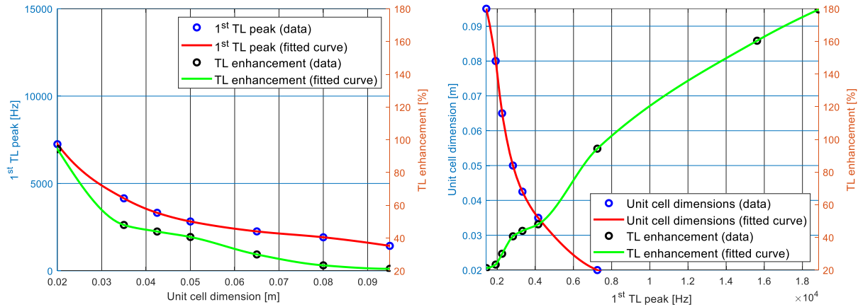
Figure 42: Transmission loss design curves as functions of the unit cell dimension (on the left) and the frequency of the 1 st peak (on the right), in the case of a 3D JCA-modeled melamine foam.
