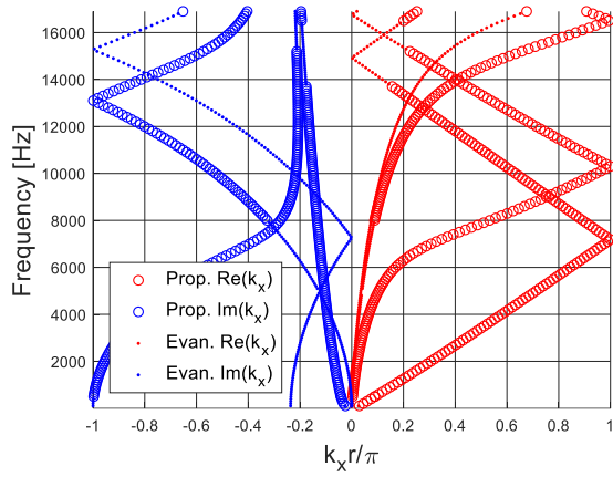
Figure 125: Dispersion curves computed for configuration 17 of Table 4.
