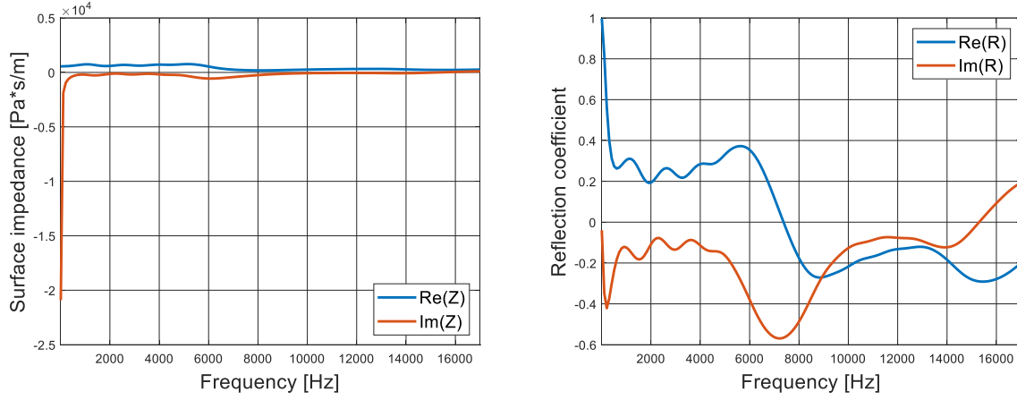
Figure 186: Surface impedance (on the left) and reflection coefficient (on the right) computed for a JCA-modeled melamine 3D unit cell with a perfectly rigid inclusion; \sigma = 10000 \frac{\text{Pa}\cdot\text{s}}{\text{m}^2} .
