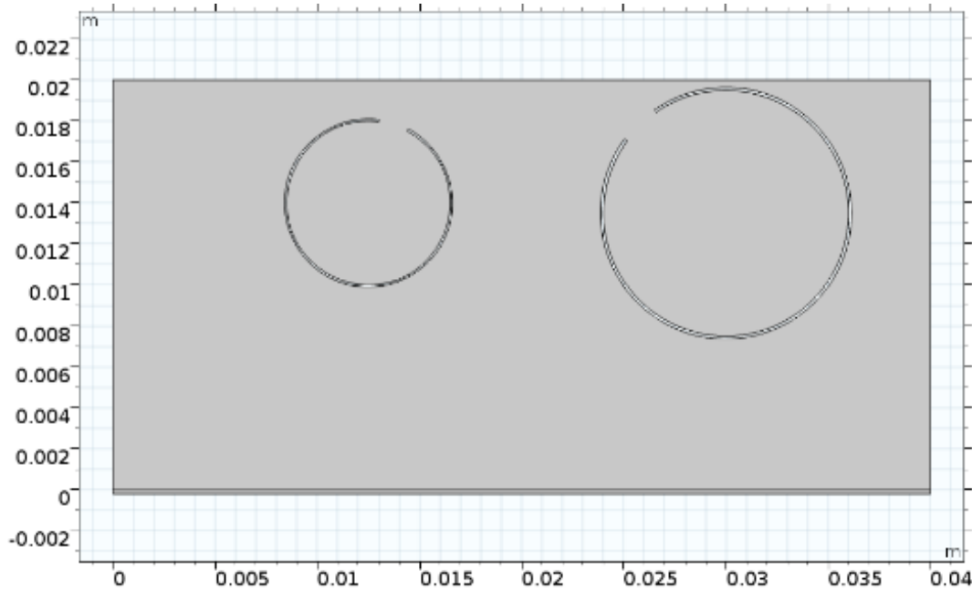
Figure 48: Unit cell with Helmholtz resonators [129].
