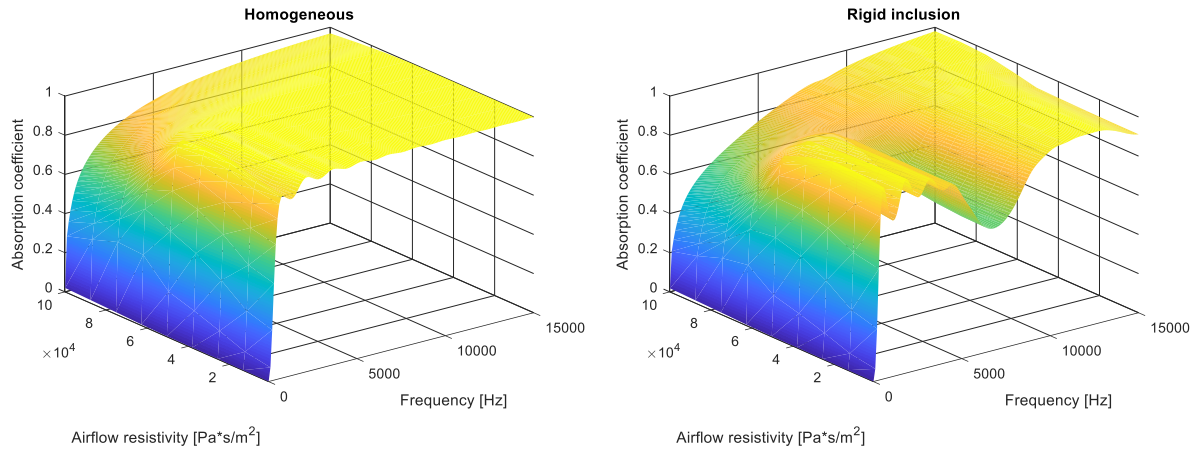
Figure 44: Absorption coefficient value as a function of frequency and foam airflow resistivity; homogeneous case (on the left) and case with a cylindrical perfectly rigid inclusion (on the right), computed for a 3D JCA-modeled melamine foam.
