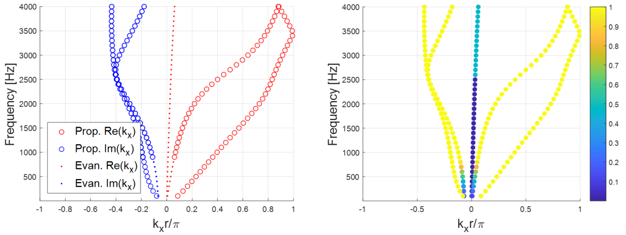
Figure 52: Dispersion curves for the unit cell with Helmholtz resonators.
