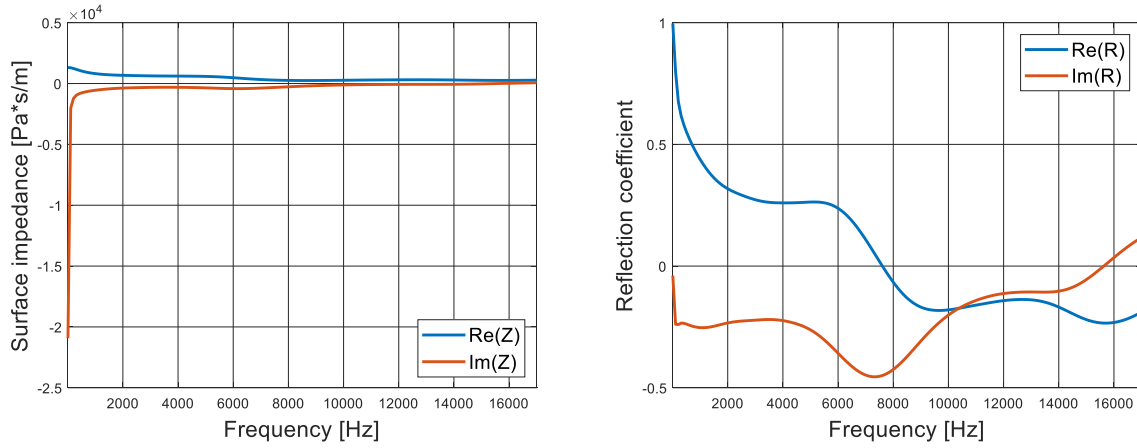
Figure 187: Surface impedance (on the left) and reflection coefficient (on the right) computed for a JCA-modeled melamine 3D unit cell with a perfectly rigid inclusion; \sigma = 25000 \frac{\text{Pa}\cdot\text{s}}{\text{m}^2} .
