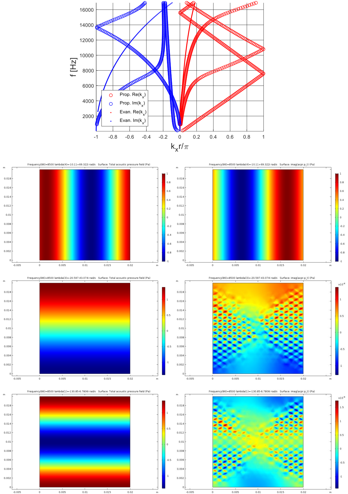
Figure 95: Dispersion curves for a homogeneous JCA-modeled melamine 2D unit cell; from top to bottom, the 1 st , 2 nd and 3 rd branch eigenvectors are shown in terms of real (on the left) and imaginary (on the right) parts.
