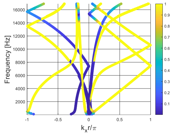
Figure 116: Dispersion curves computed for configuration 8 of Table 4.
