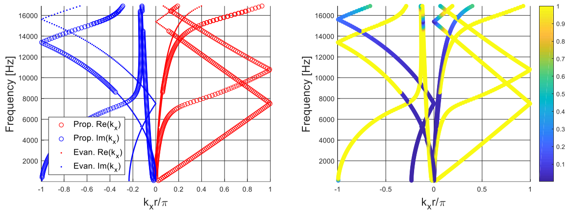
Figure 122: Dispersion curves computed for configuration 14 of Table 4.
