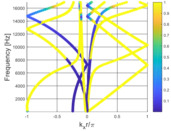
Figure 136: Dispersion curves computed for configuration 28 of Table 4.
