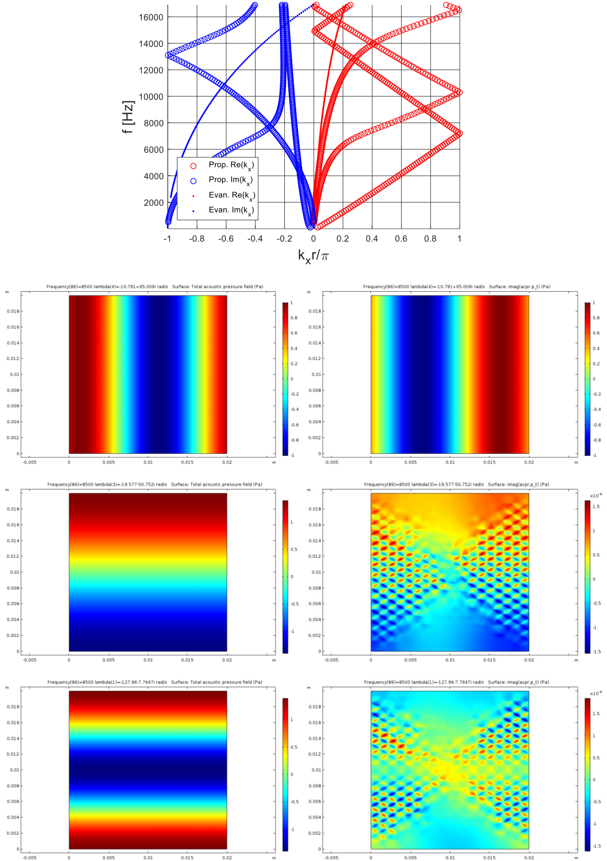
Figure 96: Dispersion curves for a homogeneous JCA-modeled black PU 2D unit cell; from top to bottom, the 1 st , 2 nd and 3 rd branch eigenvectors are shown in terms of real (on the left) and imaginary (on the right) parts.
