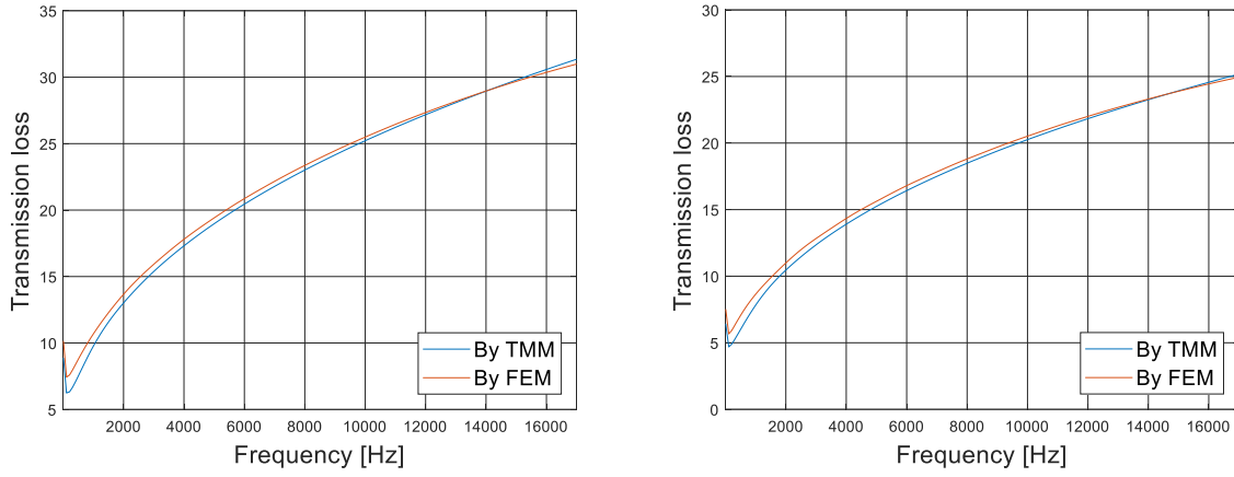
Figure 191: Transmission loss computed for a homogeneous DB-modeled melamine (on the left) and black PU (on the right) 2D unit cell.
