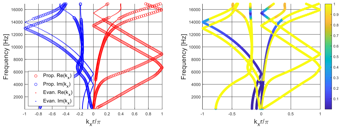
Figure 150: Dispersion curves computed for configuration 42 of Table 4.
