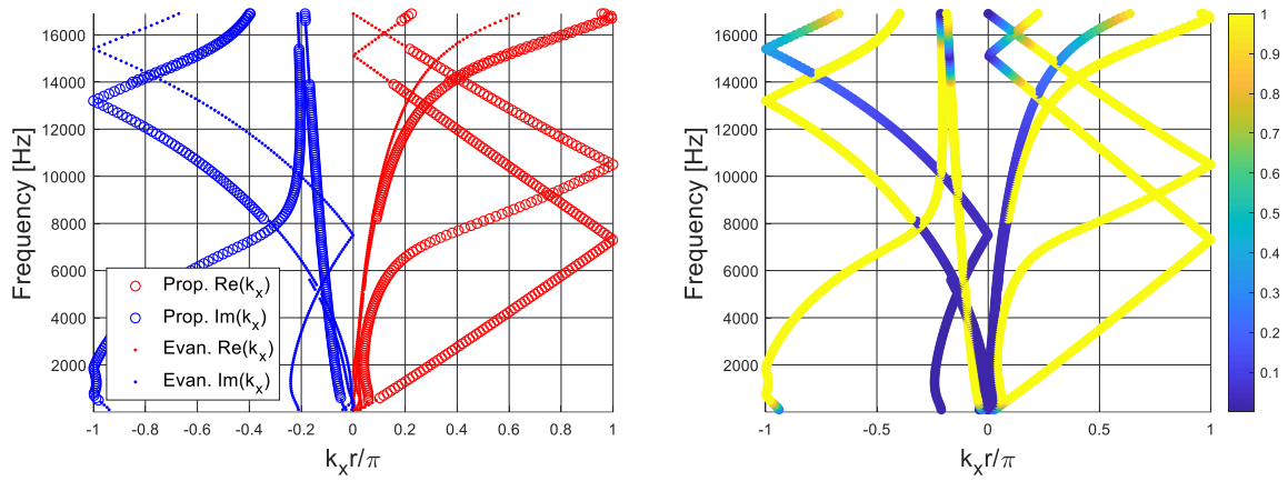
Figure 131: Dispersion curves computed for configuration 23 of Table 4.
