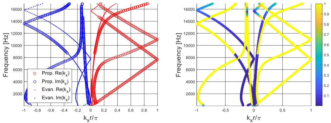
Figure 123: Dispersion curves computed for configuration 15 of Table 4.
