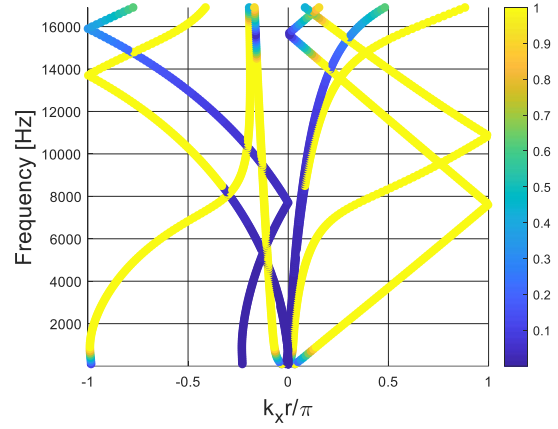
Figure 115: Dispersion curves computed for configuration 7 of Table 4.
