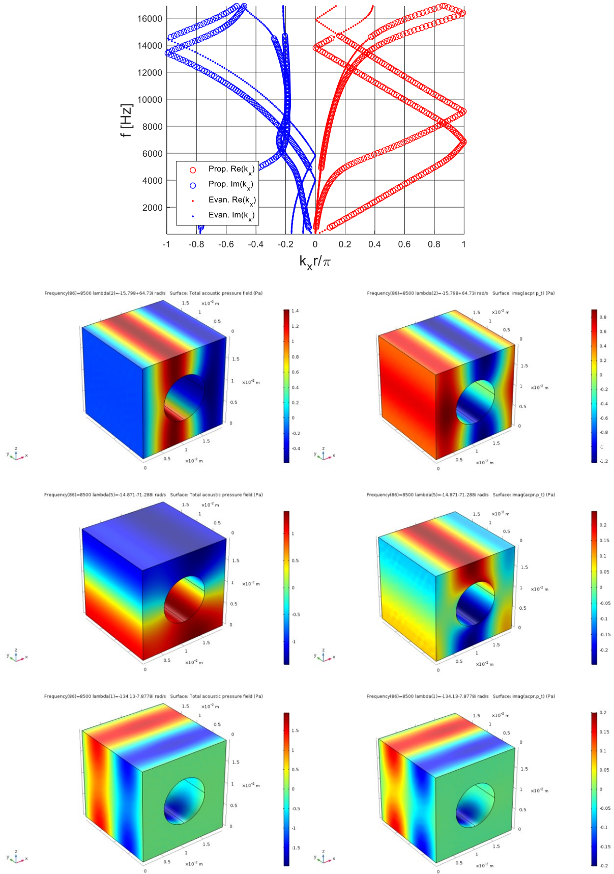
Figure 108: Dispersion curves for a JCA-modeled black PU 3D unit cell with a perfectly rigid inclusion; from top to bottom, the 1 st , 2 nd and 3 rd branch eigenvectors are shown in terms of real (on the left) and imaginary (on the right) parts.
