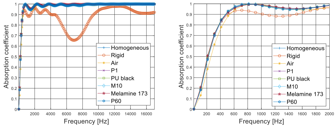
Figure 29: Comparison between the absorption coefficient curves for cases 1-8 of Table 4.
