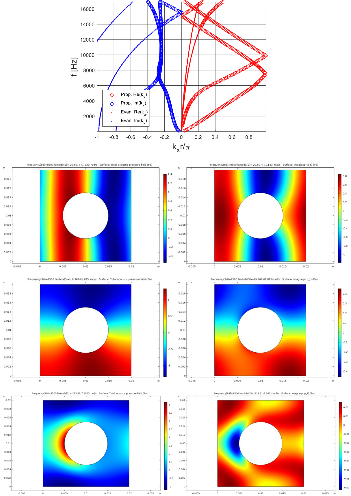
Figure 101: Dispersion curves for a DB-modeled melamine 2D unit cell with a perfectly rigid inclusion; from top to bottom, the 1 st , 2 nd and 3 rd branch eigenvectors are shown in terms of real (on the left) and imaginary (on the right) parts.
