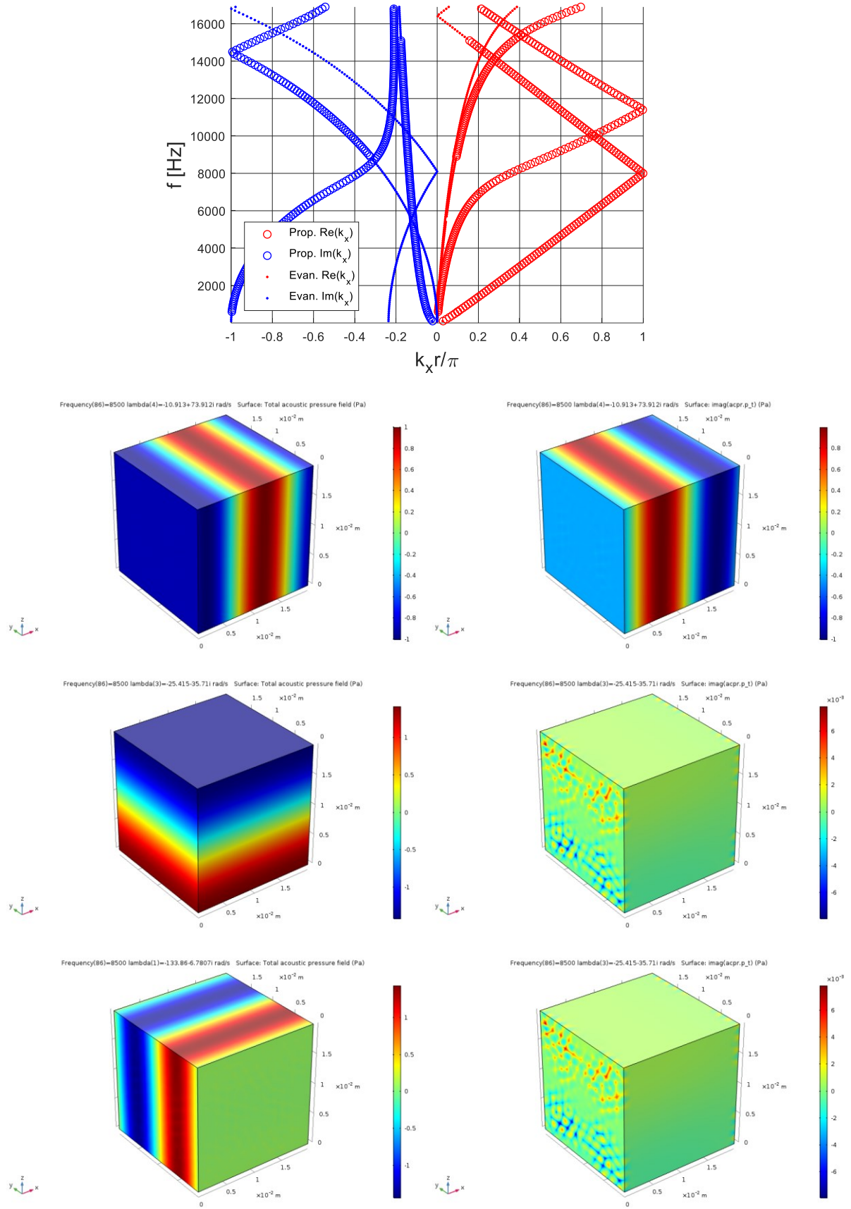
Figure 98: Dispersion curves for a homogeneous DB-modeled black PU 3D unit cell; from top to bottom, the 1 st , 2 nd and 3 rd branch eigenvectors are shown in terms of real (on the left) and imaginary (on the right) parts.
