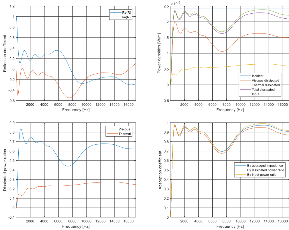
Figure 166: Reflection coefficient, power densities, dissipated power ratios and absorption coefficient computed for a DB-modeled black PU 2D unit cell with a perfectly rigid inclusion.
