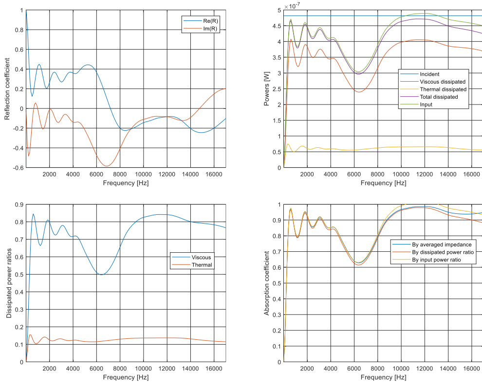
Figure 172: Reflection coefficient, powers, dissipated power ratios and absorption coefficient computed for a JCA-modeled black PU 3D unit cell with a perfectly rigid inclusion.
