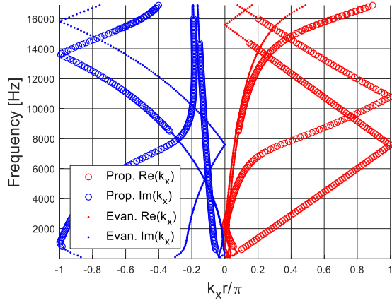
Figure 112: Dispersion curves computed for configuration 4 of Table 4.
