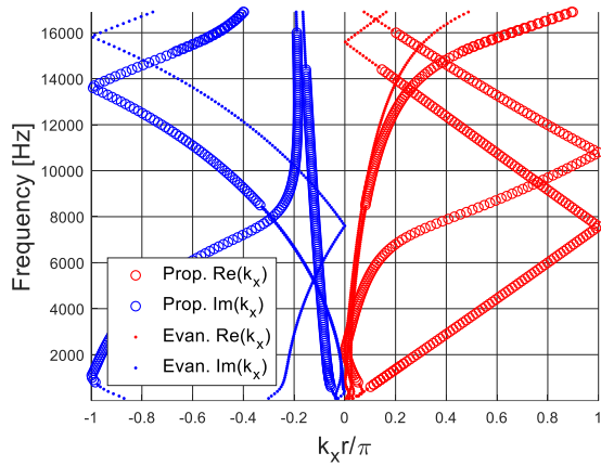
Figure 135: Dispersion curves computed for configuration 27 of Table 4.
