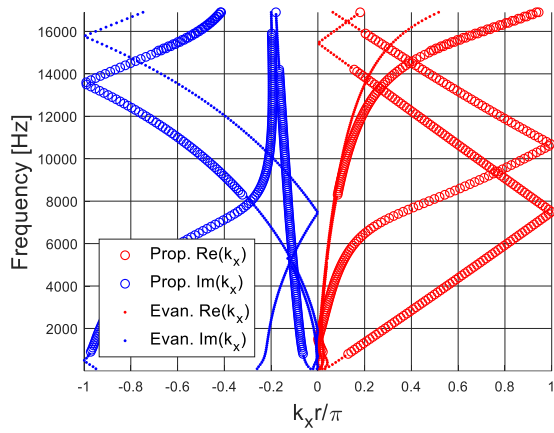
Figure 113: Dispersion curves computed for configuration 5 of Table 4.
