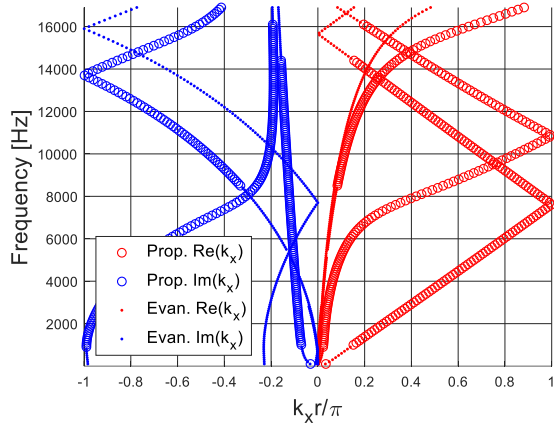
Figure 115: Dispersion curves computed for configuration 7 of Table 4.
