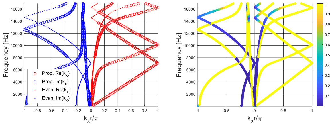
Figure 140: Dispersion curves computed for configuration 32 of Table 4.
