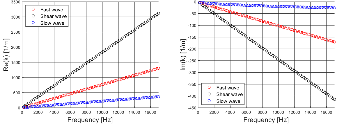
Figure 57: Real (left) and imaginary (right) parts of analytically estimated dispersion curves for a 3D Biot-modeled homogeneous PU 60 foam.
