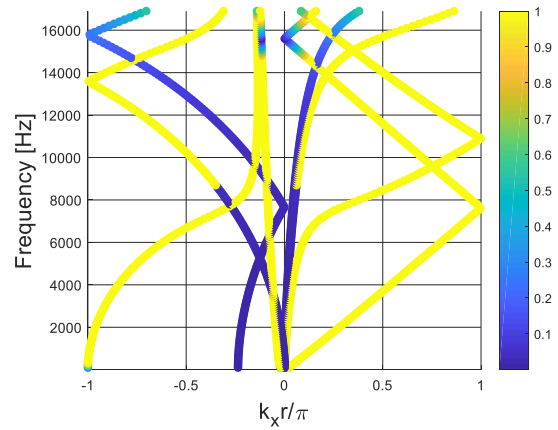
Figure 117: Dispersion curves computed for configuration 9 of Table 4.
