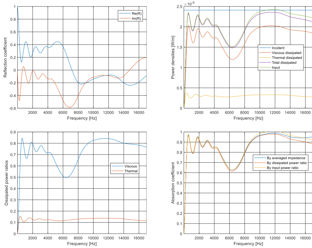
Figure 168: Reflection coefficient, power densities, dissipated power ratios and absorption coefficient computed for a JCA-modeled black PU 2D unit cell with a perfectly rigid inclusion.
