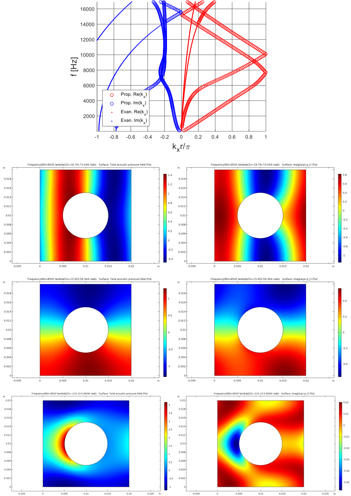
Figure 102: Dispersion curves for a DB-modeled black PU 2D unit cell with a perfectly rigid inclusion; from top to bottom, the 1 st , 2 nd and 3 rd branch eigenvectors are shown in terms of real (on the left) and imaginary (on the right) parts.
