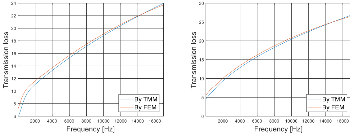
Figure 192: Transmission loss computed for a homogeneous JCA-modeled melamine (on the left) and black PU (on the right) 2D unit cell.
