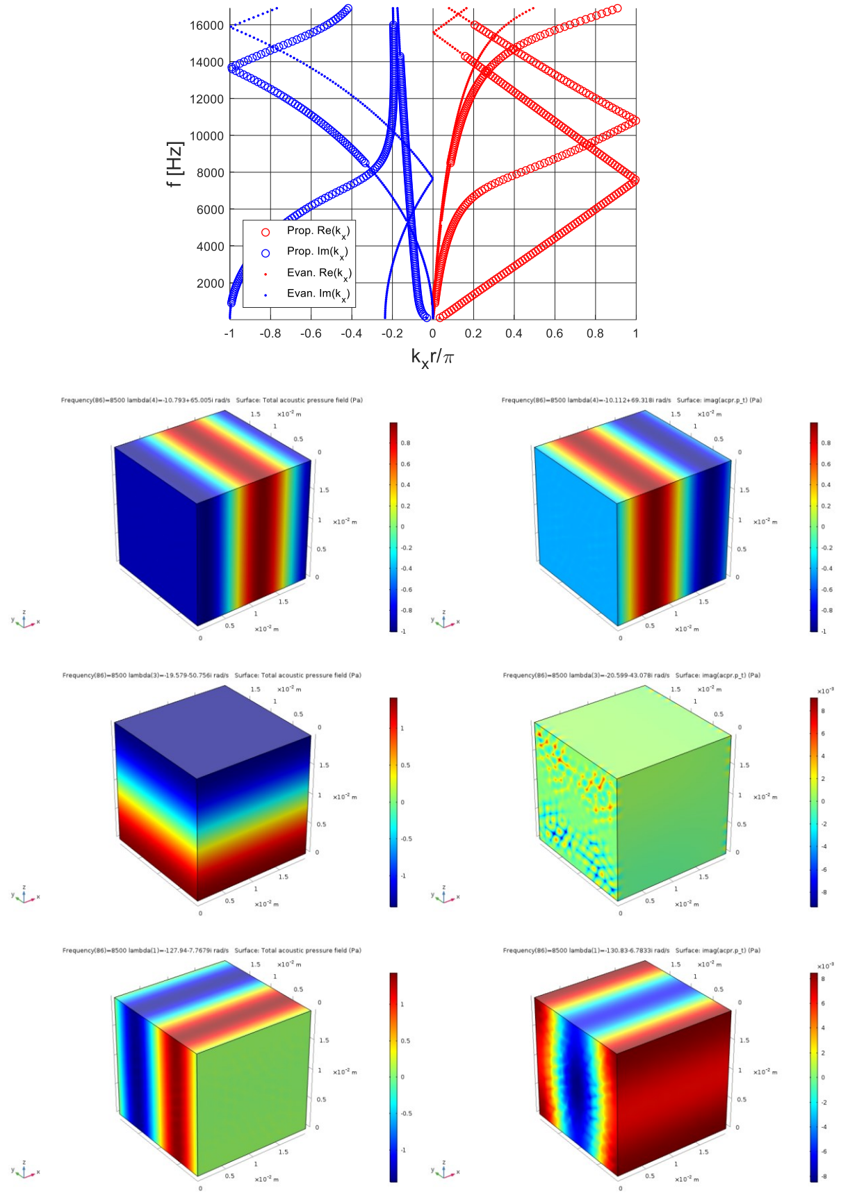
Figure 99: Dispersion curves for a homogeneous JCA-modeled melamine 3D unit cell; from top to bottom, the 1 st , 2 nd and 3 rd branch eigenvectors are shown in terms of real (on the left) and imaginary (on the right) parts.
