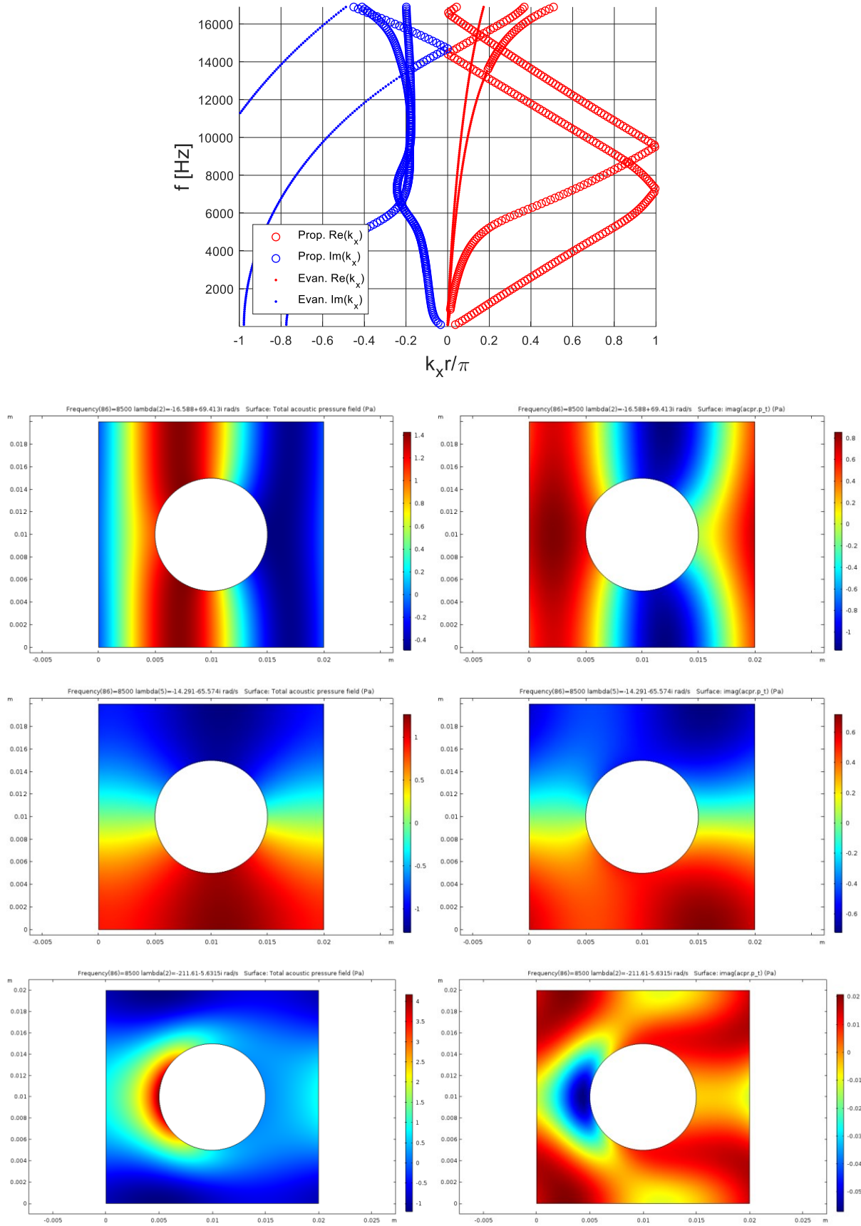
Figure 103: Dispersion curves for a JCA-modeled melamine 2D unit cell with a perfectly rigid inclusion; from top to bottom, the 1 st , 2 nd and 3 rd branch eigenvectors are shown in terms of real (on the left) and imaginary (on the right) parts.
