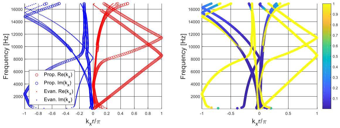
Figure 119: Dispersion curves computed for configuration 11 of Table 4.
