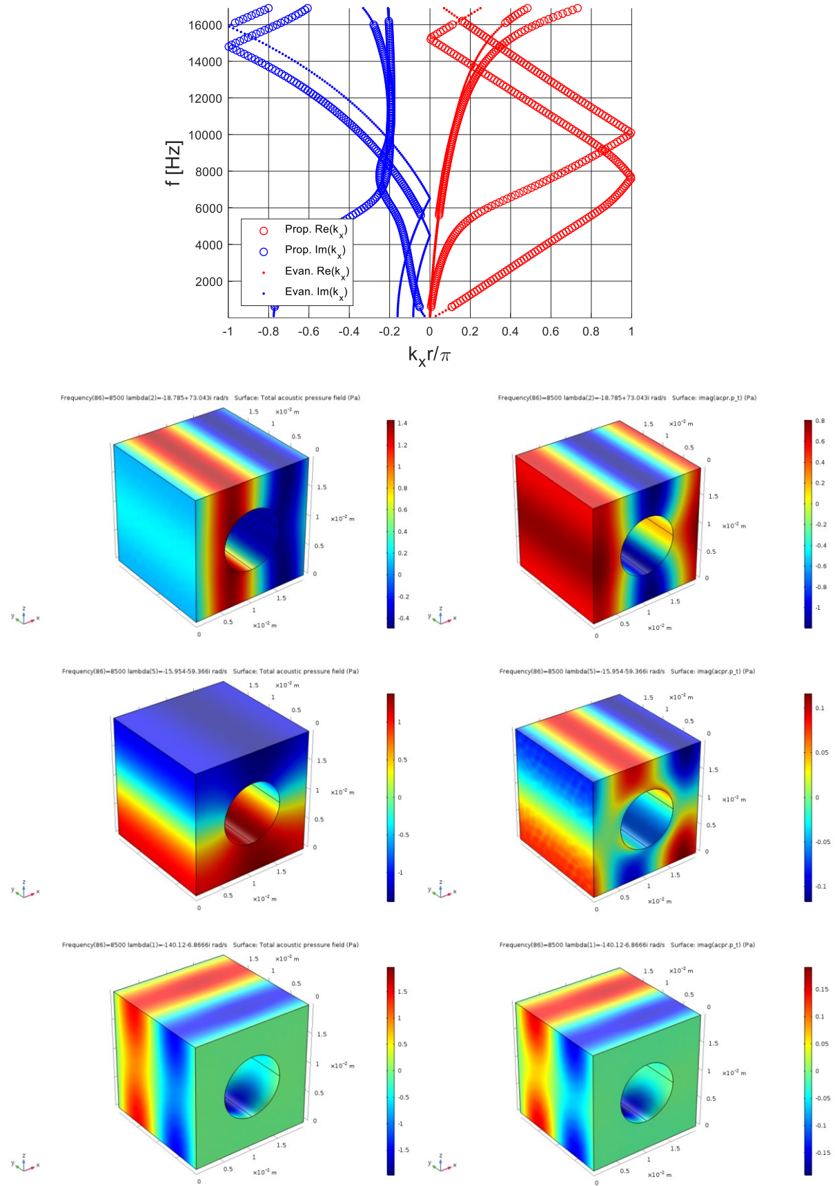
Figure 106: Dispersion curves for a DB-modeled black PU 3D unit cell with a perfectly rigid inclusion; from top to bottom, the 1 st , 2 nd and 3 rd branch eigenvectors are shown in terms of real (on the left) and imaginary (on the right) parts.
