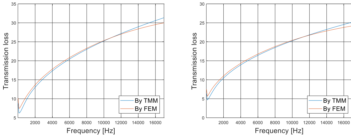
Figure 193: Transmission loss computed for a homogeneous DB-modeled melamine (on the left) and black PU (on the right) 3D unit cell.
