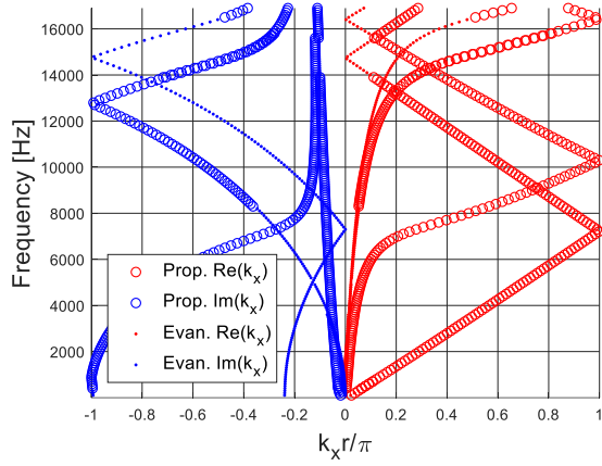
Figure 136: Dispersion curves computed for configuration 28 of Table 4.
