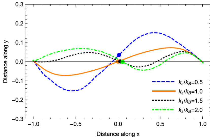
Figure 2.18 – S -shaped trajectories for annihilating \pm 1 defect pairs. Different elastic constant have been used The backflow effects are neglected and the defects are considered aligned with the far c -director field. Reprinted from Tang and Selinger [2020]. Copyright (2020) by The American Physical Society.
