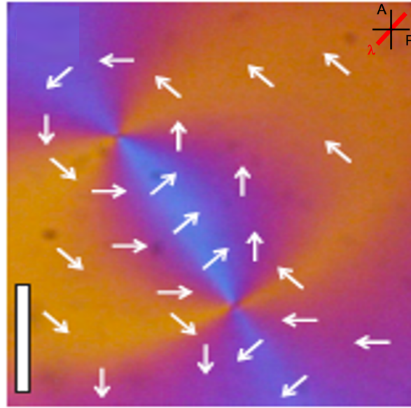
Figure 2.6 – Defect pair on the way to annihilation. White arrows sketch the c -director configuration. The +1 defect (top) and the -1 defect (bottom) about 21 seconds before the annihilation time. The white bar is 50 \mu\text{m} . Experimental data carried out by Peter Salamon. Reprinted from Missaoui et al. [2020] . Copyright (2020) by The American Physical Society.
