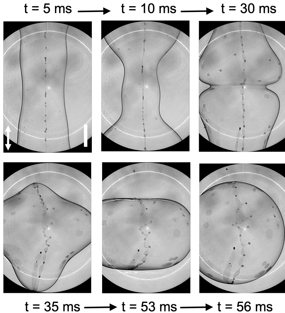
Figure 4.10 – Relaxation of a smectic bubble of equilibrium radius a \approx 2.3 mm, created by the collapse of a catenoid-shaped film. After pinch-off ( t = 0 ms), the bubble has an elongated shape. It will then relax to acquire the stable spherical shape, after about 56 ms. The bubble is excited with oscillating films remaining on the catenoid rings and without loudspeakers. The white bar represents 1 mm. The axis of symmetry of the catenoid is indicated by the white arrow.
