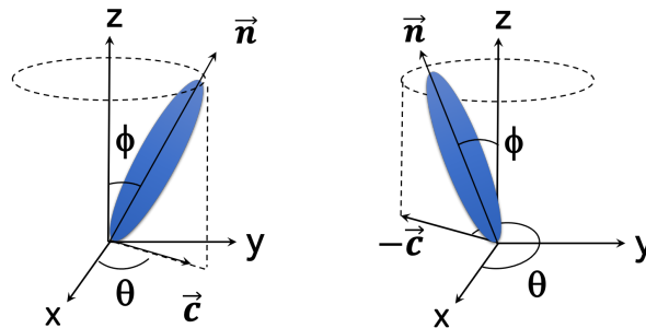
Figure 1.2 – The SmC director. The projection of molecules onto the layer plane ( xy ) allows the construction of the c-director . Unlike the nematic director \vec{n} , \vec{c} is not equivalent to -\vec{c} .
