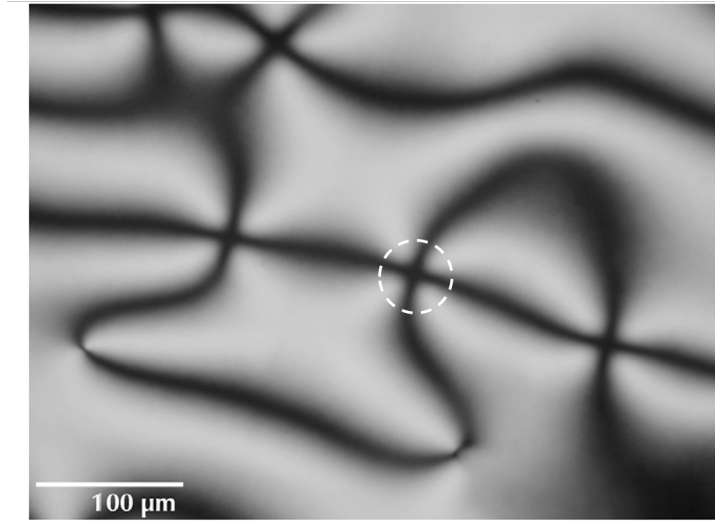
Figure 1.6 – An example of the characteristic schlieren texture of nematic liquid crystals observed by the mean of polarizing microscope between crossed polarizers. The white circle points out one singular point. Reproduced from Publication Lagerwall and Scalia [2012]. Copyright (2012), with permission from Elsevier.
