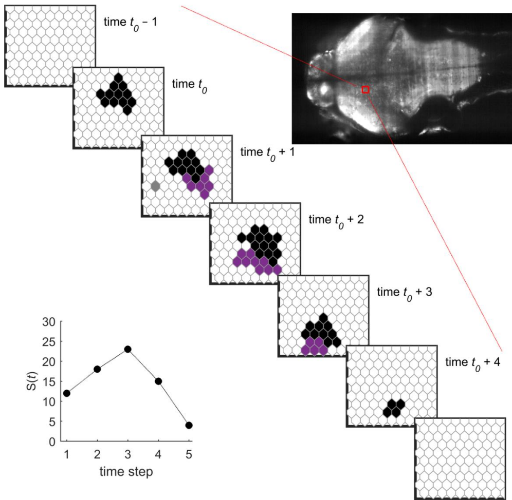
Supplemental figure S3. Avalanche definition. Related to Figure 2. The illustration of an avalanche is shown here in 2D for simplicity but note that the analysis was done in 3D. An avalanche was initiated with the detection of a cluster of active ROIs at time t_0 , the avalanche continued at time t_0+1 with a cluster composed of ROIs that were active at the preceding time t_0 (represented in black) plus ROIs that activated at t_0+1 (represented in purple), and so on, until this condition no longer held. The avalanche terminated at time t_0+4 . The ROI represented in gray that was activated at time t_0+1 did not participate in an avalanche, since it did not belong to any activity cluster. For this schematic example the size and duration of the avalanche were equal to S = 72 (the cumulative sum of the number of activated ROIs during the avalanche) and T = 5 \times dt (number of frames multiply by the temporal resolution, dt , of the data), respectively. The time-course of the avalanche size, S(t) , is shown in the left bottom panel.
