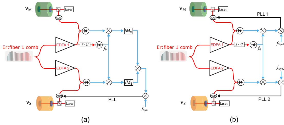
Figure 4.3: In (a) multi-branch transfer scheme. In (b) multi-branch assessment without a transfer beatnote.
