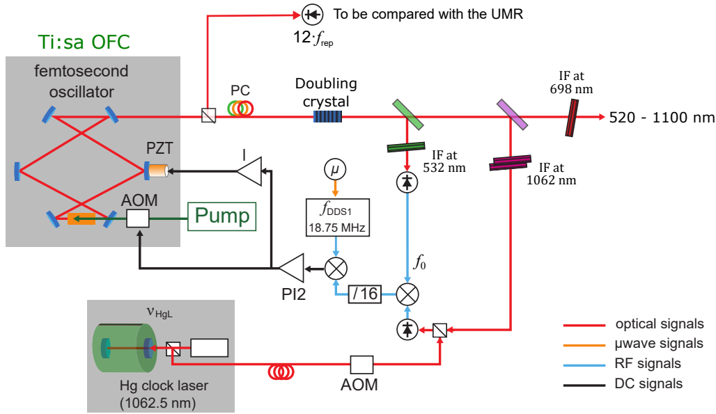
Figure 2.2: Phase lock of the Ti:sapphire comb to an ultrastable cw laser at 1062.5 nm and unique optical output. AOM: acousto-optic modulator, IF: interferometric filter (0.1 – 1 nm), PC: photonic crystal, and PZT: piezo-electric ceramic.
