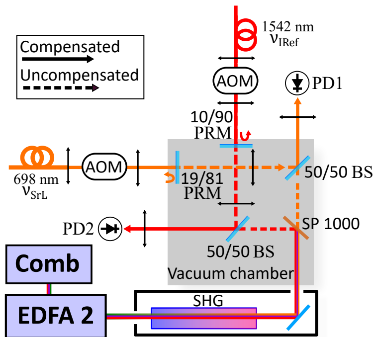
Figure 4.10: Optical setup for the \nu_{IRref} at 1542 nm (master laser) spectral purity transfer to the \nu_{SrL} at 698 nm (slave laser). The comb's light is split up in two with a short-pass (SP) dichroic mirror, separating the infrared and the visible light. Reflection for fiber noise compensation in partial retro-reflector mirrors (PRMs), combination with the lasers' lights for beatnote generation in beam splitters (BSs) and photodetection (PD1 and PD2) takes place individually.
