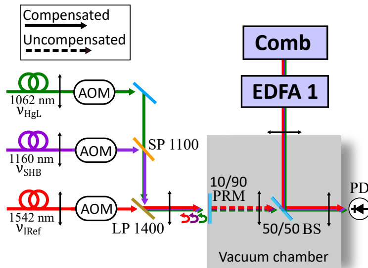
Figure 4.6: Optical setup for the \nu_{\text{IRef}} at 1542 nm (master laser) spectral purity transfer to \nu_{\text{HgL}} at 1062 nm (slave laser), with the possibility of being applied to \nu_{\text{SHB}} at 1160 nm. The three lasers’ paths are overlapped using short-pass (SP) and long-pass (LP) dichroic mirrors so they can be reflected back in the same 10/90 (R/T) partial retro-reflector mirror (PRM) for fiber noise compensation. Subsequently they are all combined on a 50/50 beam splitter (BS) with the comb’s light for beatnote detection by the same photodetector (PD).
