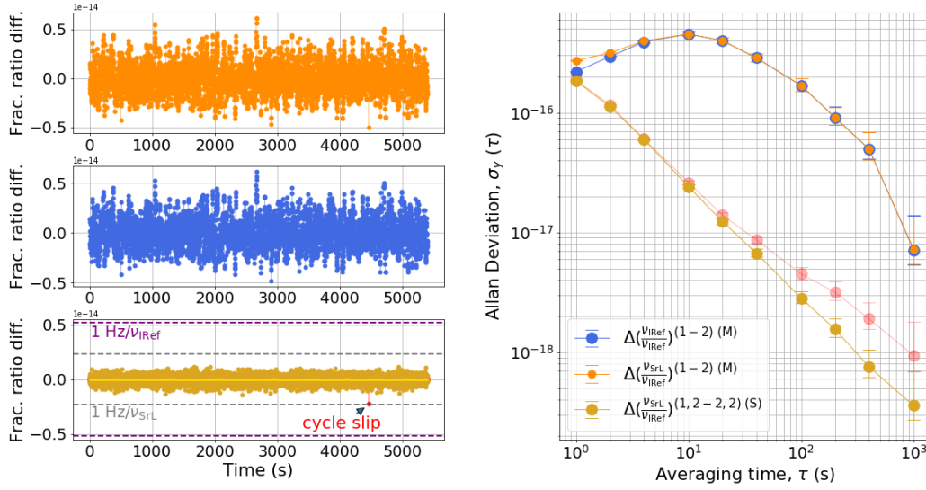
Figure 3.13: Multi-branch optical comparison (M: i \neq j ) between the two fiber combs for \nu_{\text{SrL}}^{(z,i)} / \nu_{\text{IRef}}^{(z,j)} (orange) and \nu_{\text{IRef}}^{(z,i)} / \nu_{\text{IRef}}^{(z,j)} (blue). Bottom plot shows a direct detection of cycle slips on a single-branch optical comparison (S: i = j ) for \nu_{\text{SrL}}^{(z,i)} / \nu_{\text{IRef}}^{(z,j)} and its impact on the fractional stability (red curve).
