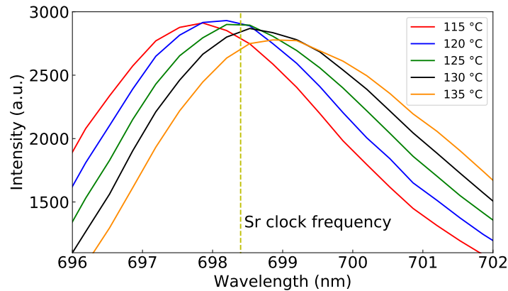
Figure 4.8: PPLN doubling crystal spectrum versus temperature for the EDFA 2 of Er: fiber 2. The yellow dash line shows an optimal temperature of 125 °C for the Sr clock wavelength. The optical resolution of the spectrometer is 1.5 nm approximately.
