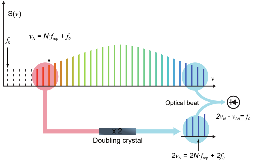
Figure 1.3: f-2f interferometer used for the f_0 detection.
