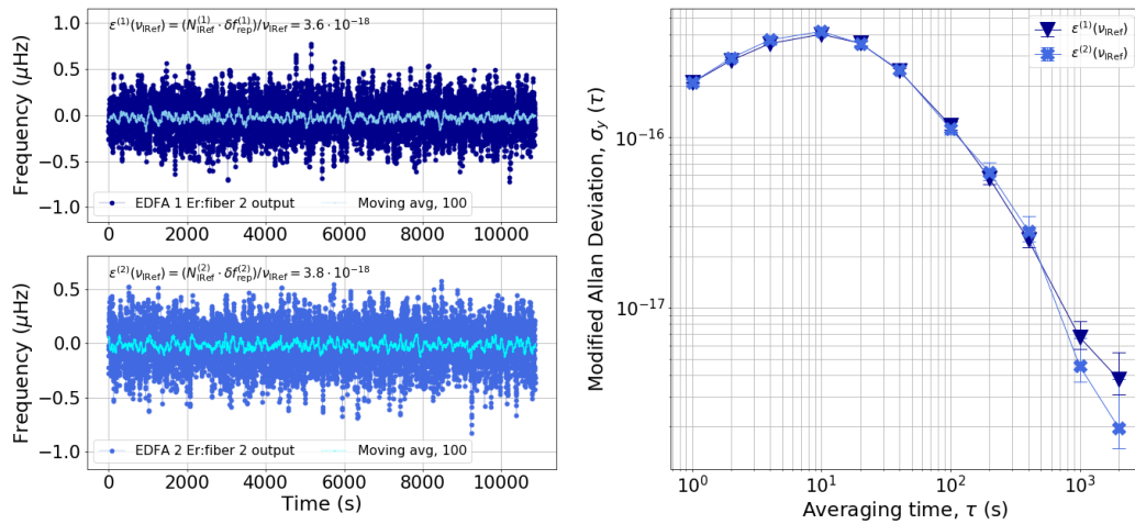
Figure 2.13: Averaged fractional values and fractional stabilities after the Er:fiber 2 comb optical amplifiers EDFA 1 and EDFA 2. N_{IRef}^{(1)} and N_{IRef}^{(2)} are equal to 777 289 and 777 290, respectively. Measurements in Lambda mode.
