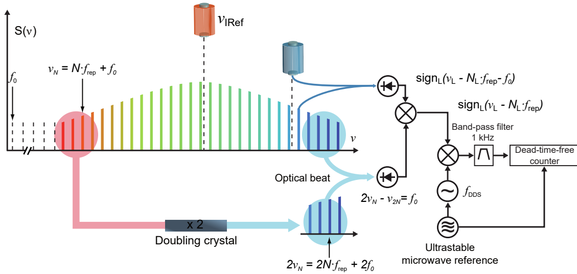
Figure 2.9: Optical beatnote detection and real-time f_0 demodulation. Red ultrastable cavity represents the USL, v_{\text{LRef}} , to which the OFC is locked. Blue cavity is the USL to be measured once the beatnote has been photodetected, demodulated and filtered in the RF domain.
