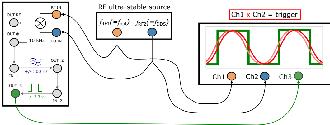
Figure 2.10: Setup used to measure the phase response of the 1 kHz filter. After 10 kHz down-conversion (“OUT \phi 1”), 1 kHz band-pass filter (“OUT 2”) and square wave conversion (“OUT 3”), the signal is sent to the scope (green). Next, it is triggered with a simulated demodulated signal f_{\text{dem,osc}} which results from multiplying internally \text{Ch1} \times \text{Ch2} in the scope (red).
